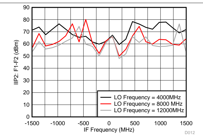
12. IIP2: F1-F2 Across LO Frequency for External LO Mode
