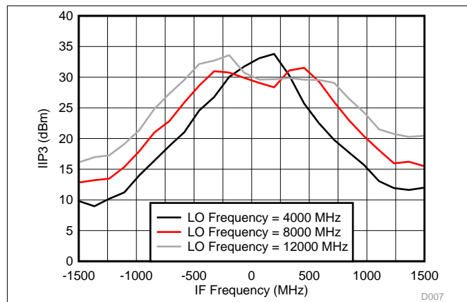
9. IIP3 Across IF Frequency for Internal LO Mode
