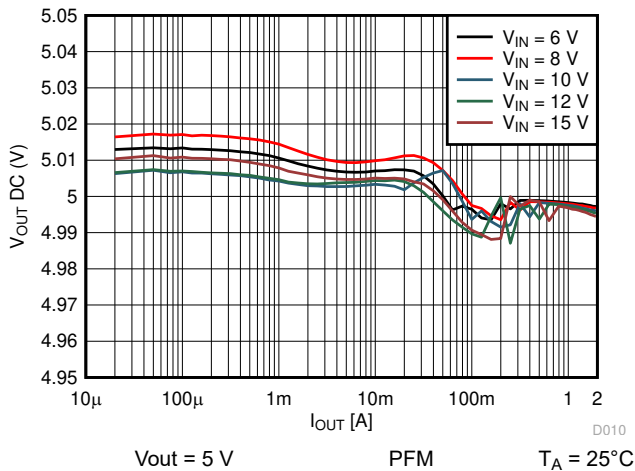
10-28. Output Voltage vs Output Current
