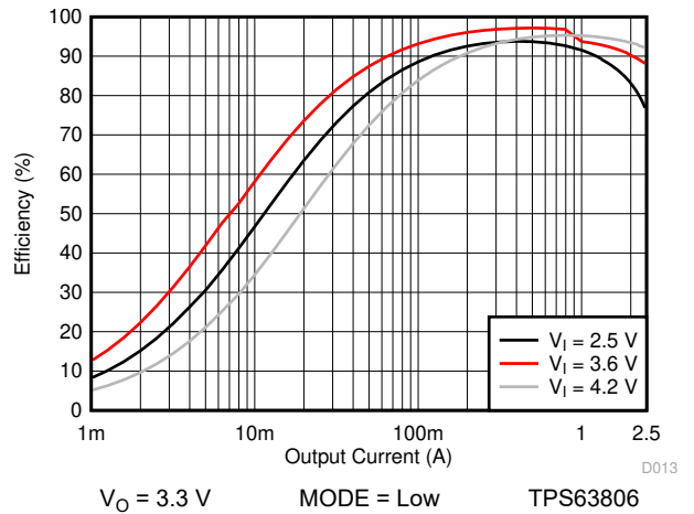
10-14. Efficiency versus Output Current (PWM Only)
