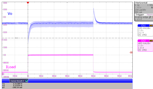
10-35. Load Transient, PFM/PWM Buck Operation
