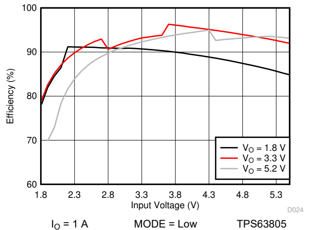
10-12. Efficiency versus Input Voltage (PWM Only)
