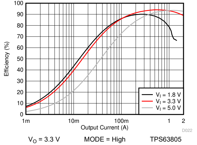
10-10. Efficiency versus Input Voltage (PWM Only)
