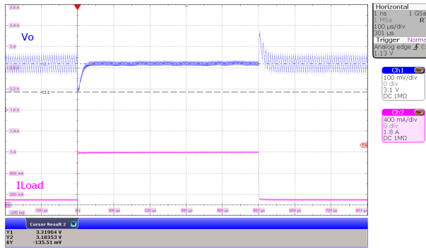
10-33. Load Transient, PFM/PWM Boost Operation
