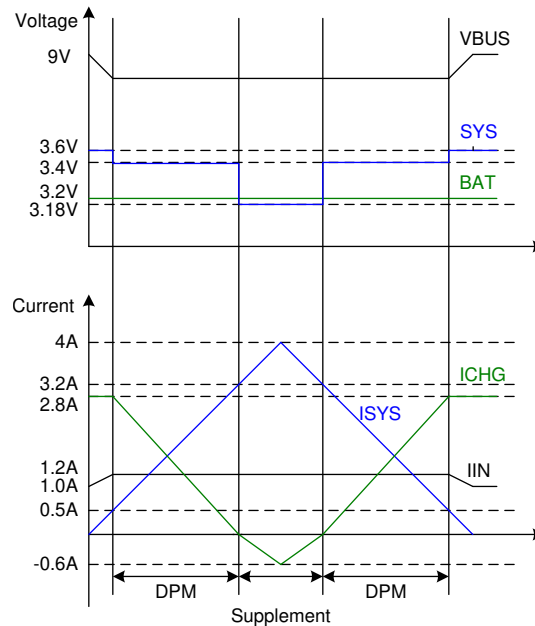
9-8. DPM Response
