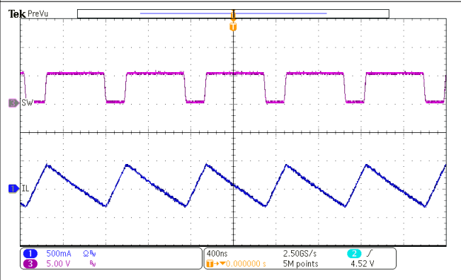
10-11. OTG Switching
