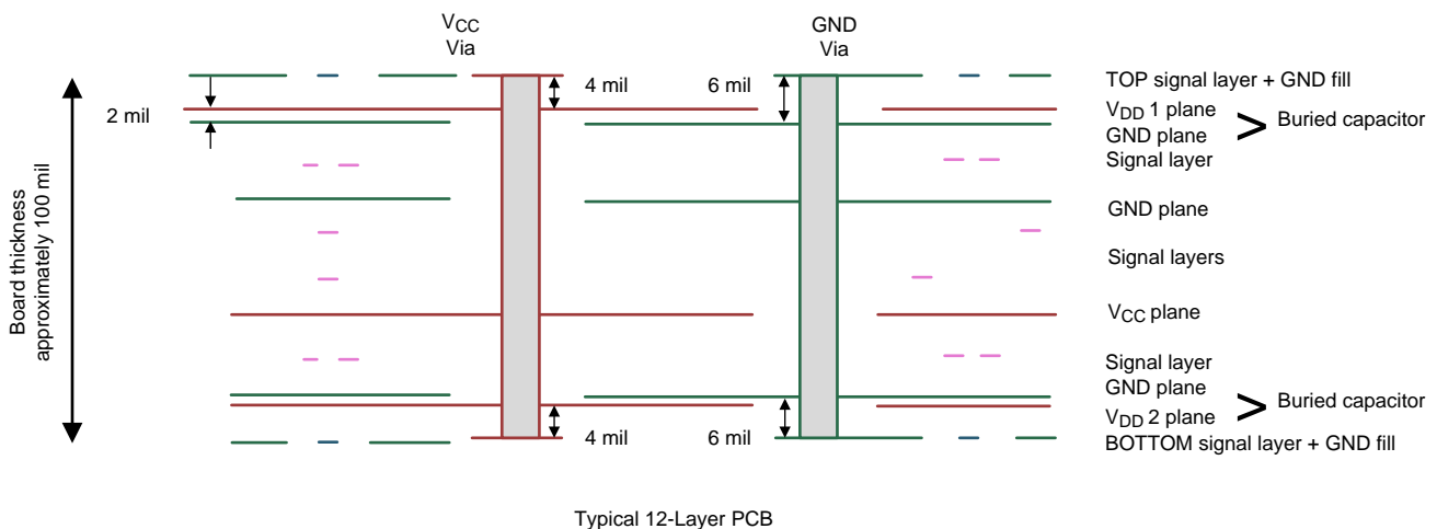
☒ 20. Low-Inductance, High-Capacitance Power Connection
