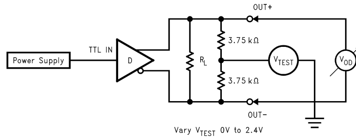
Fig 8. Differential Driver Full Load DC Test Circuit
