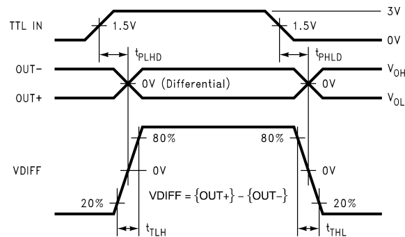
Fig 10. Differential Driver Propagation Delay and Transition Time Waveforms
