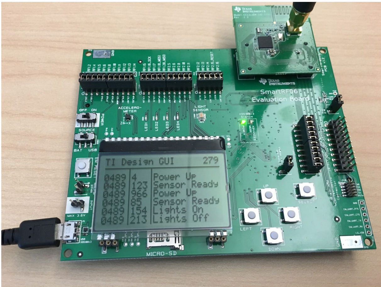
Figure 12. Building Automation Sub-1GHz Sniffer GUI
