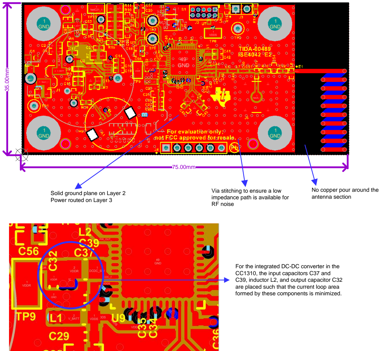
図 35. Low-Power PIR Motion Detector Reference Design Layout Guidelines
