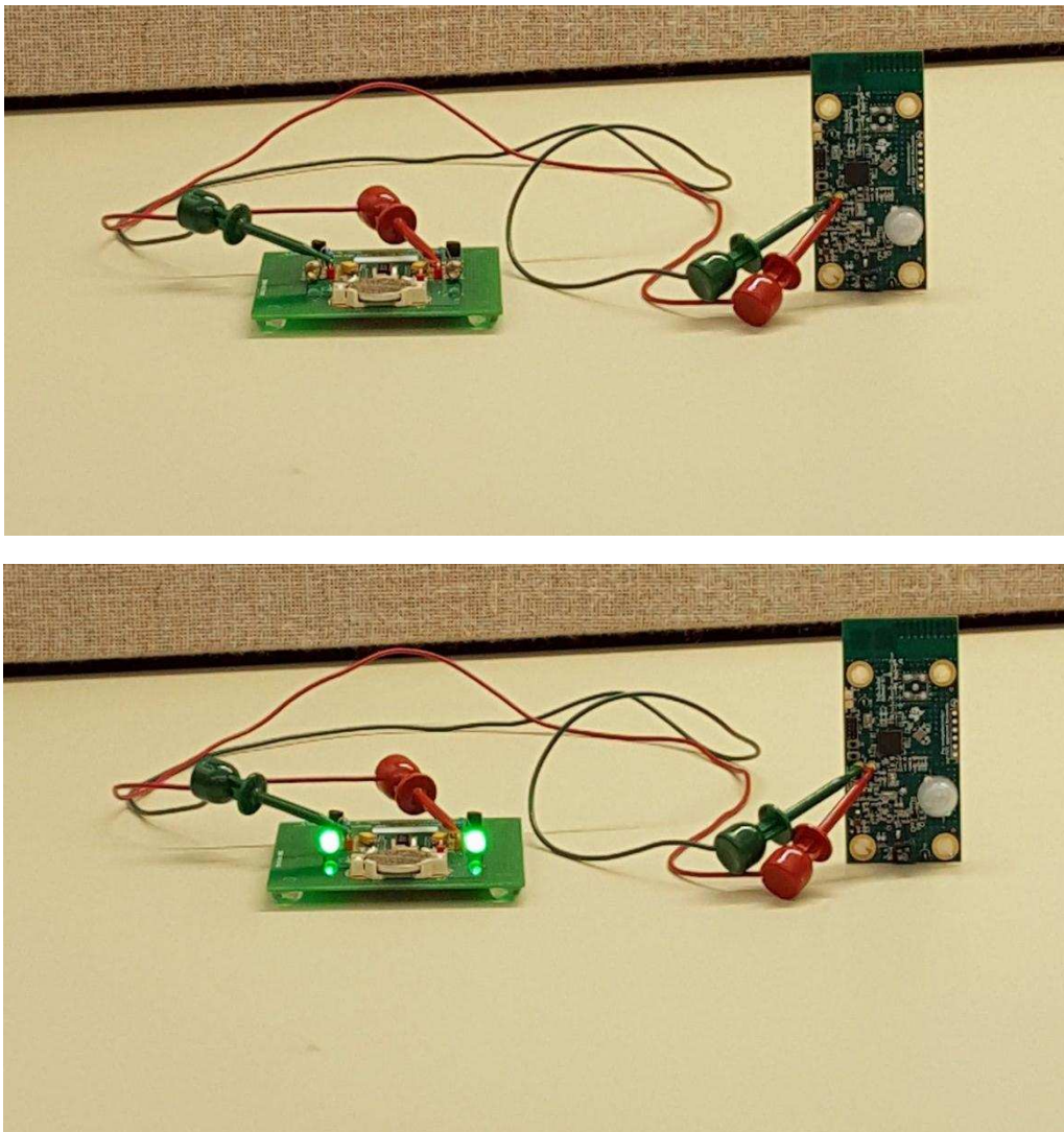
図 20. Motion Sensitivity Test Setup (Top: No Motion; Bottom: Motion Detected)
