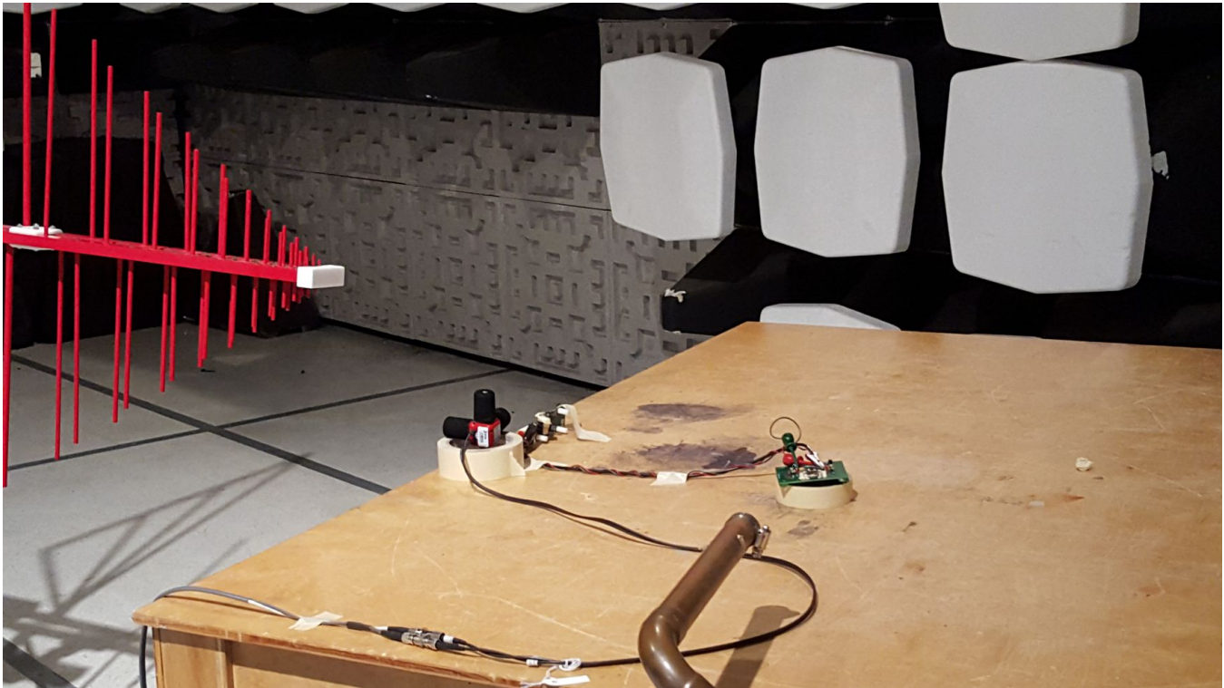
21. RF Immunity Test Setup
