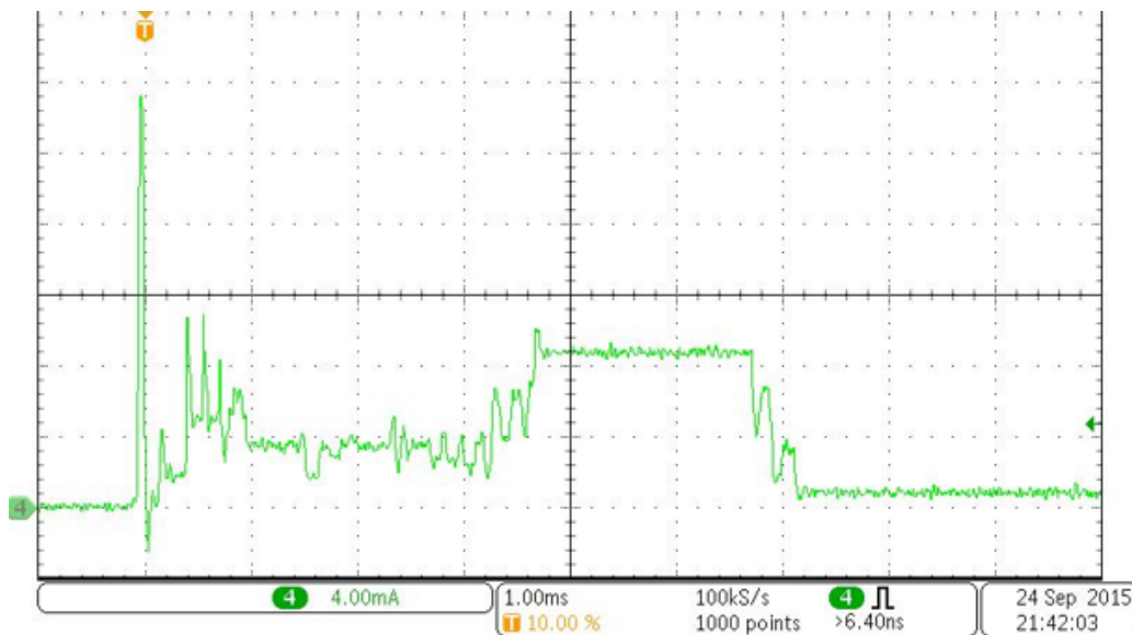
図 22. Radio Transmission Event Supply Current (Zoomed in)
