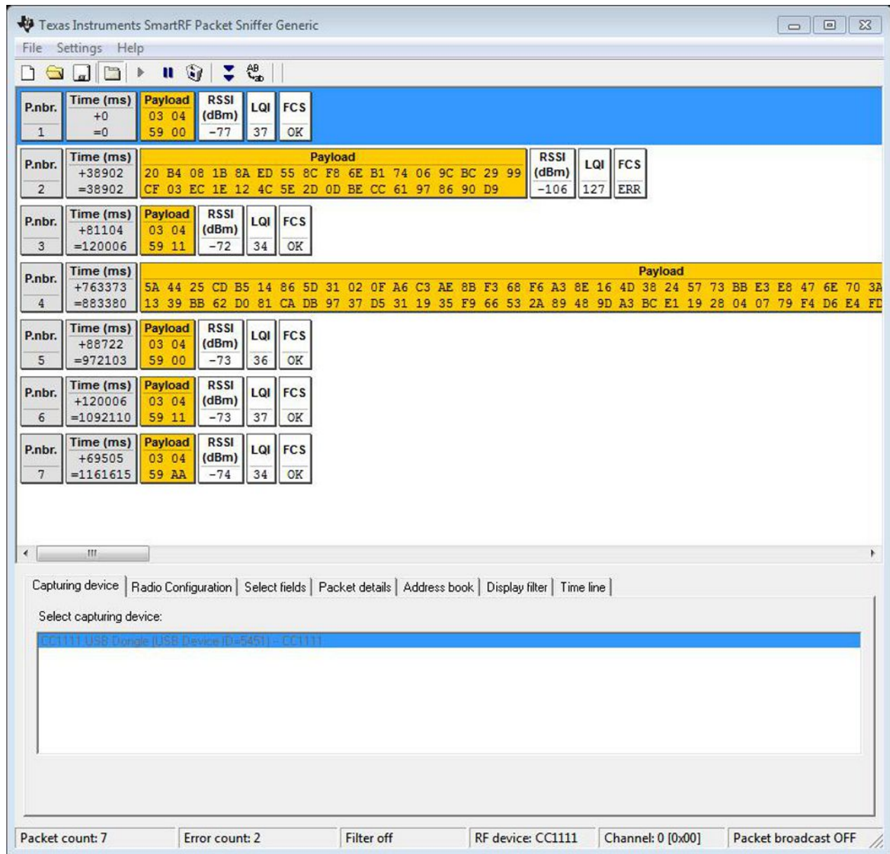
図 15. Packet Sniffer Software, Filterless Recording
