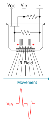
図 4. PIR Motion Sensor Illustration
