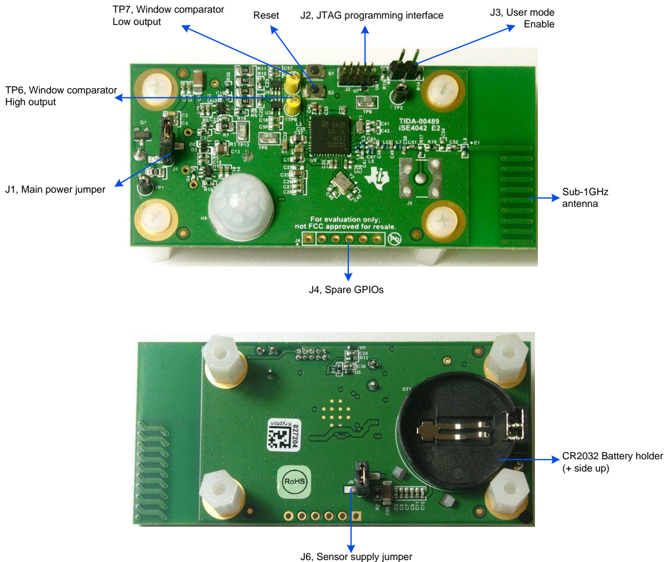
Figure 10. Low-Power Wireless PIR Motion Detector Reference Design Hardware Description
