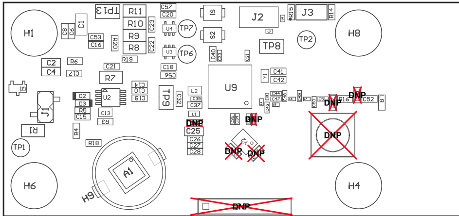
図 37. Top Assembly Drawing
