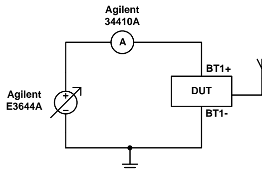
17. Test Circuit Used for Measuring Supply Current
