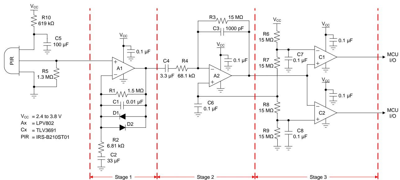
Fig 5. PIR Motion Sensor Analog Signal Path Schematic
