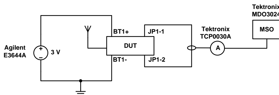
18. Test Circuit Used for Measuring Supply Current During Radio Transmission Intervals
