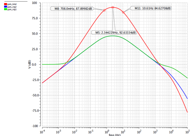
Fig 7. Amplified Filter Simulation Results (Nonideal)
