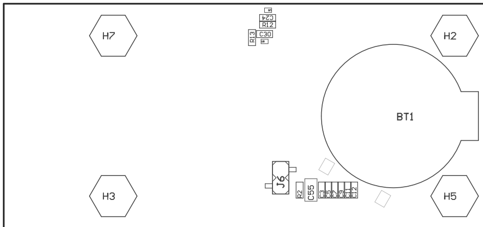
図 38. Bottom Assembly Drawing
