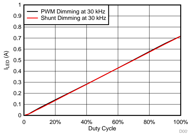
図 27. I_{LED} (A) versus Duty Cycle (%) for PWM or Shunt Dimming at 30 kHz for Red LED String
