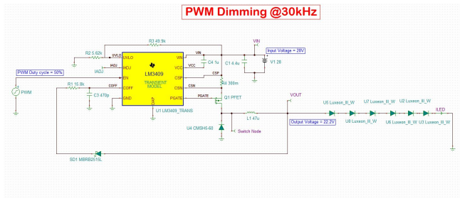
55 . Simulation Circuit for PWM Dimming With LM3409
