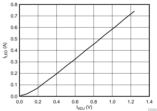
図 26. I_{LED} (A) versus I_{ADJ} (V) for White LED String
