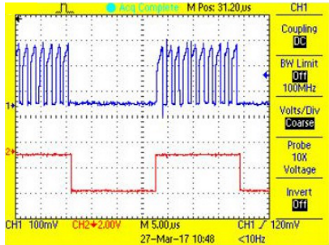
48. P-FET Current During On-Time and Shunt PWM Waveform for Red LED String at 50% Duty Cycle
