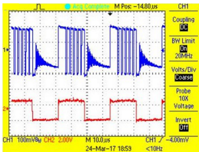
41. Switch Node and PWM Waveform for Green LED String at 50% Duty Cycle
