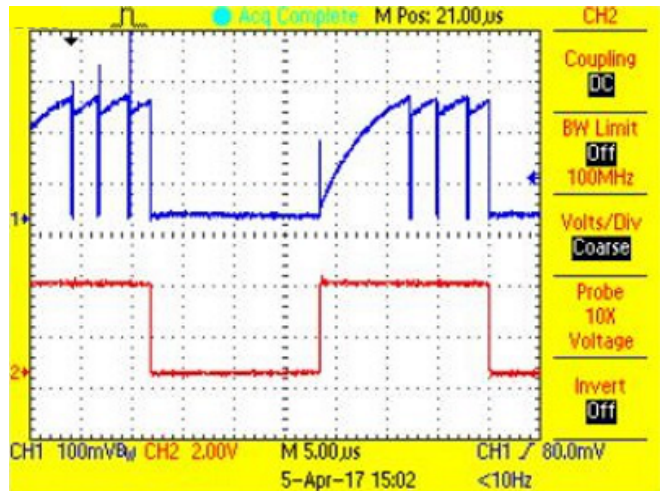
図 46. P-FET Current During On-Time and PWM Waveform for White LED String at 50% Duty Cycle
