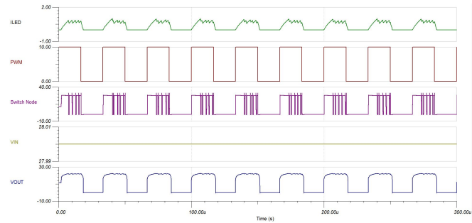
56 . Simulation Results for PWM Dimming at 30 kHz
