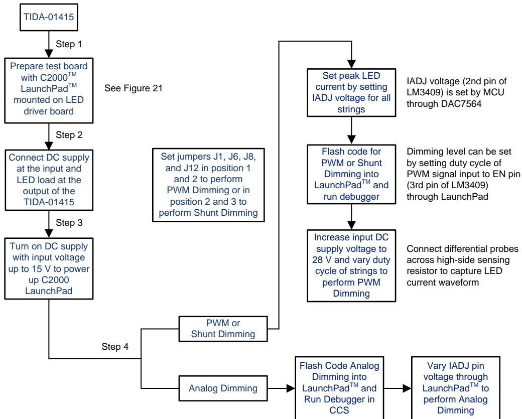
Figure 22. Test Flow to Perform Analog Dimming and PWM or Shunt Dimming Through TIDA-01415
