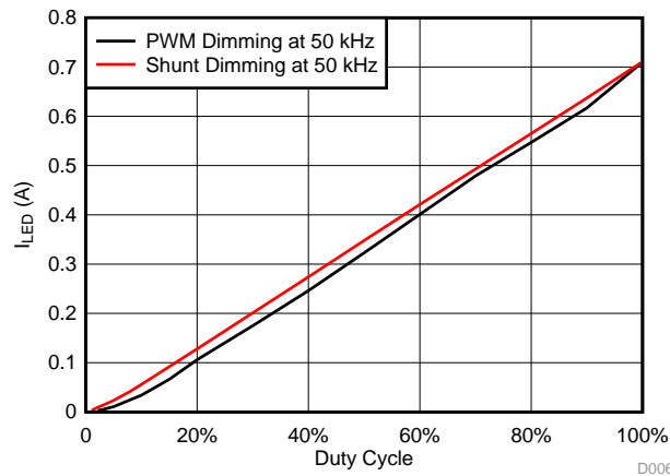
図 32. I LED (A) versus Duty Cycle (%) for PWM or Shunt Dimming at 50 kHz for Green LED String
