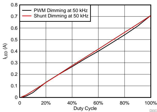
図 33. I LED (A) versus Duty Cycle (%) for PWM or Shunt Dimming at 50 kHz for Blue LED String
