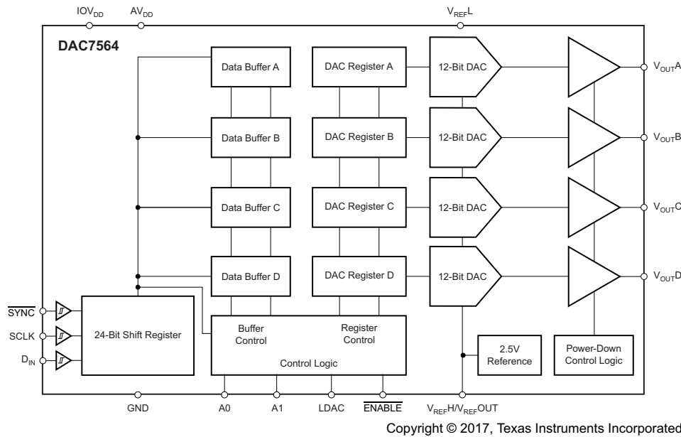
図 6. Functional Block Diagram of DAC7564
