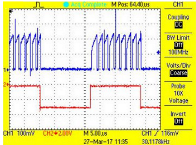
図 52. P-FET Current During On-Time and Shunt PWM Waveform for Blue LED String at 50% Duty Cycle
