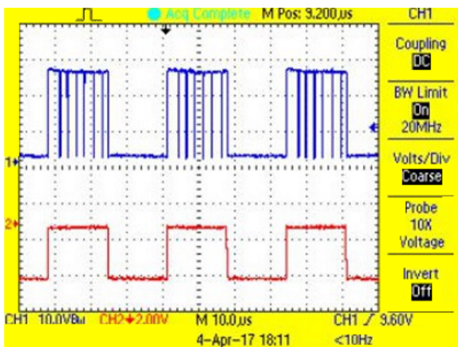
図 53. Switch Node and Shunt PWM Waveform for White LED String at 50% Duty Cycle
