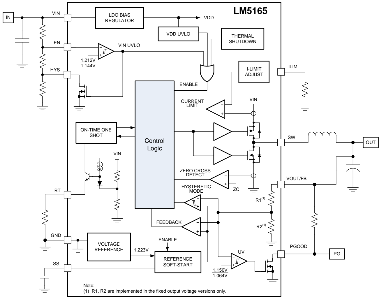
図 10. Functional Block Diagram of LM5165
