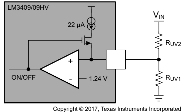
Figure 11. UVLO Circuit of LM3409
