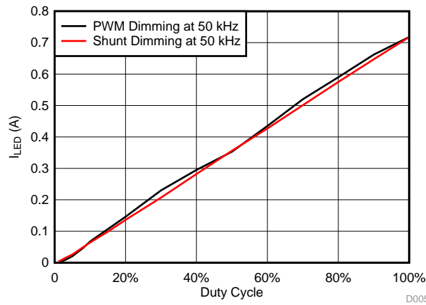
図 31. I_{LED} (A) versus Duty Cycle (%) for PWM or Shunt Dimming at 50 kHz for Red LED String
