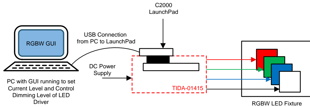
Figure 20. Hardware Interconnections of TIDA-01415
