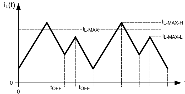
Figure 13. Inductor Current i_L(t) Showing I_{L-MAX} Offset
