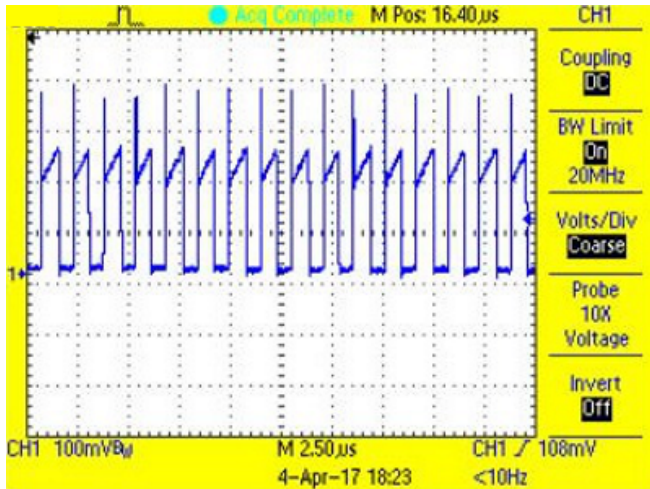
図 35. P-FET Current During On-Time at I_{ADJ} = 1.24\text{ V} for Red String
