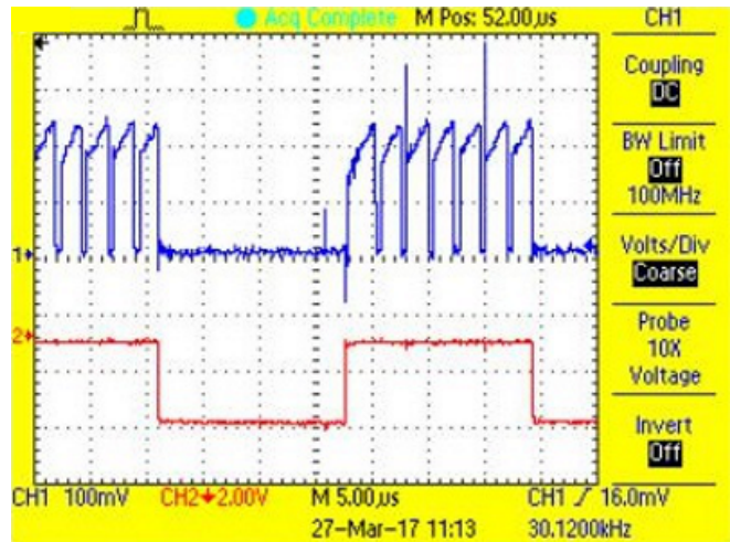
50. P-FET Current During On-Time and Shunt PWM Waveform for Green LED String at 50% Duty Cycle
