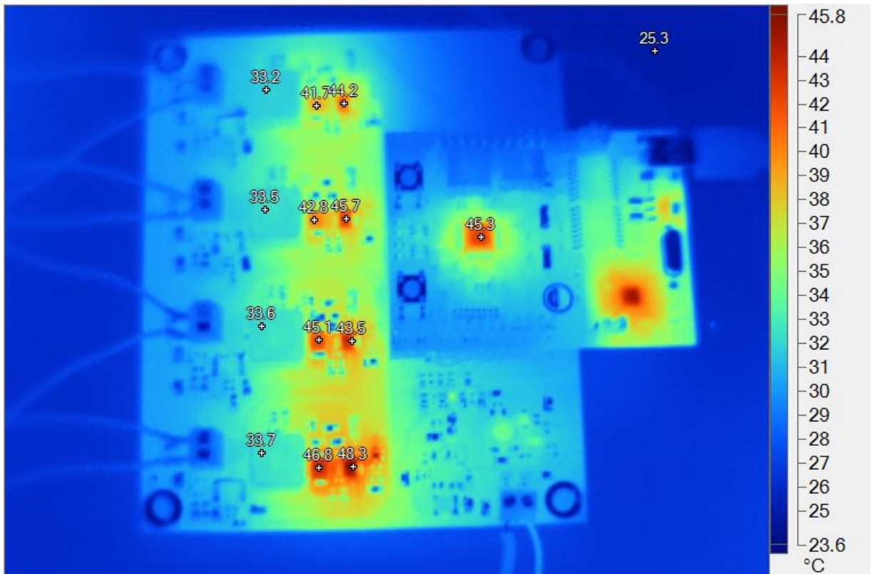
図 61. Thermal Image of Top Side of TIDA-01415 Board for Shunt Dimming at 2.9-A Total LED Current (100% Duty Cycle for All Strings)
