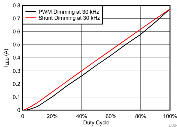
図 30. I LED (A) versus Duty Cycle (%) for PWM or Shunt Dimming at 30 kHz for White LED String
