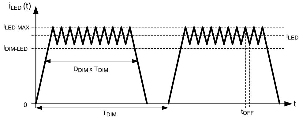
図 15. LED Current i_{LED}(t) During EN Pin PWM Dimming
