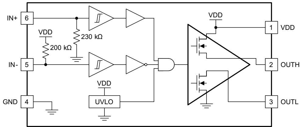
図 7. Functional Block Diagram of UCC27511
