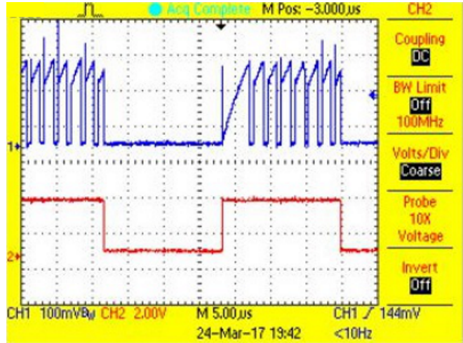
図 44. P-FET Current During On-Time and PWM Waveform for Blue LED String at 50% Duty Cycle
