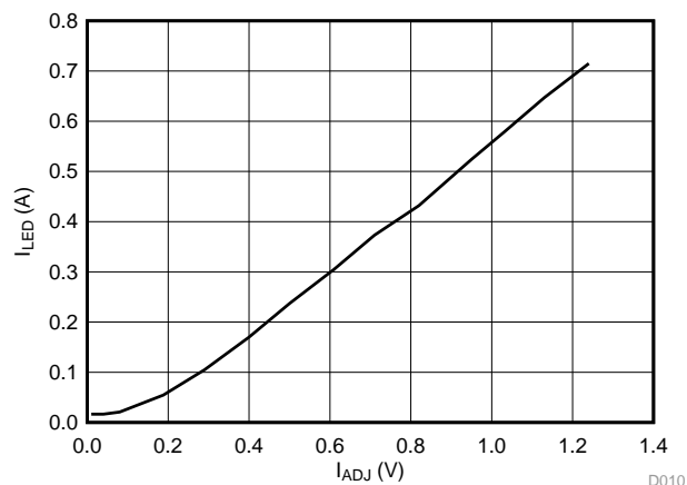
図 23. I_{LED} (A) versus I_{ADJ} (V) for Red LED String
