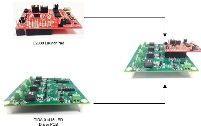
Figure 21. C2000 LaunchPad Mounted on TIDA-01415 LED Driver Board
