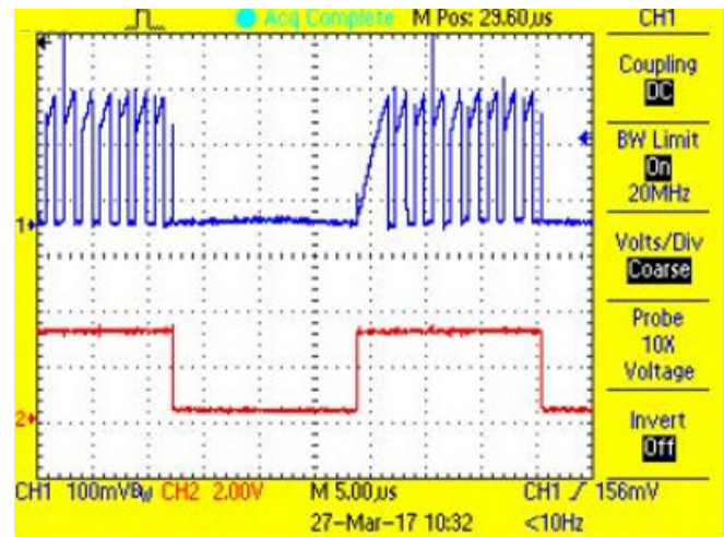
40. P-FET Current During On-Time and PWM Waveform for Red LED String at 50% Duty Cycle
