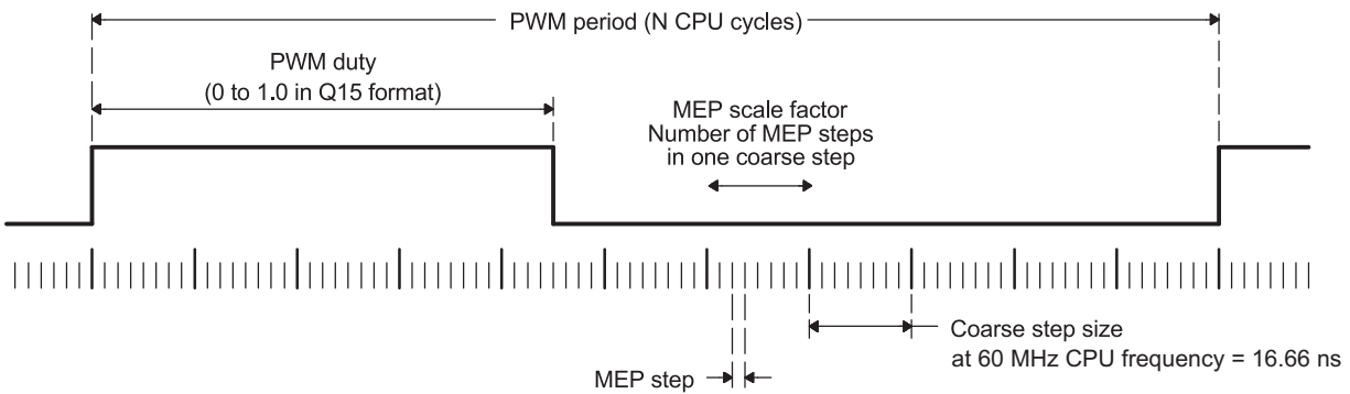
図 16. Conventional PWM and HRPWM Timing Diagram
