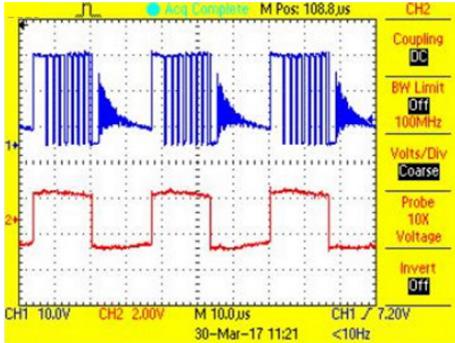
図 43. Switch Node and PWM Waveform for Blue LED String at 50% Duty Cycle
