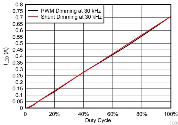
図 29. I LED (A) versus Duty Cycle (%) for PWM or Shunt Dimming at 30 kHz for Blue LED String
