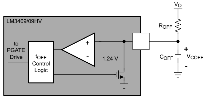
Figure 12. Off-Time Control Circuit
