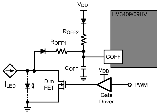
Figure 14. External Parallel FET Dimming Circuit
