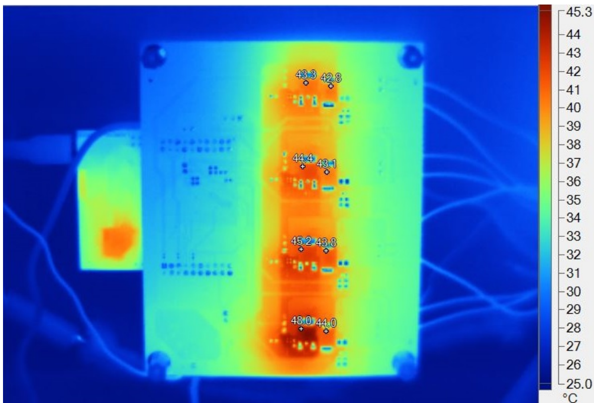
図 60. Thermal Image of Bottom Side of TIDA-01415 Board for PWM Dimming at 2.9-A Total LED Current (100% Duty Cycle for All Strings)
