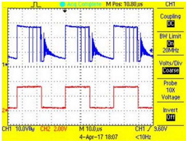
図 45. Switch Node and PWM Waveform for White LED String at 50% Duty Cycle
