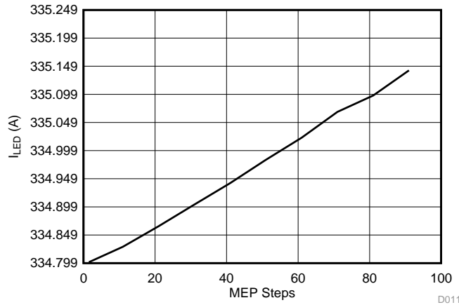
図 17. I LED versus MEP Steps for Green LED String at 30-kHz PWM Dimming Frequency
