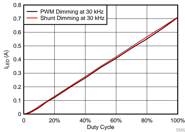
図 28. I LED (A) versus Duty Cycle (%) for PWM or Shunt Dimming at 30 kHz for Green LED String
