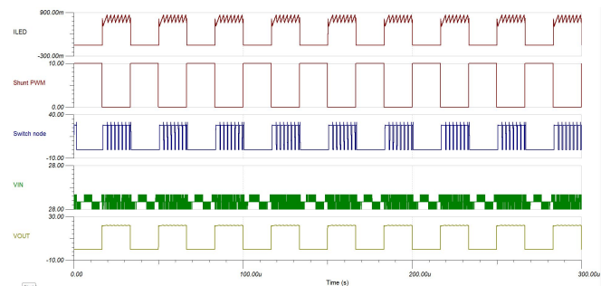
58 . Simulation Results for Shunt Dimming at 30 kHz
