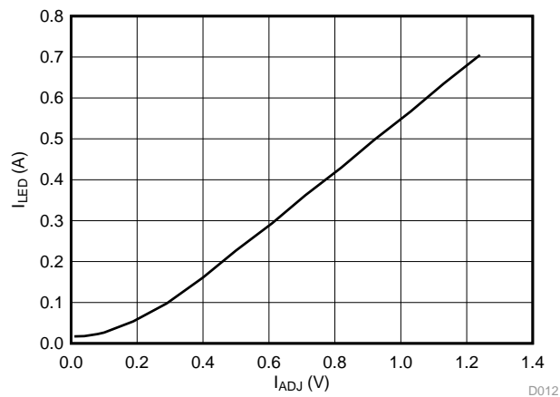
図 25. I_{LED} (A) versus I_{ADJ} (V) for Blue LED String
