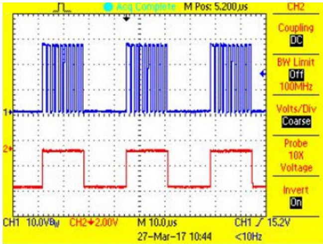
47. Switch Node and Shunt PWM Waveform for Red LED String at 50% Duty Cycle
