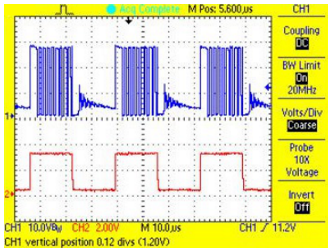
39. Switch Node and PWM Waveform for Red LED String at 50% Duty Cycle
