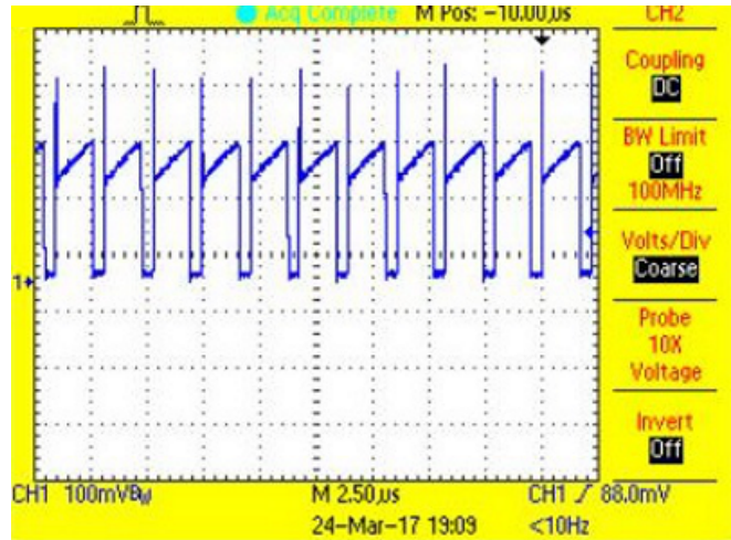
図 36. P-FET Current During On-Time at I_{ADJ} = 1.24\text{ V} for Green String
