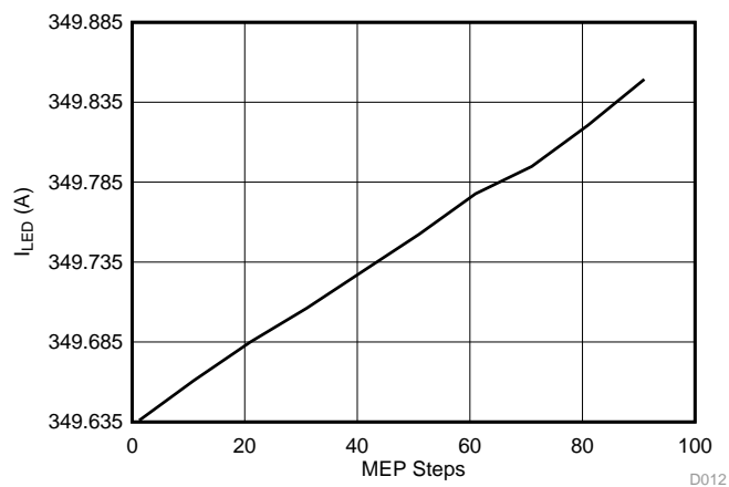
図 18. I_{LED} versus MEP Steps for Green LED String at 30-kHz Shunt Dimming Frequency
