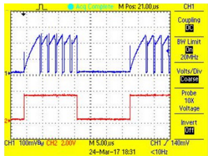
42. P-FET Current During On-Time and PWM Waveform for Green LED String at 50% Duty Cycle
