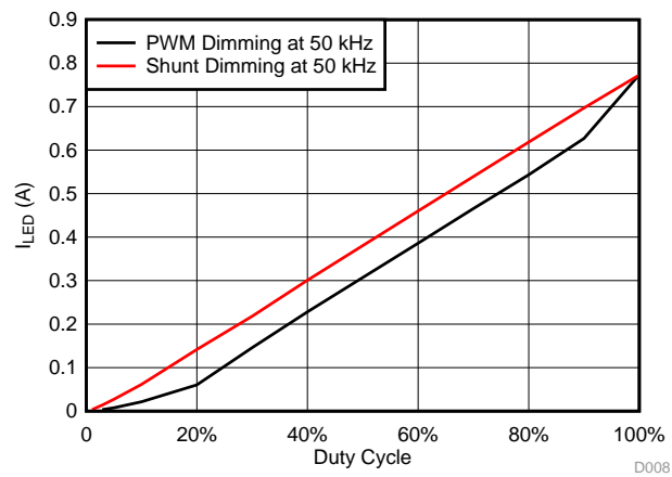
図 34. I_{LED} (A) versus Duty Cycle (%) for PWM or Shunt Dimming at 50 kHz for White LED String
