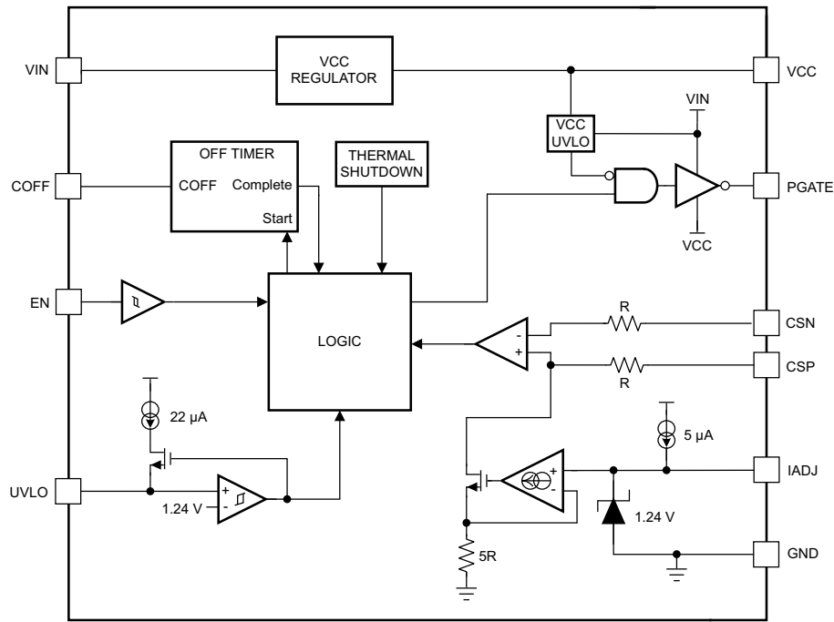
図 5. Functional Block Diagram of LM3409
