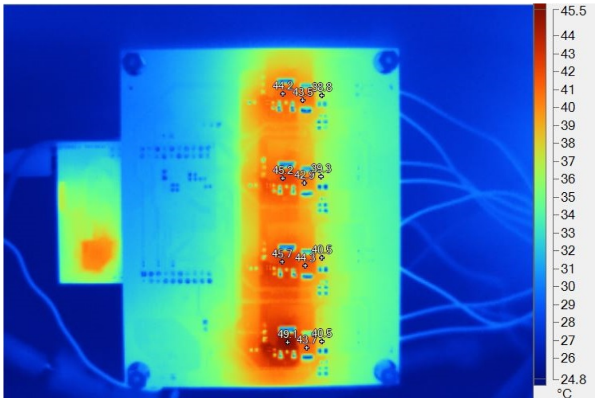
図 62. Thermal Image of Bottom Side of TIDA-01415 Board for Shunt Dimming at 2.9-A Total LED Current (100% Duty Cycle for All Strings)
