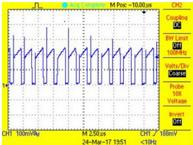
図 37. P-FET Current During On-Time at I_{ADJ} = 1.24\text{ V} for Blue String
