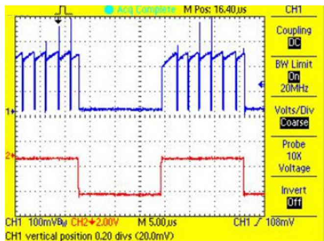
図 54. P-FET Current During On-Time and Shunt PWM Waveform for White LED String at 50% Duty Cycle
