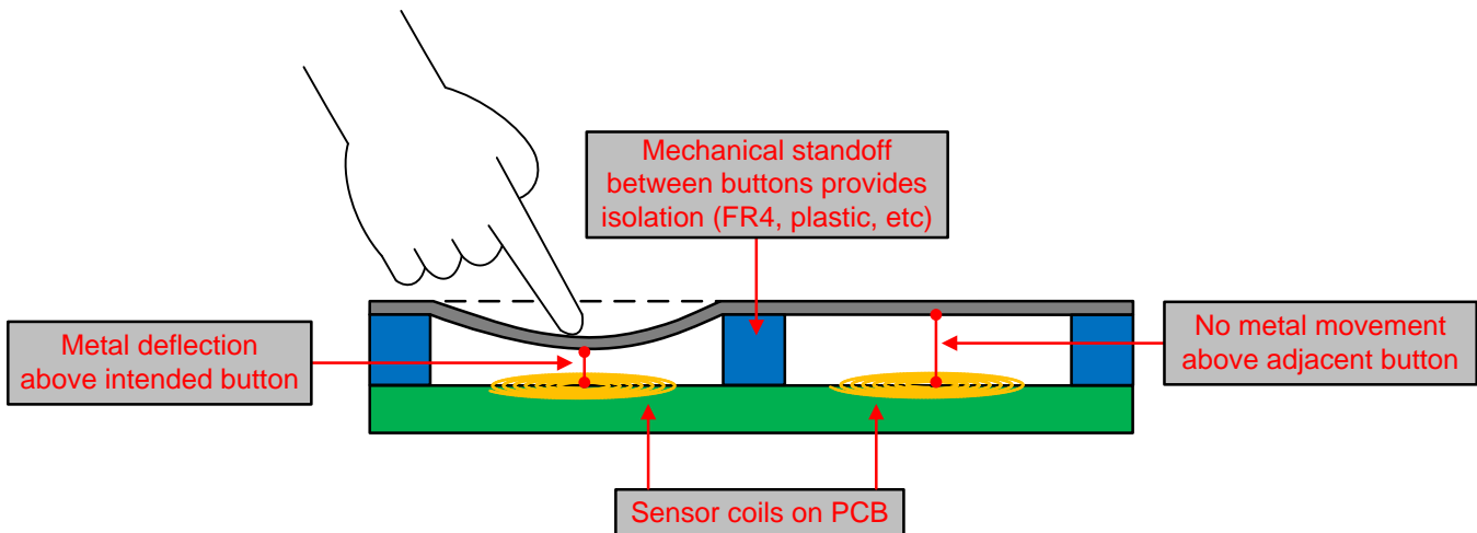
図 9. Mechanical Isolation Between Buttons
