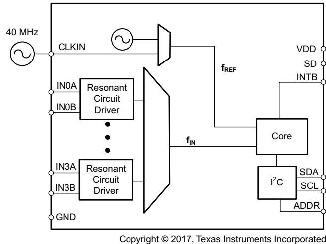
図 3. LDC1614 Functional Block Diagram
