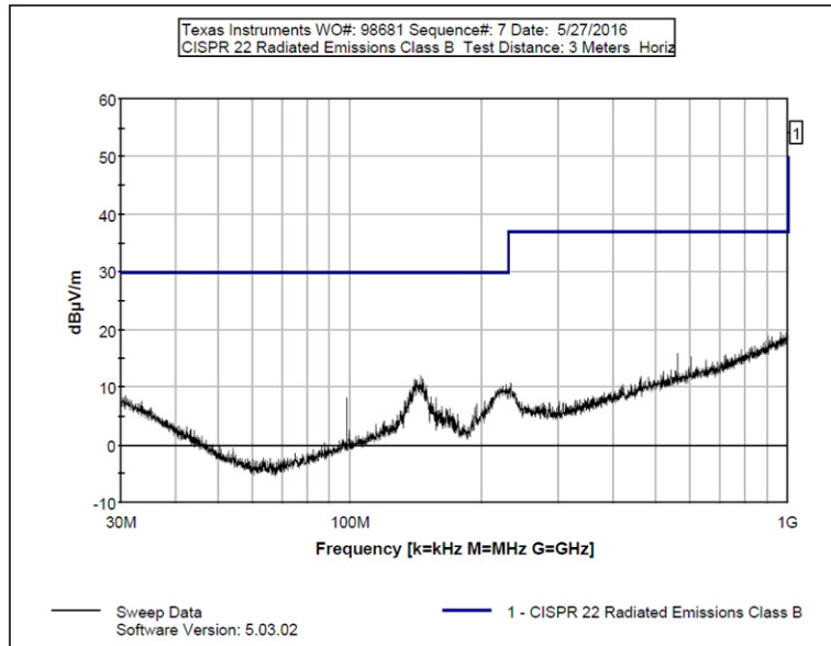
☒ 46. TIDA-01102 CISPR 22 Results for Horizontal Orientation
