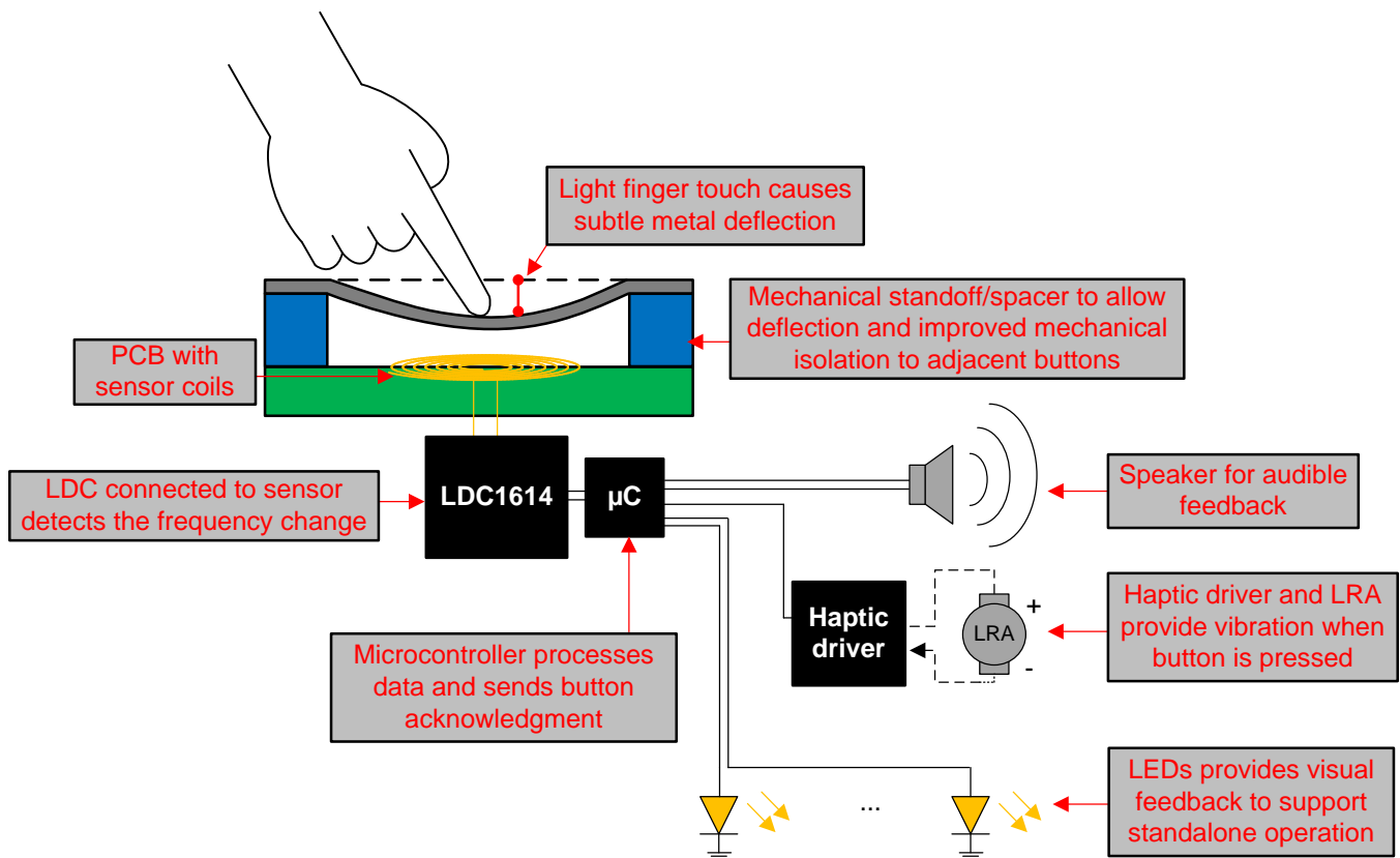
図 5. System Functional Diagram
