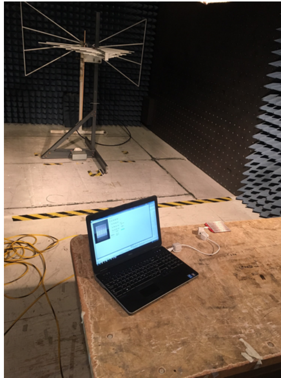
図 47. EMI Setup for CISPR 24 Susceptibility Testing
