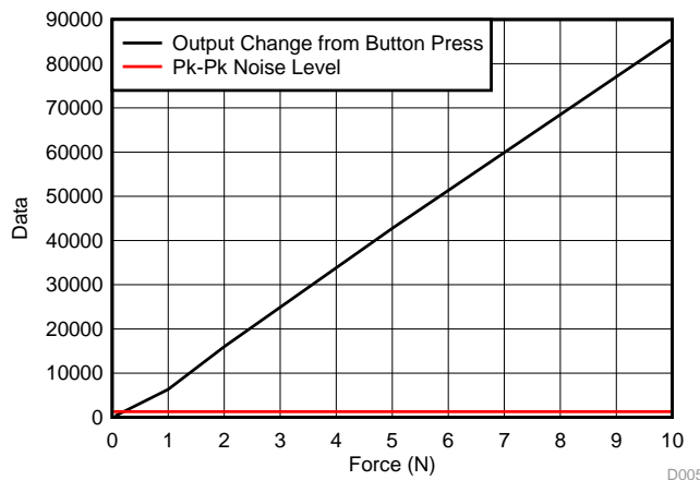
39. Code Change versus Force
