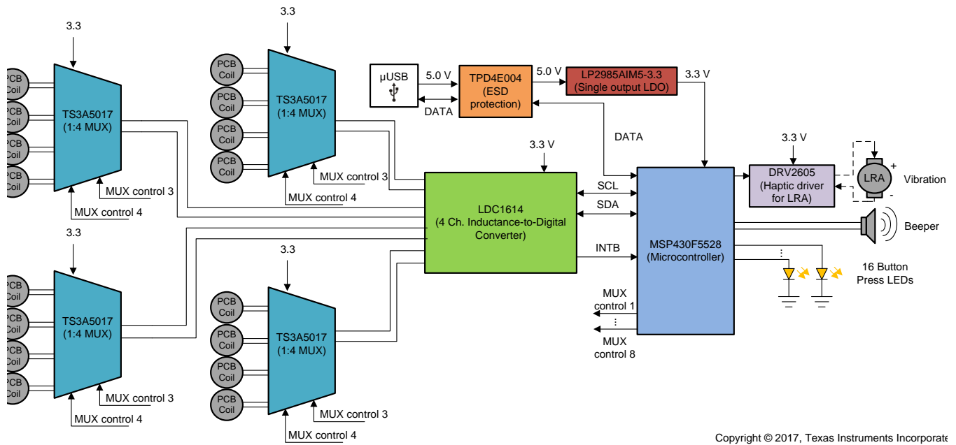
☒ 2. System Block Diagram
