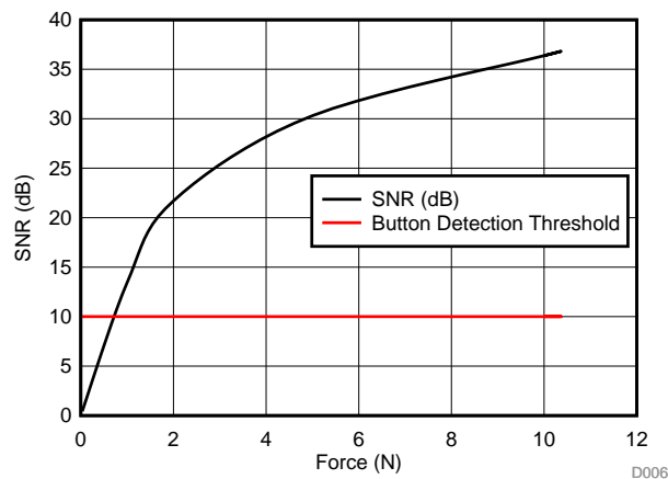
図 40. SNR in dB versus Force
