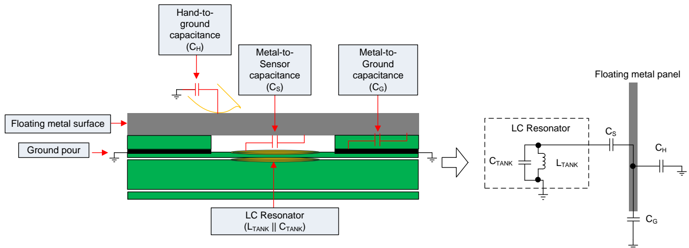
図 12. Capacitive Effect of Floating Metal Surface
