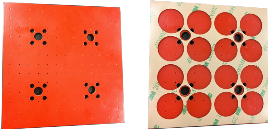
図 27. FR4 Stiffener With 9492MP Pre-Applied (Front and Back)
