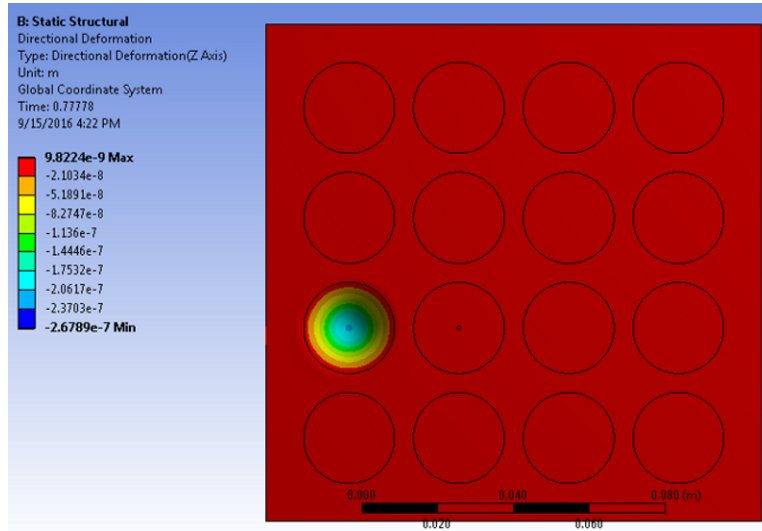
図 8. Simulation of Button Deflection for TIDA-01102
