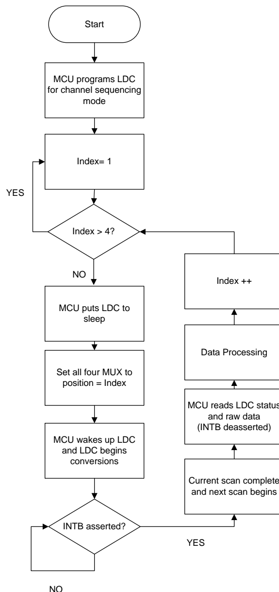
Figure 15. Data Collection Flow Chart for Single LDC1614 Device and Four TS3A5017 Devices
