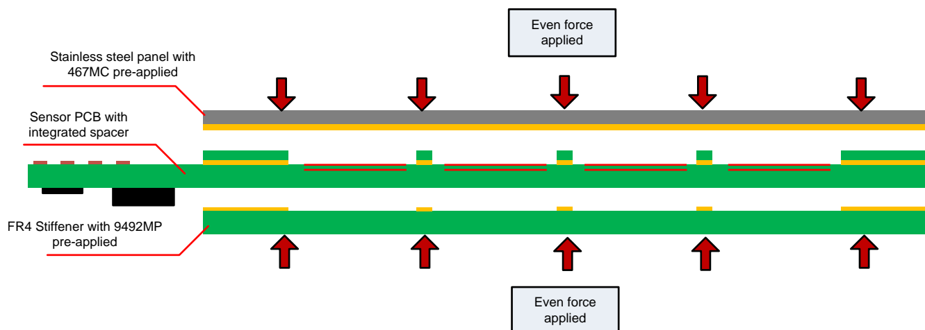
図 28. Assembly Process
