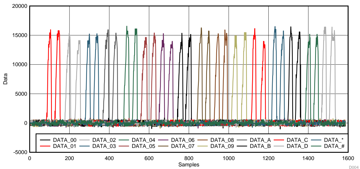
38. Time Domain TIDA-1102 Response With 2-N Force Applied to Each Button Twice
