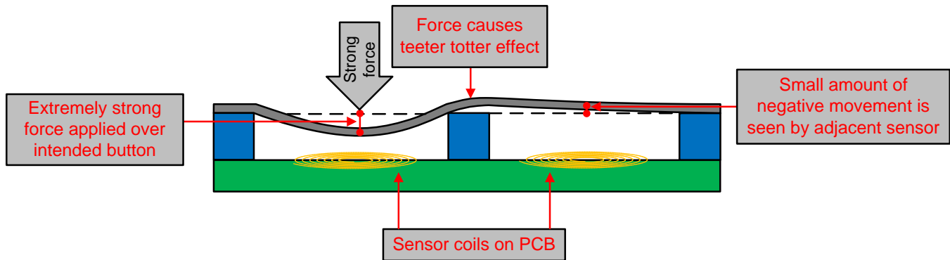
図 35. Extremely Strong Force Causing Teeter Totter Effect
