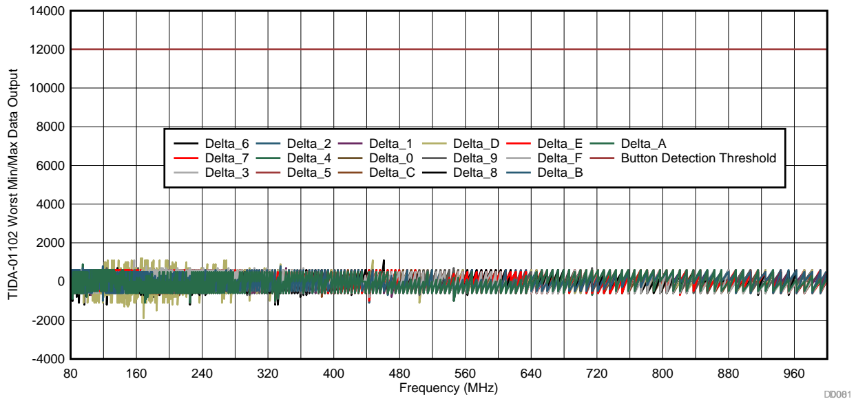
図 48. TIDA-01102 CISPR 24 EMI Susceptibility Raw Output
