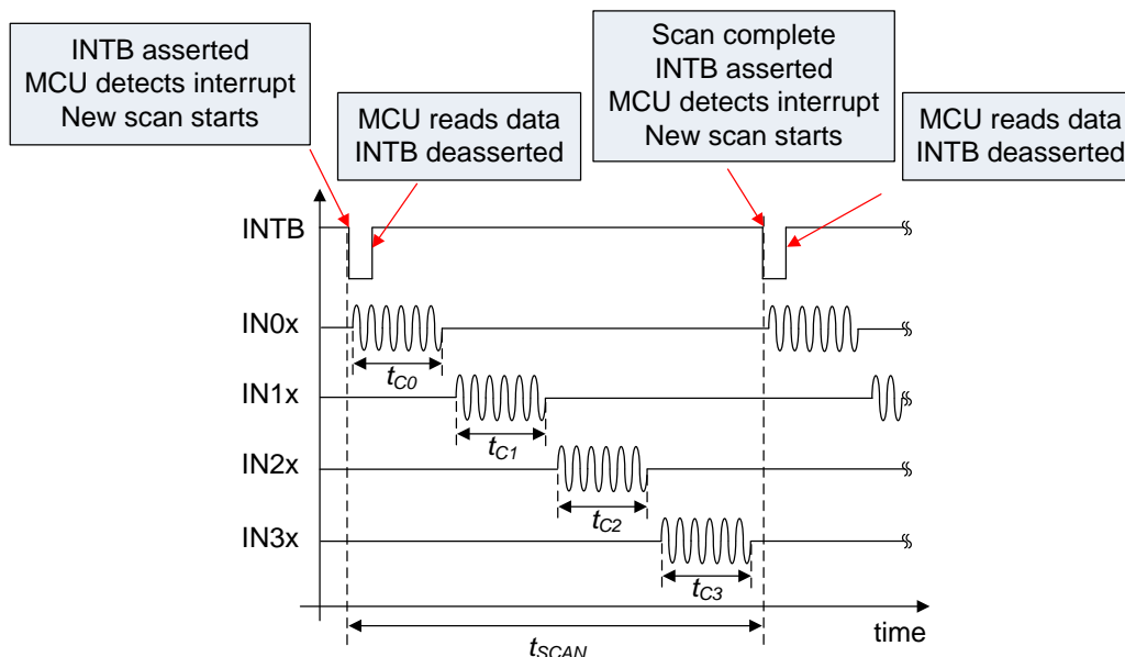
図 13. LDC1614 Scanning and Data Ready Timing Diagram
