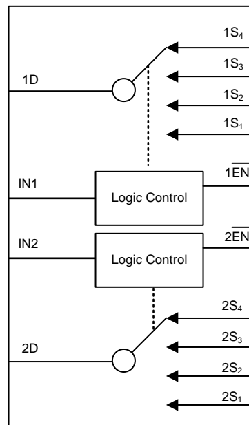
図 4. TS3A5017 Functional Block Diagram
