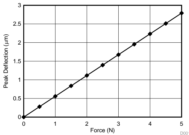
図 7. Force versus Deflection for TIDA-01102
