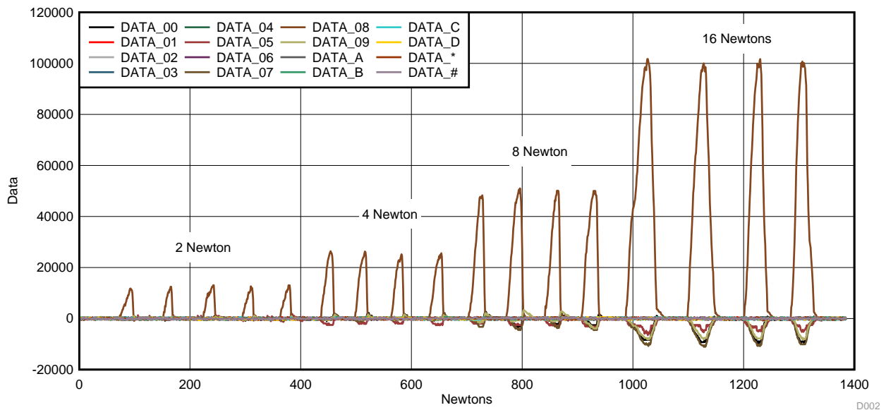
図 34. TIDA-01102 Output Response With 2-, 4-, 8-, and 16-N Force
