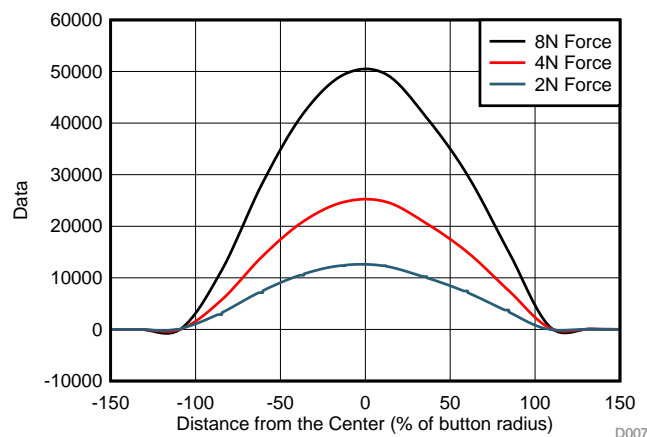
図 42. Output Code versus Button Press Location
