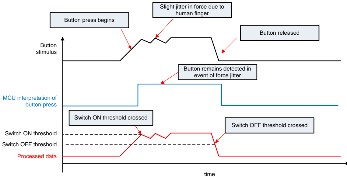
図 21. Hysteresis on Button Threshold Prevents Flickering Output State
