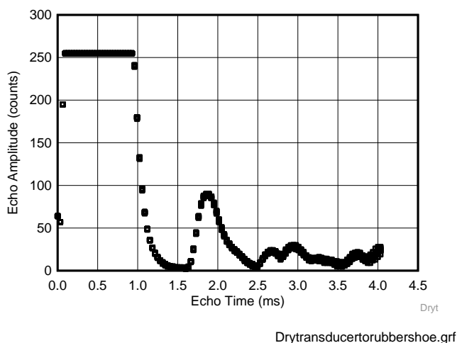
☒ 60. Response With Normal Transducer to Rubber Shoe
