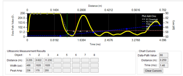
☒ 40. Sports Shoe Detected at 255 mm
