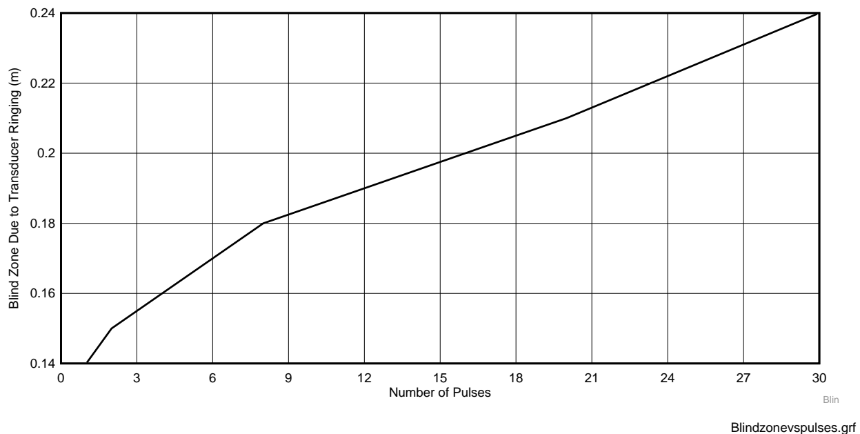
Figure 25. Effect of Increasing Number of Applied Pulses on Minimum Measurable Distance
