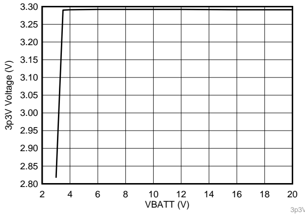
Figure 20. 3.3-V Supply Voltage Versus Input Voltage
