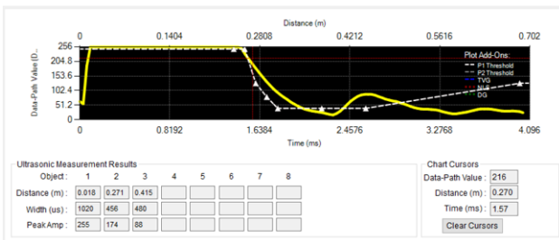
47 . Detection of Foot at 271 mm Using PUI Transducer
