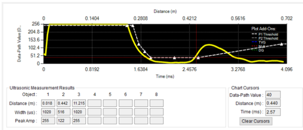
43 . Detection of Ground at 442 mm Using PUI Transducer
