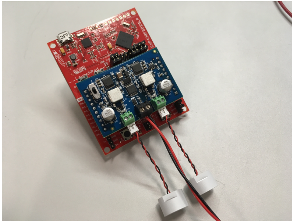
☒ 13. TIDA-01424 Board Mounted on MSP430™ LaunchPad™ Board
