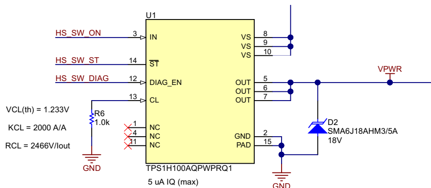
Figure 8. Electrical Schematic of High-Side Switch for Applying Power to Ultrasonic Transducer Circuits
