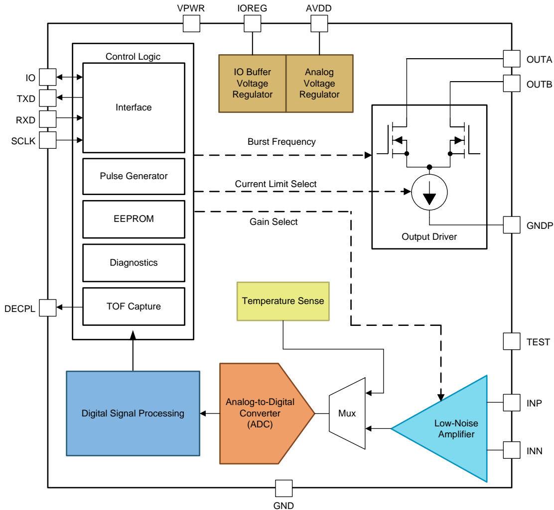
Figure 2. Functional Block Diagram of PGA460-Q1
