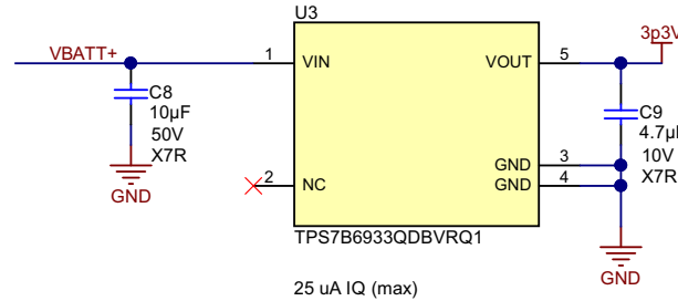
図 6. Electrical Schematic of 3.3-V Supply Regulator Circuit
