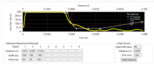
46 . Detection of Foot at 292 mm Using PUI Transducer
