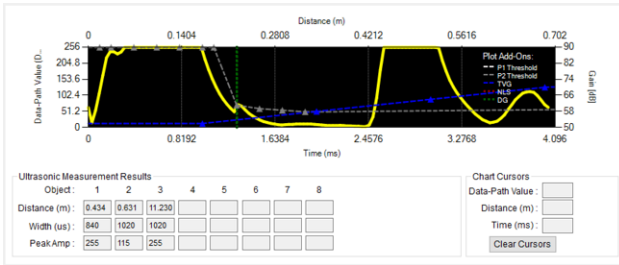
Figure 28. Echo With Rubber Top Shoe, Ground Detection
