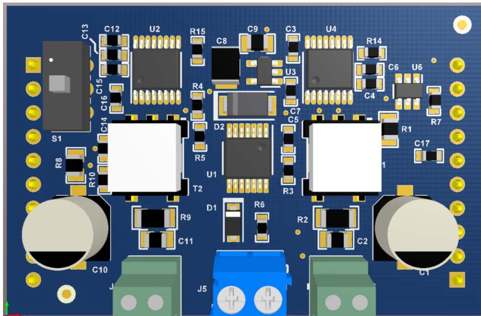
☒ 66. Top View of TIDA-01424 Board
