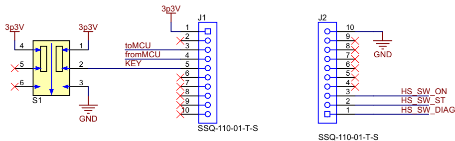
Figure 10. Electrical Schematic of MCU Interface
