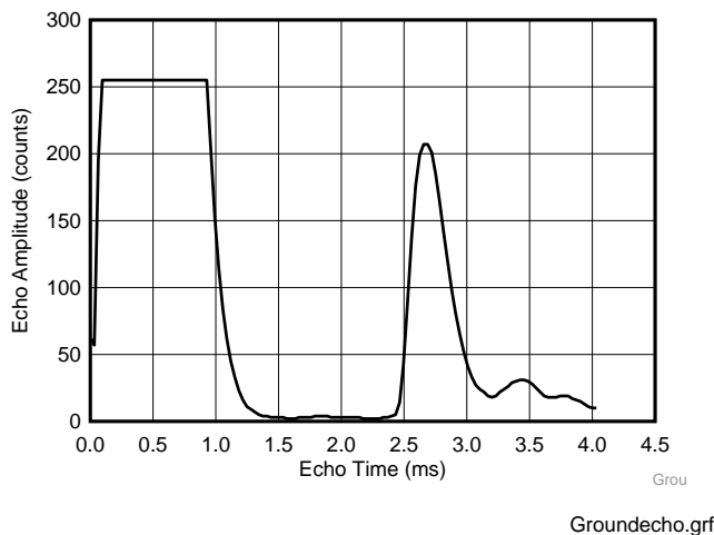
Figure 62. Echo From Ground Beneath Bumper
