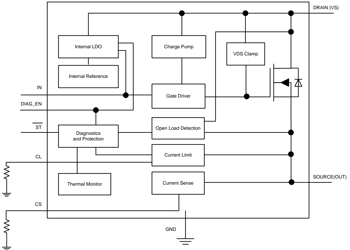
☒ 3. Functional Block Diagram of TPS1H100-Q1
