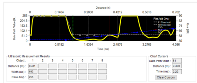
[34]. Sports Shoe Echo Below Threshold, Ground Detected at 431 mm
