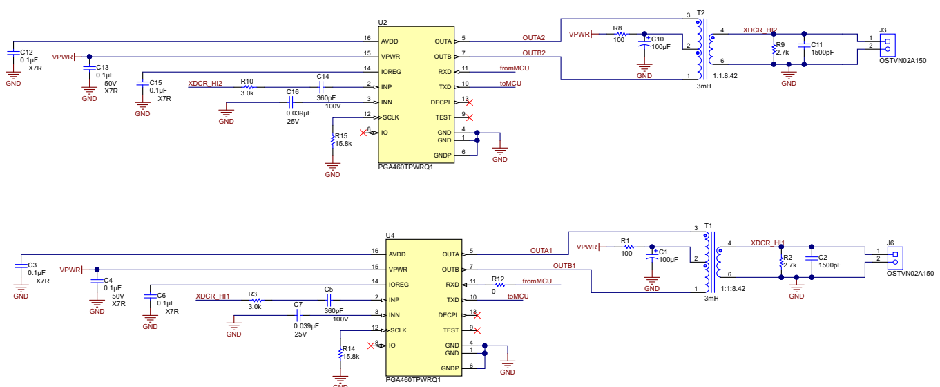
Figure 9. Electrical Schematic, Ultrasonic Transducer Driver and Echo Receiver Circuit
