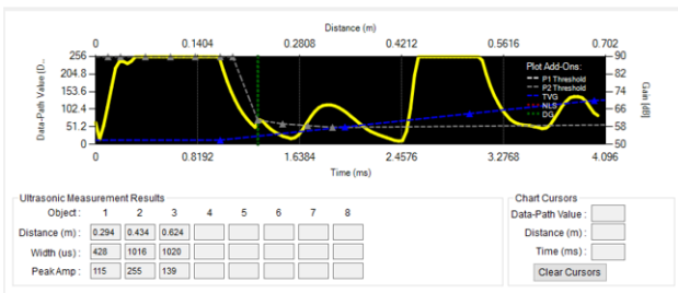
Figure 30. Echo With Rubber Top Shoe, Detection of Shoe at 294 mm
