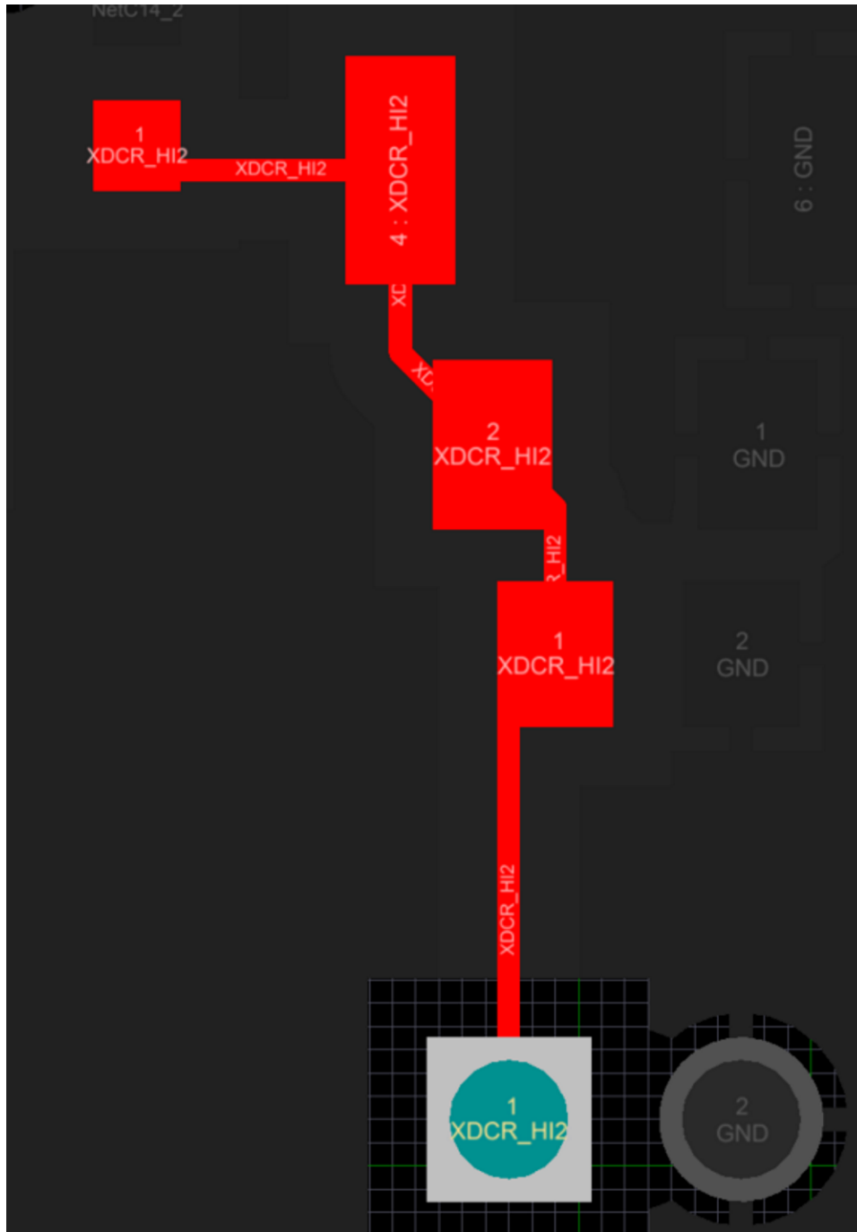
図 68. XDCR_HI2 Signal Trace
