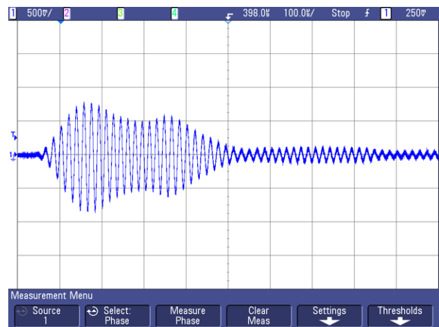
Figure 24. Ultrasonic Acoustic Waveform, R = 10 kΩ, C = 700 pF
