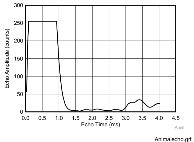
Figure 63. Echo From Stuffed Animal Beneath Bumper
