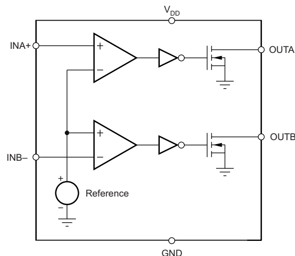
Figure 5. Functional Block Diagram of TPS3700-Q1
