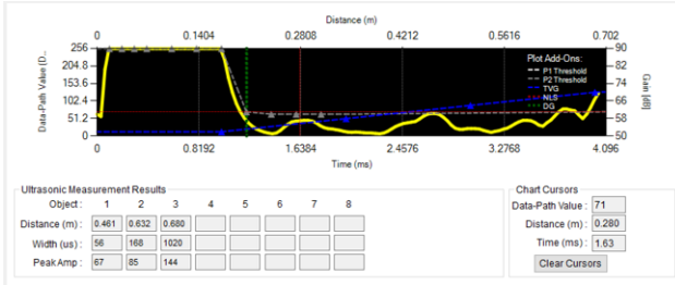
☒ 39. Sports Shoe Echo Below Threshold at 260 mm, Ground Detected at 461 mm
