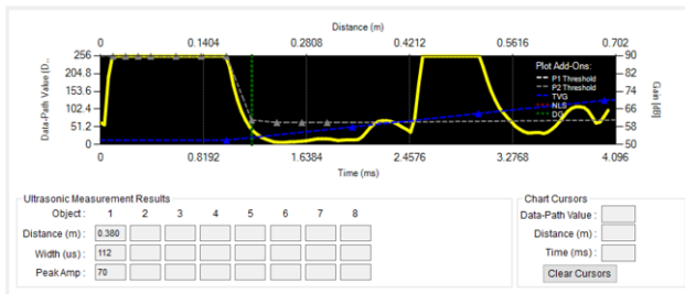
[33]. Sports Shoe Detected at 380 mm
