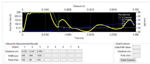
Figure 32. Echo With Rubber Top Shoe, Detection of Shoe at 232 mm
