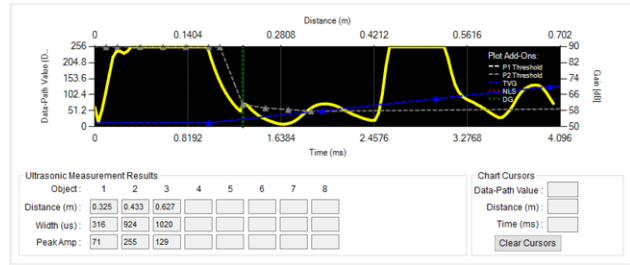
Figure 29. Echo With Rubber Top Shoe, Detection of Shoe at 325 mm
