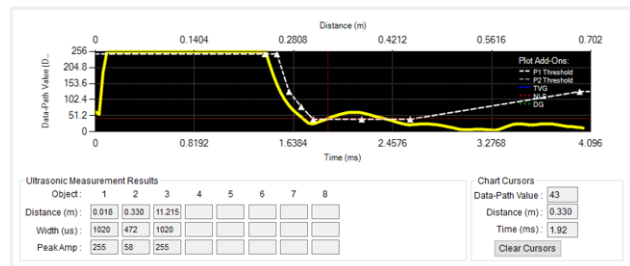
48 . Foot Not Detected Closer Than 270 mm, Secondary Surface Detected at 330 mm, Using PUI Transducer
