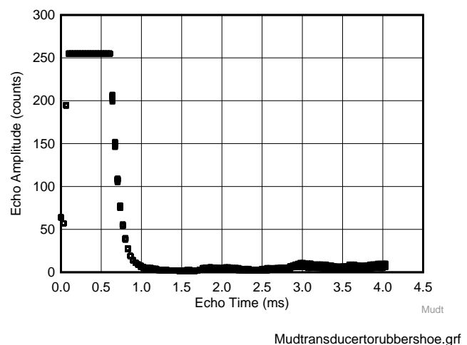
☒ 61. Response With Muddy Transducer to Rubber Shoe
