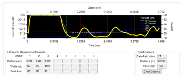
[38]. Sports Shoe Detected at 282 mm
