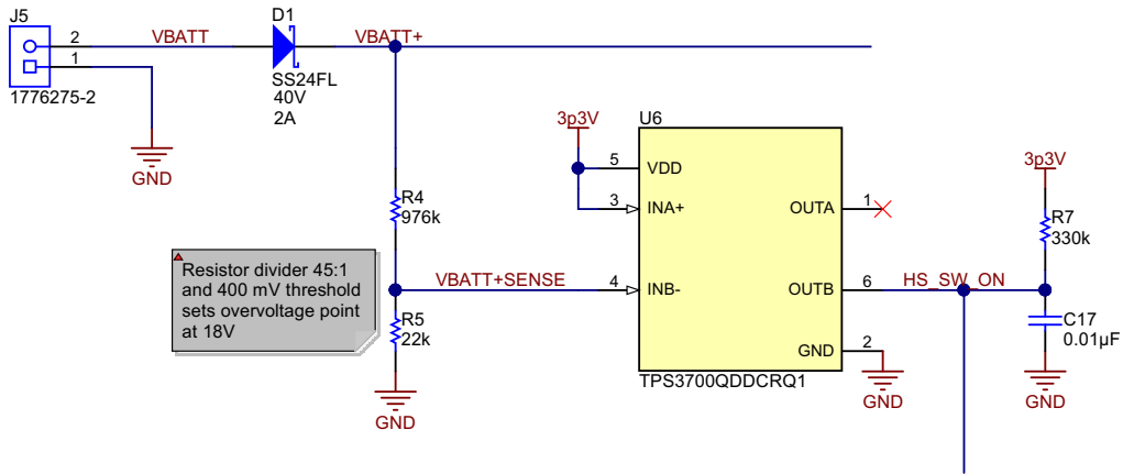
図 7. Electrical Schematic of Input Power Protection Circuit
