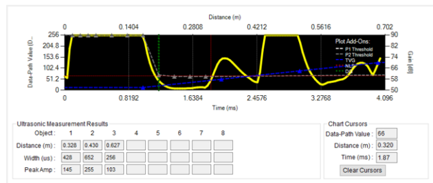
[36]. Sports Shoe Detected at 328 mm
