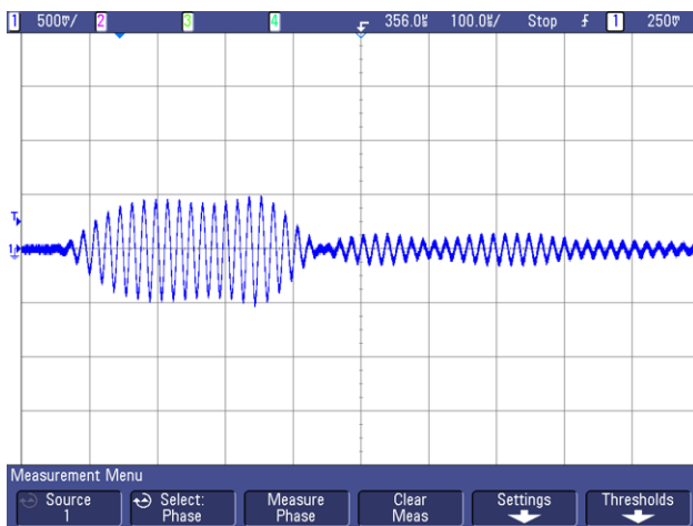
Figure 23. Ultrasonic Acoustic Waveform, R = 2.7 kΩ, C = 1500 pF
