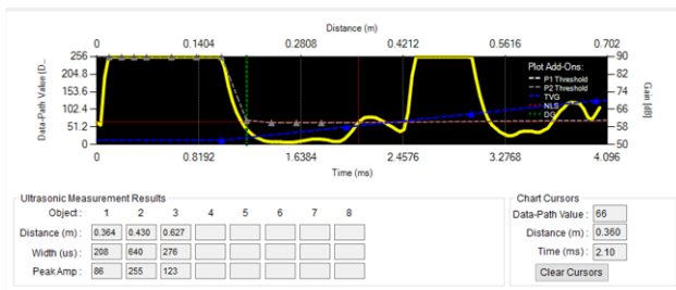
[35]. Sports Shoe Detected at 364 mm
