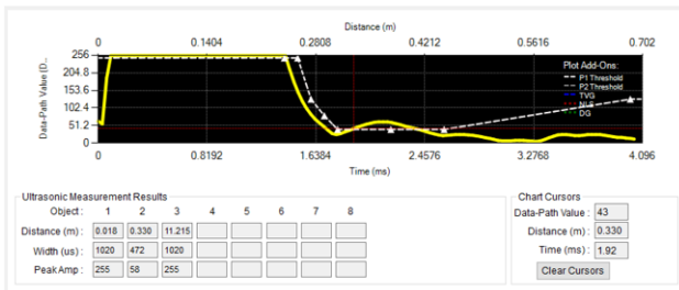
45 . Detection of Foot at 330 mm Using PUI Transducer
