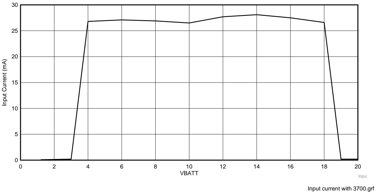
Figure 17. Input Current Versus VBATT Voltage, Showing TPS3700-Q1 Threshold at 18 V, TIDA-01424 Board Only
