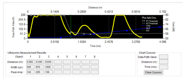
Figure 31. Echo With Rubber Top Shoe, Detection of Shoe at 262 mm
