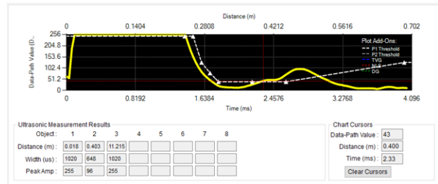
44 . Detection of Foot at 403 mm Using PUI Transducer
