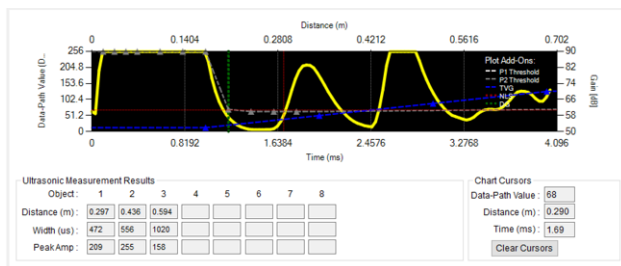
[37]. Sports Shoe Detected at 297 mm
