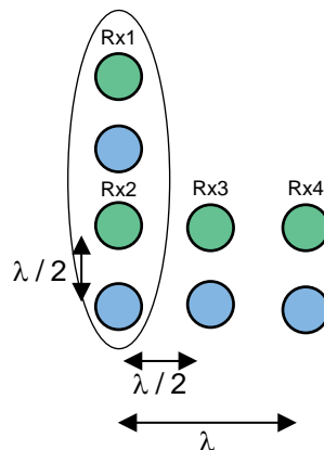
図 5. Virtual Antenna Array for Range-Elevation-Angle Heat-Map Calculation
