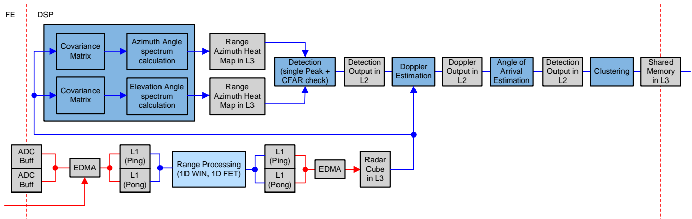
図 4. System Process Chain
