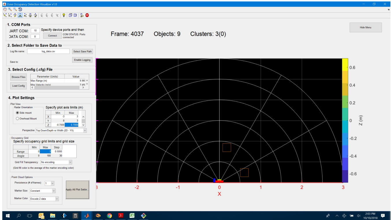
Figure 10. Horizontal Concrete Block and Plastic Reflector - 2D View
