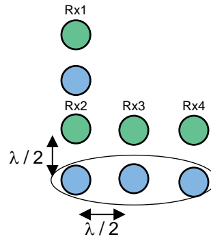
図 6. Virtual Antenna Array for Range-Azimuth-Angle Heat-Map Calculation
