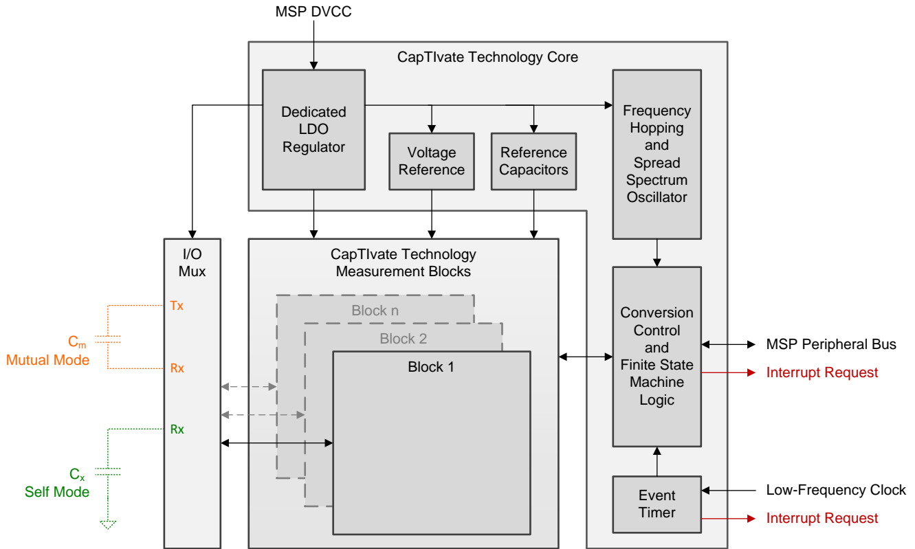
図 3. CapTlvate Technology Block Diagram
