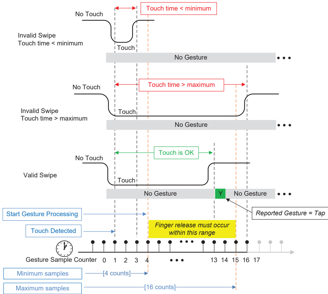
図 7. Tap Gesture Detection
