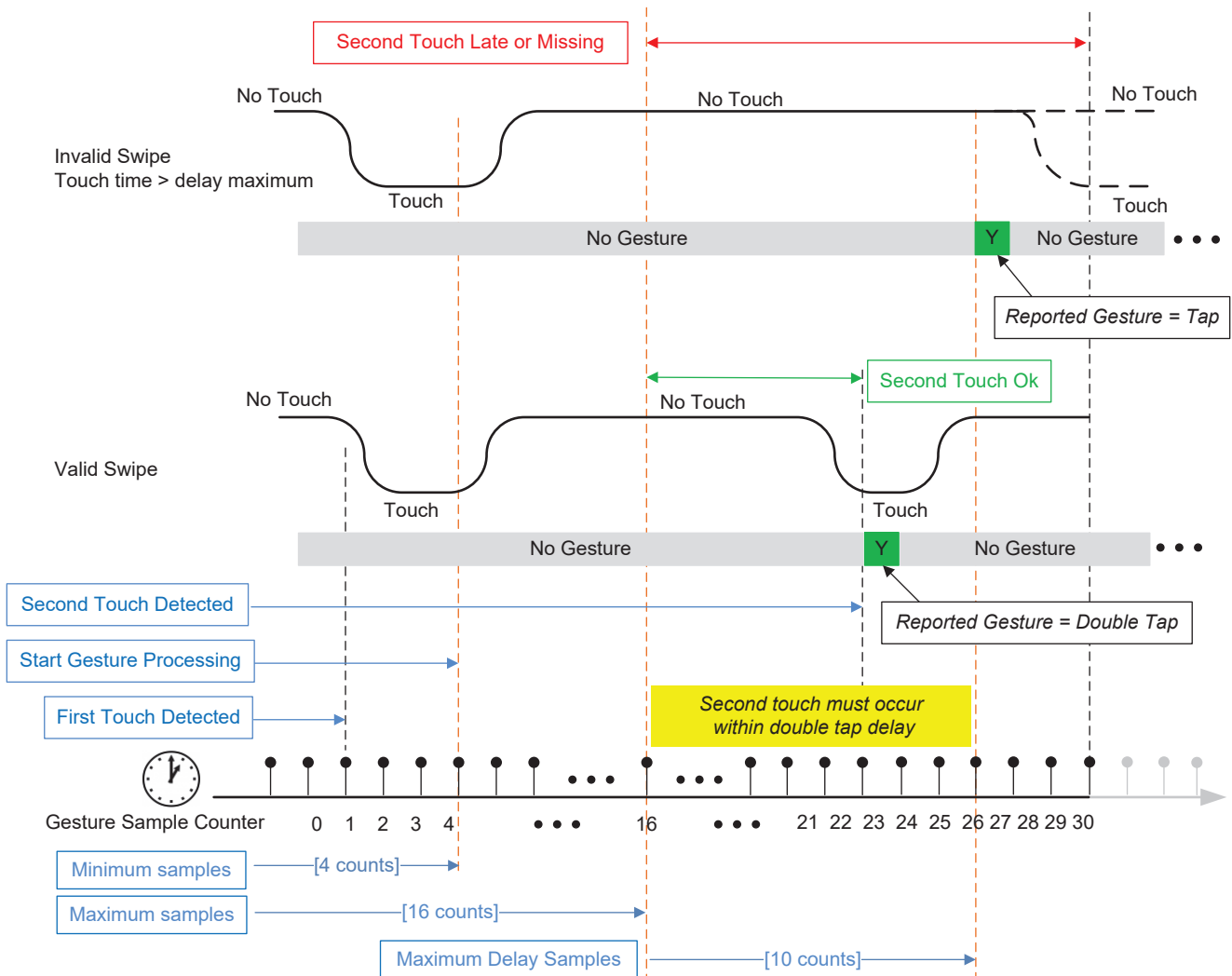
8. Double Tap Gesture Detection
