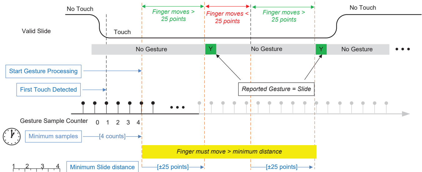
Figure 11. Slide Gesture Detection
