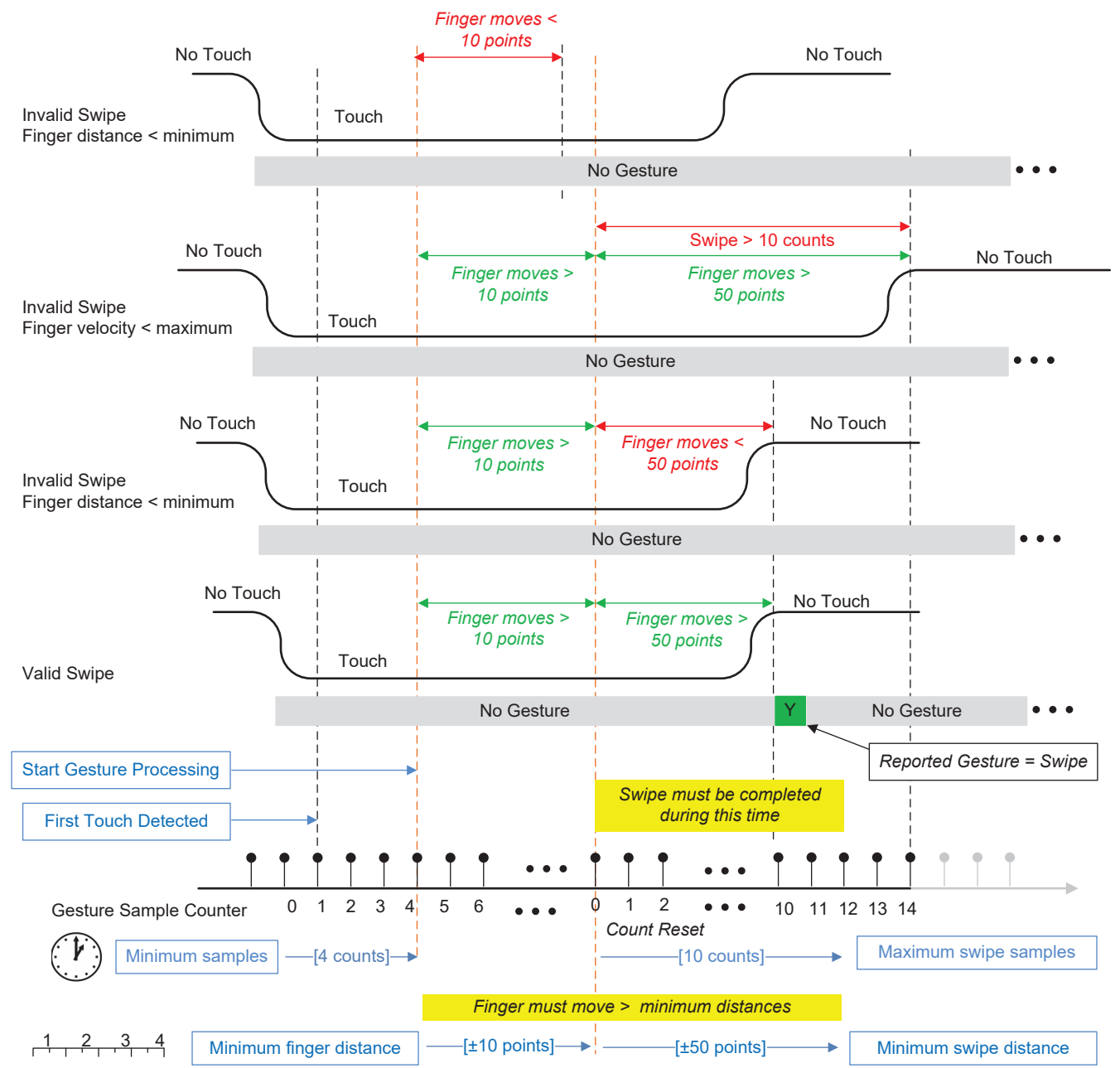
図 10. Swipe Gesture Detection
