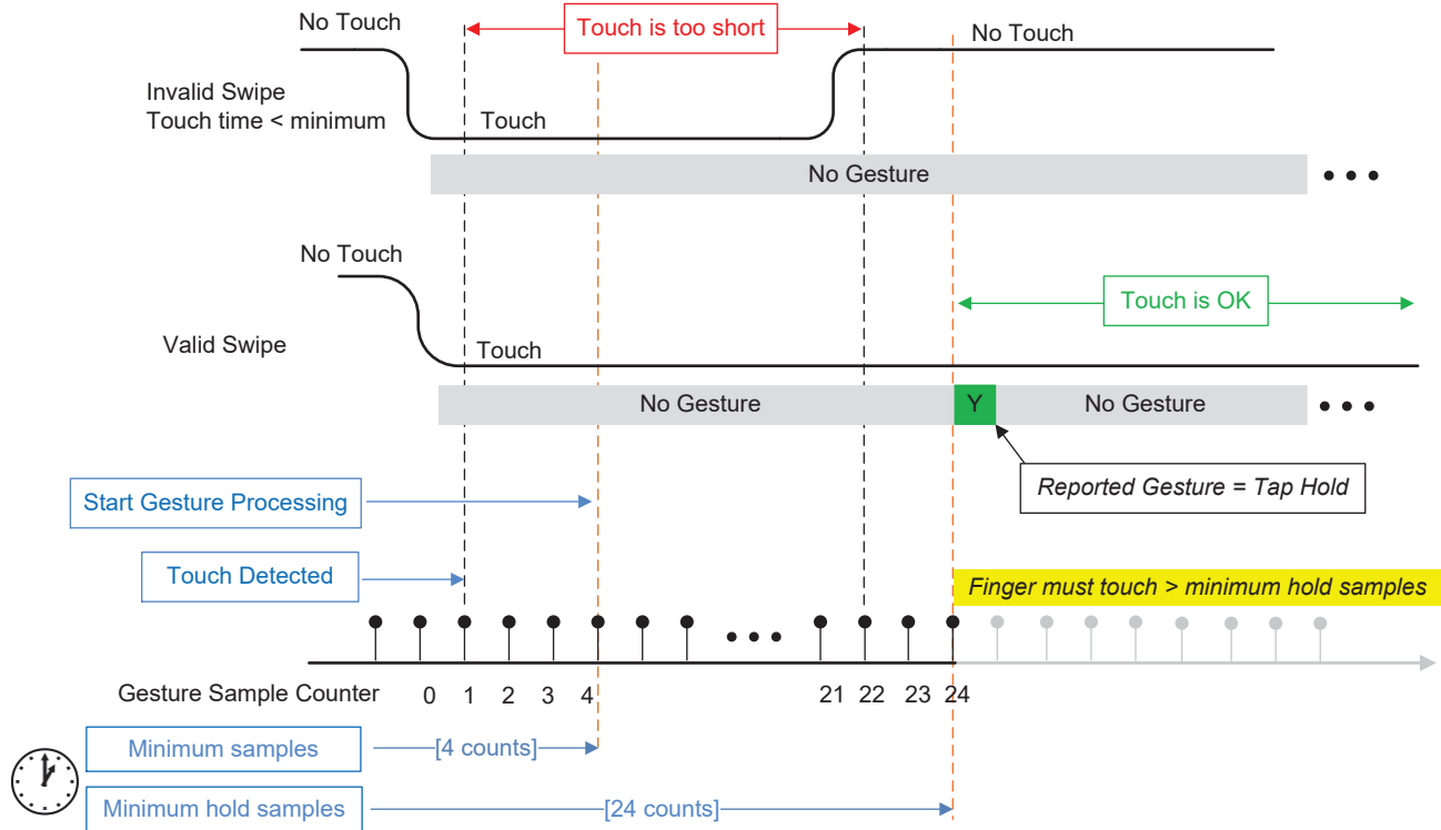
図 9. Tap-and-Hold Gesture Detection
