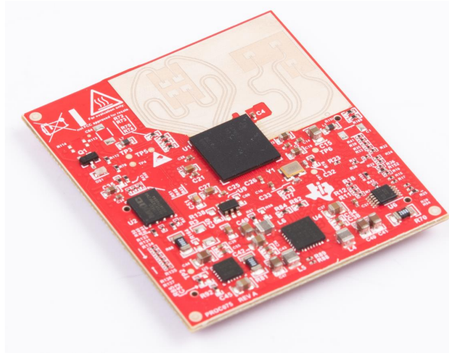
図 4. IWR6843ISK-ODS Board View
