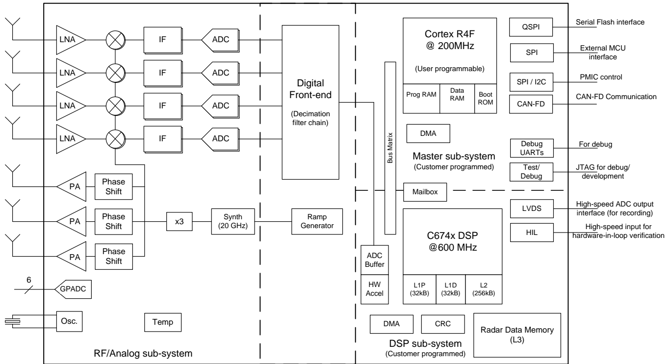
図 2. IWR6843 mmWave Sensor Functional Block
