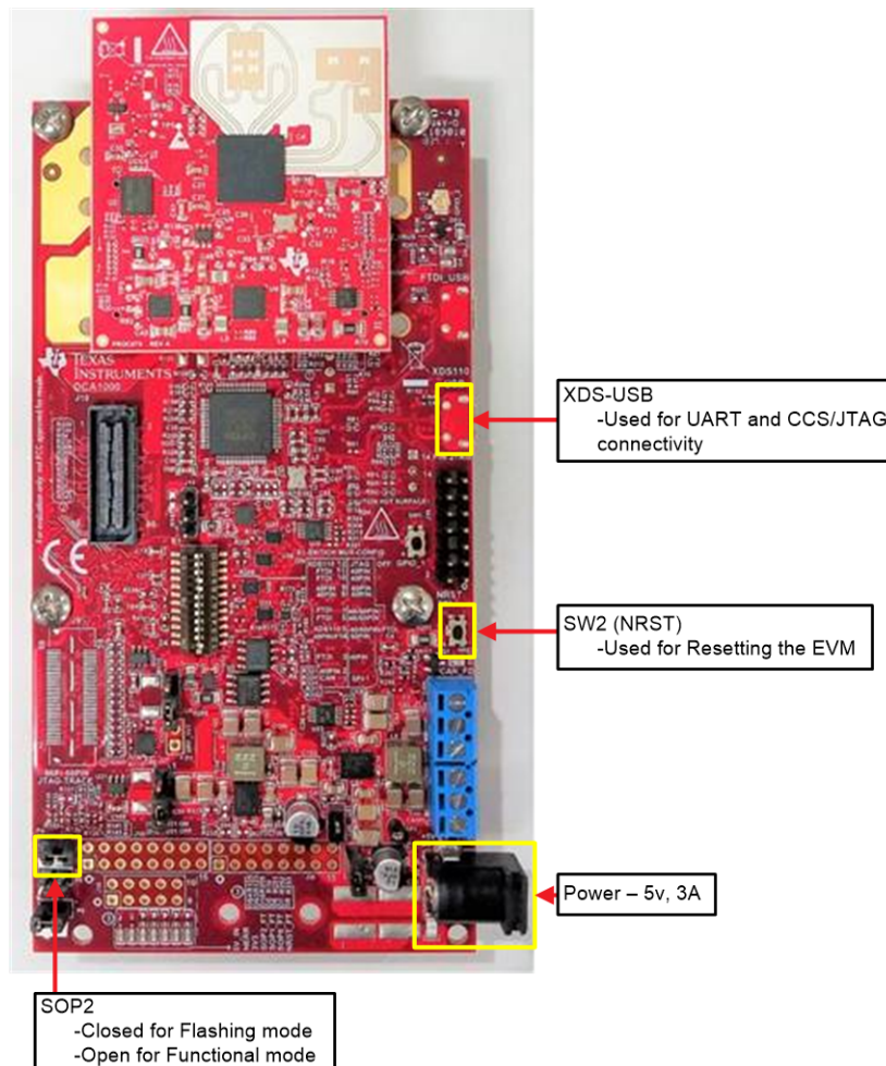
Figure 5. mmWave EVM: MMWAVEICBOOST + IWR6843ISK-ODS
