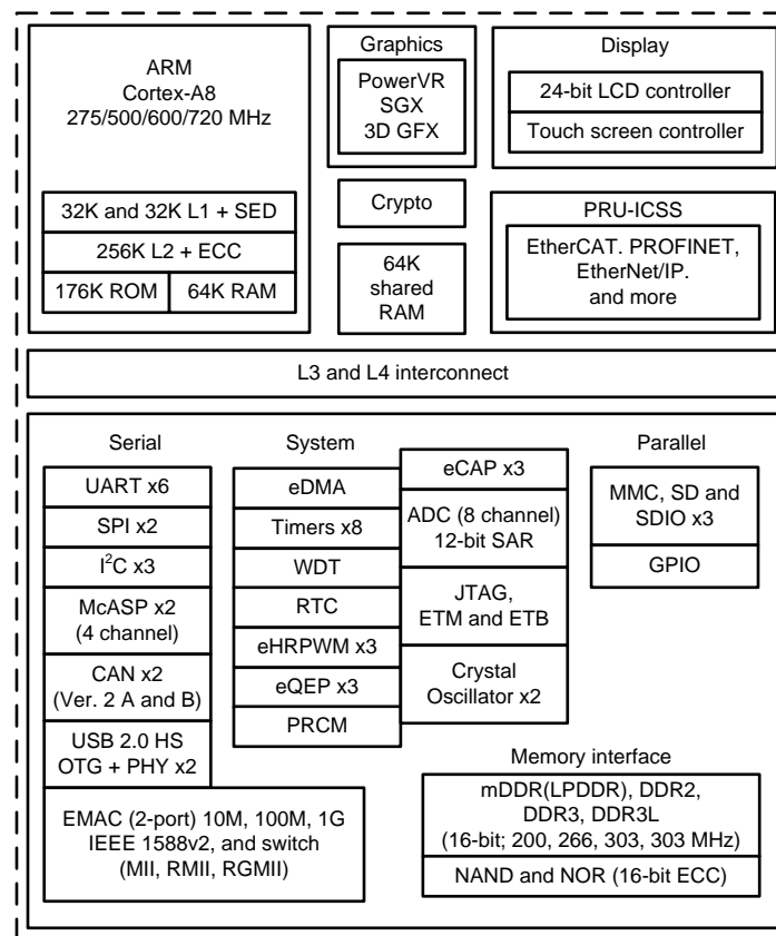
Figure 1. AM335x Processor Block Diagram
