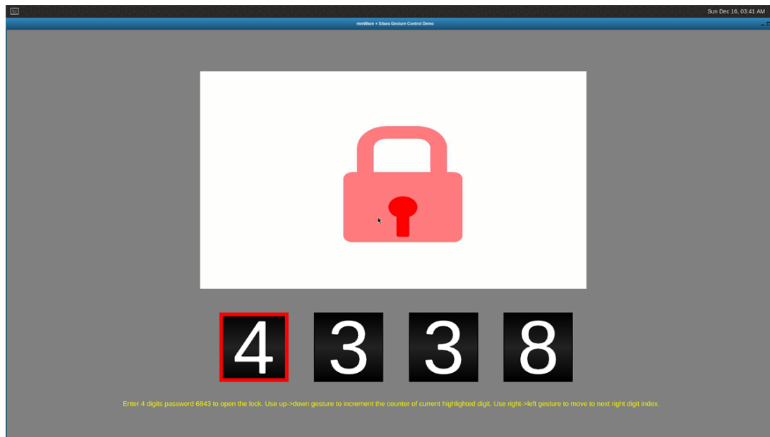
Figure 11. Down-Swipe Gesture
