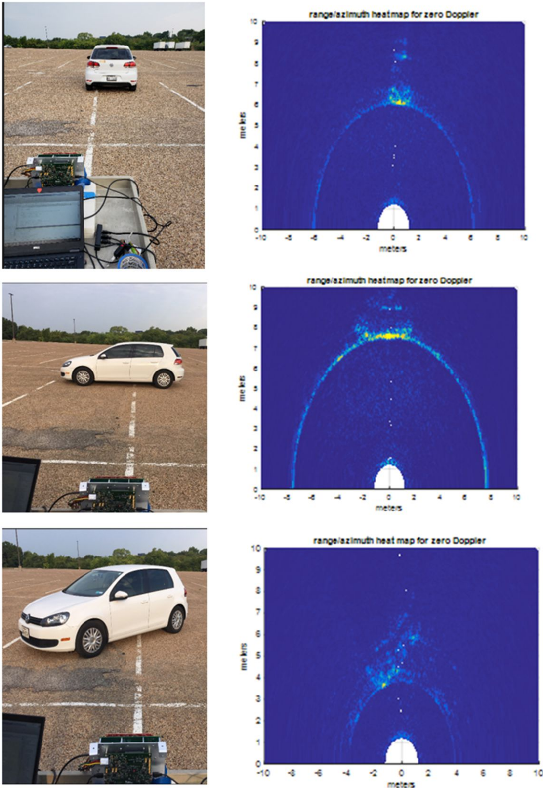
図 13. Car at 0 Degrees (Top), 90 Degrees (Middle) and 135 Degrees (Bottom) Orientation and Corresponding Azimuth Range Heatmap
