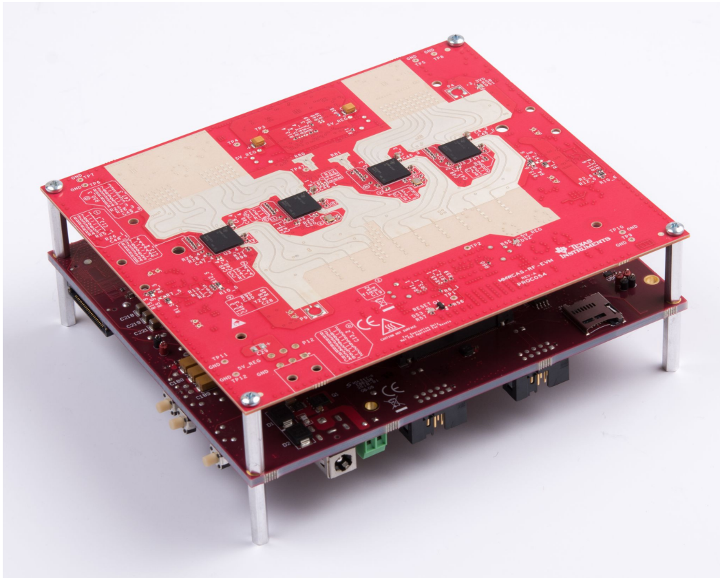
図 1. AWR1243P Four-Device Cascade Radar RF Radar Board
