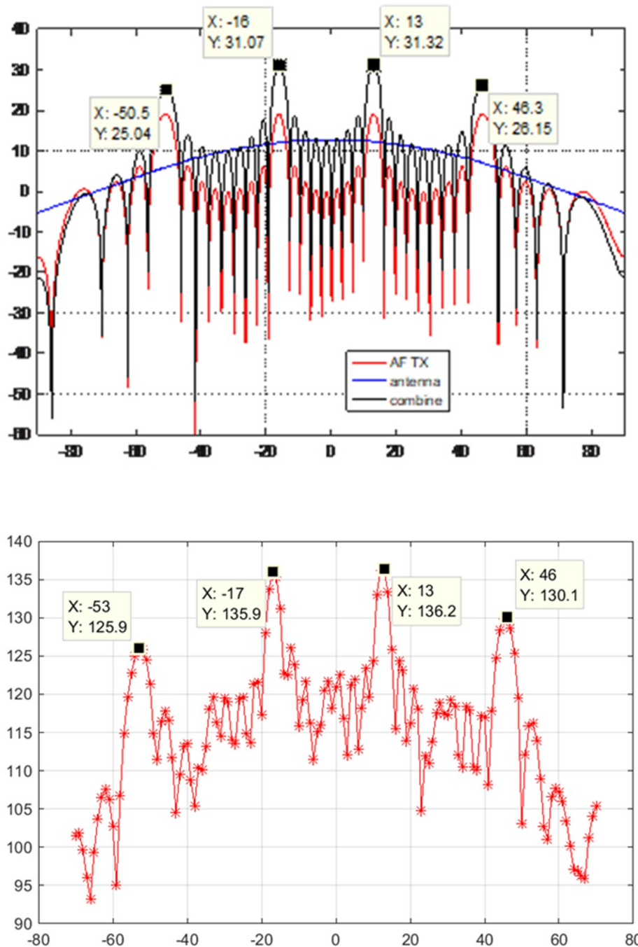
図 15. Simulated (Top) and Measured (Bottom) 15 Degree Beam Steering Test
