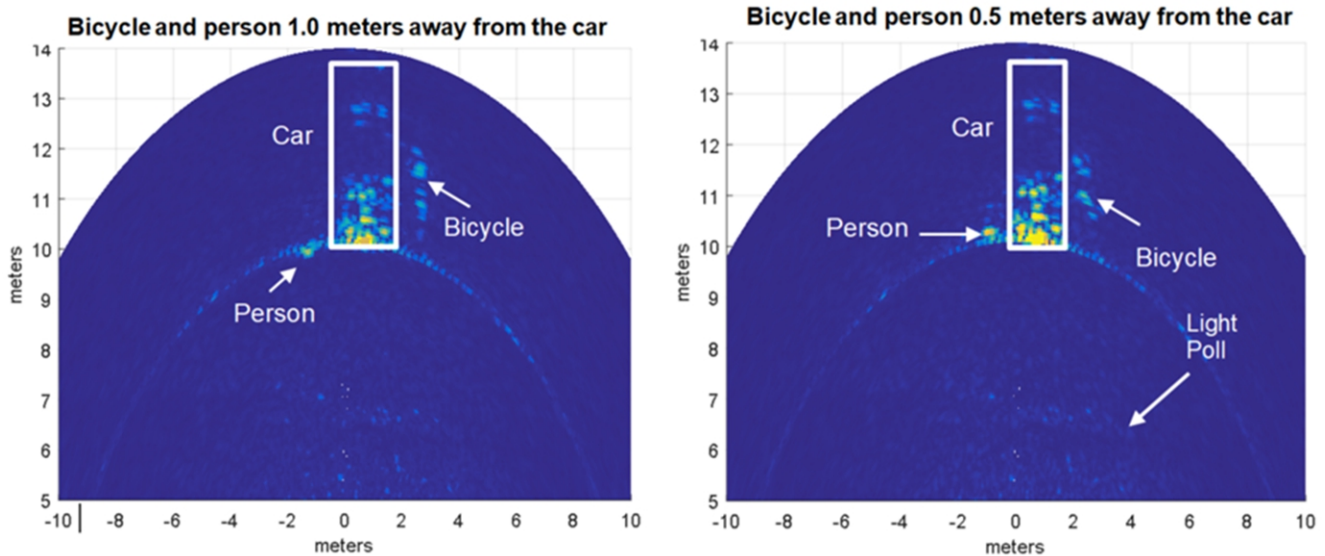
図 12. Bicycle and Person 1.0 m (Left) and 0.5 m (Right) Away From Vehicle
