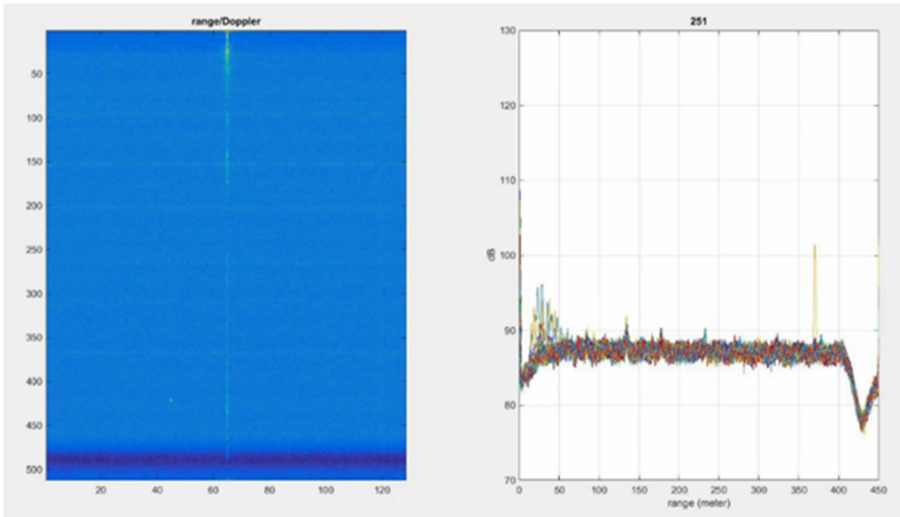
図 17. Range Profile (Left), and Doppler-Range Plot of a Vehicle 350-m Range
