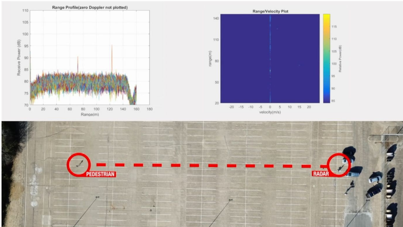
図 16. Range Profile (Top Left), and Doppler-Range Plot of a Pedestrian Jogging Away From Radar at 120-m Range
