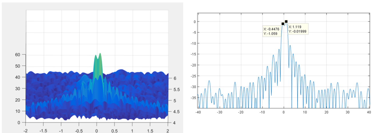
図 8. Range-Doppler FFT Plots Showing Detected, Separated Peaks From Both Reflectors
