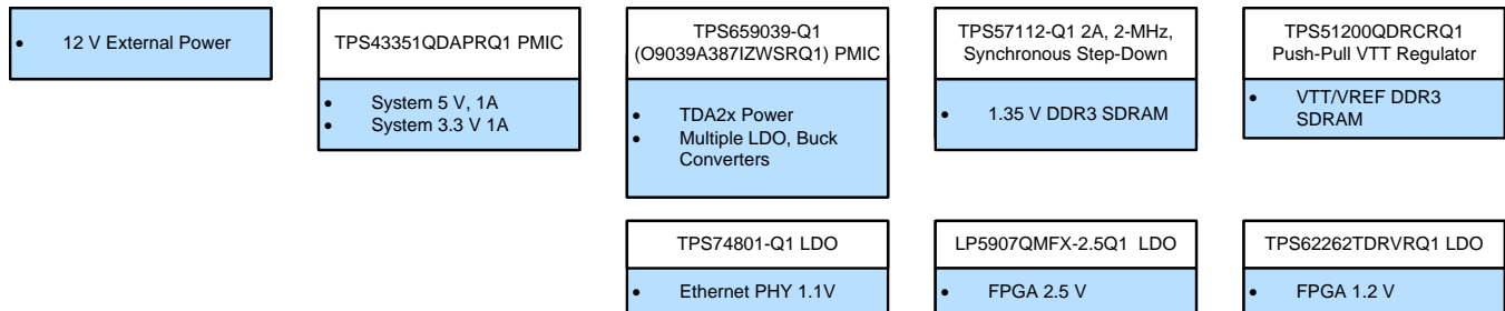
図 3. Cascade Radar Host Processor Power Block Diagram
