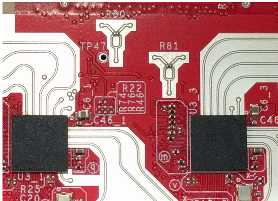
図 5. 20-GHz LO Distribution Board Implementation
