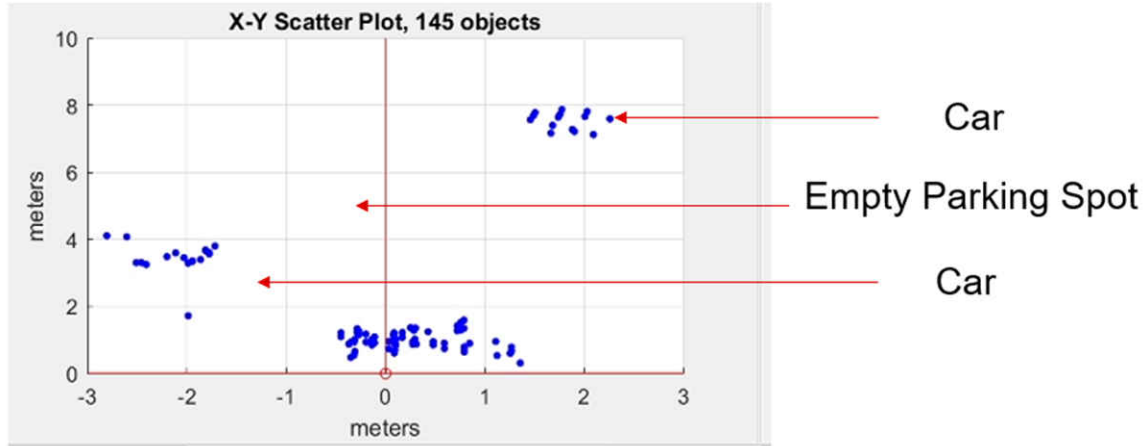
図 3-8. Detection Point Cloud of Empty Parking Space
