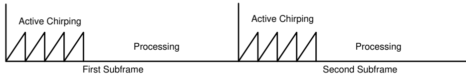
Figure 2-1. Multi-Mode Sub-Frames
