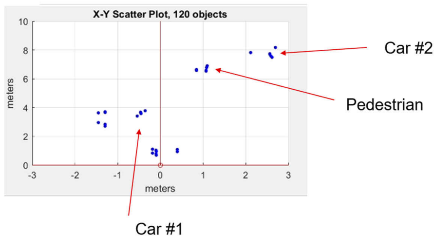
Figure 3-5. Detection Point Cloud of Pedestrian Standing in Empty Parking Space
