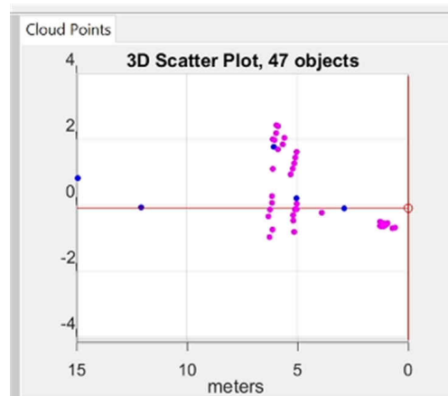
☒ 3-3. Detection Point Cloud of Traffic Sign Pole – Elevation View
