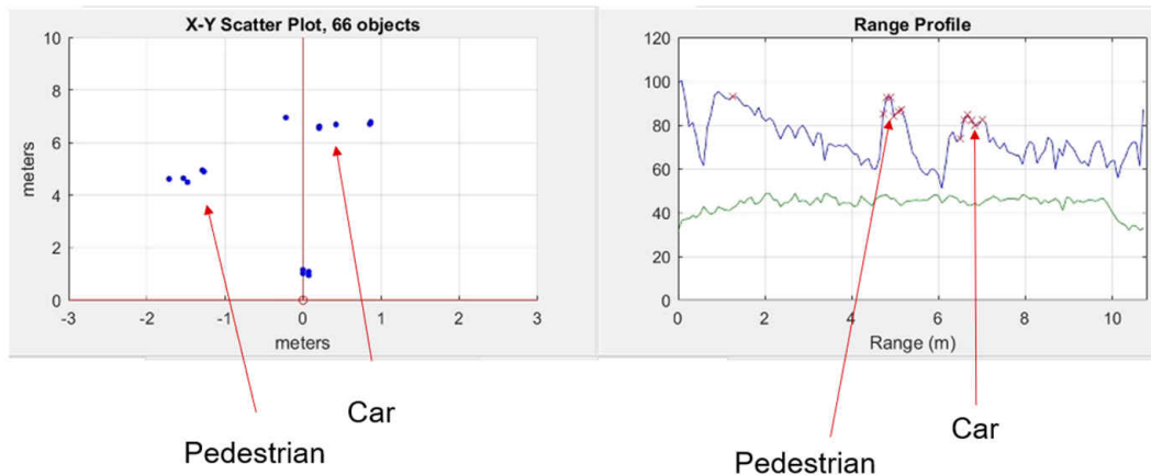
Figure 3-7. Point Cloud for Static Detection
