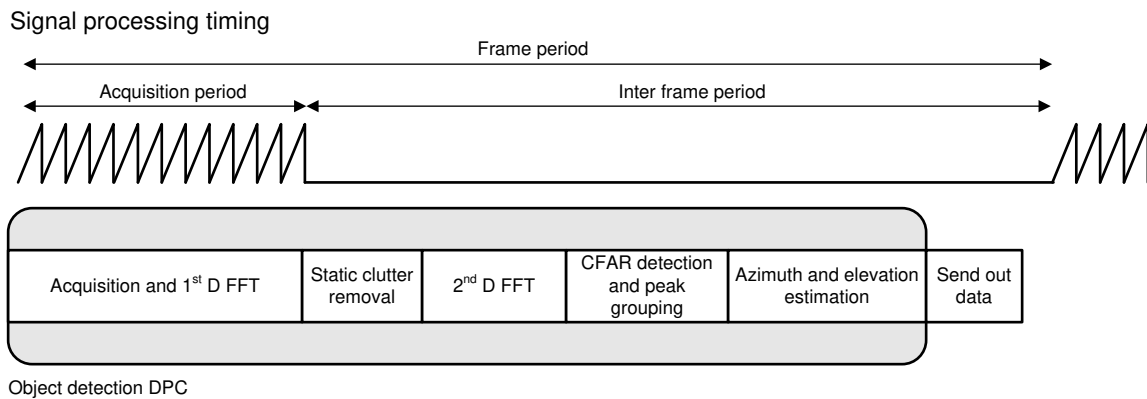
Figure 2-2. Datapath Processing and Timing
