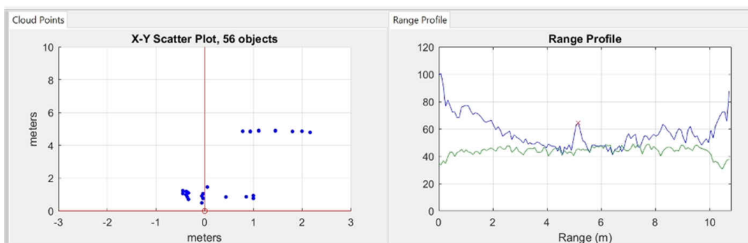
Figure 3-10. Detection Point Cloud of Parking Block
