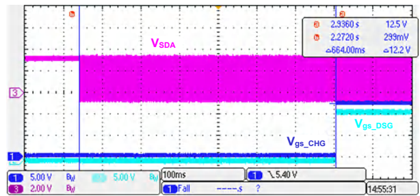
図 3-14. Hardware Watchdog Protection
