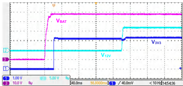
図 3-4. Auxiliary Start-Up
