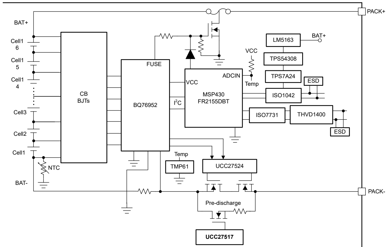
Figure 2-1. TIDA-010216 Block Diagram
