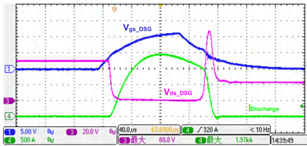
図 3-13. Short-Circuit Discharge Protection
