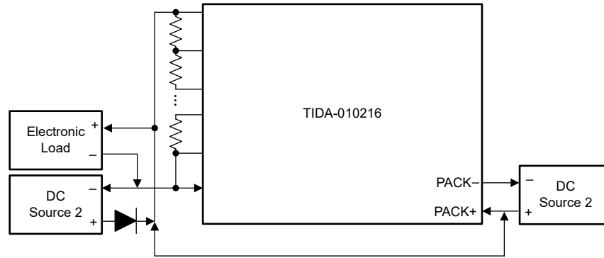
☒ 3-1. Charge Setup
