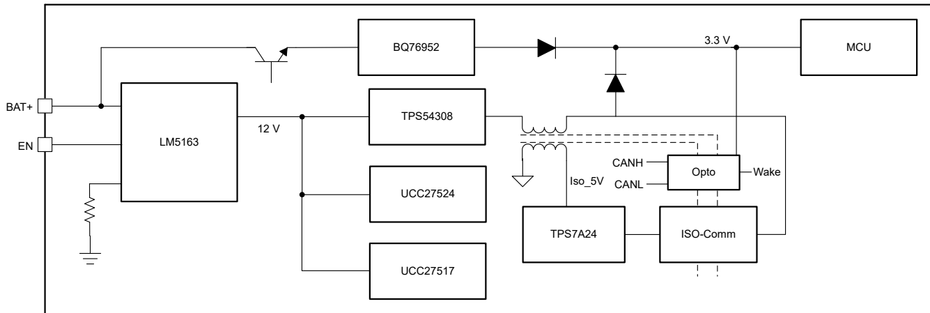
Figure 2-2. Auxiliary Power Architecture
