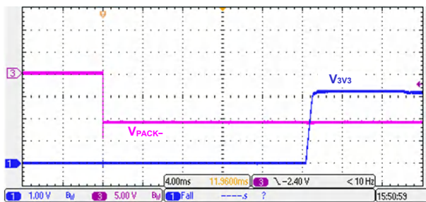
図 3-15. Ship Mode to Normal Mode
