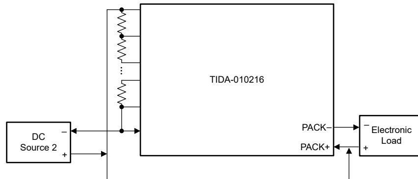
☒ 3-2. Discharge Setup
