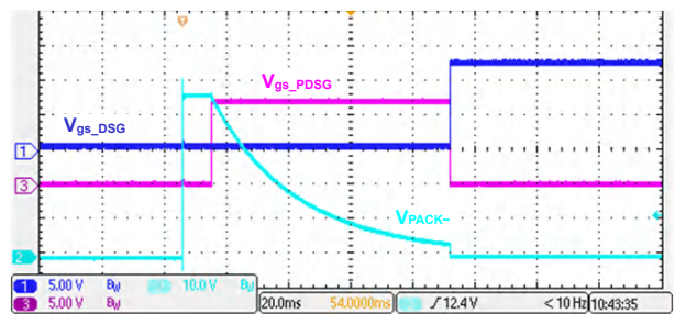
図 3-16. Capacitive Load Attach Detect
