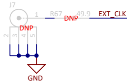
Figure 2-9. Optional External Clock Connection
