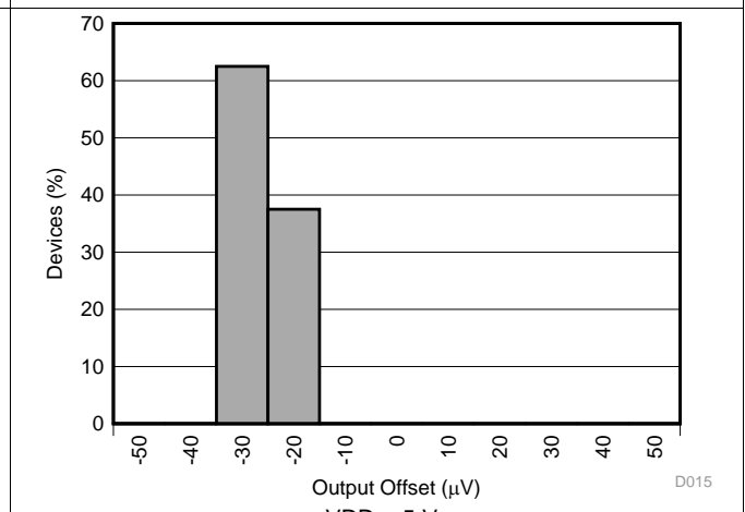
Figure 18. Shunt-Sense Amplifier Output Offset Histogram
