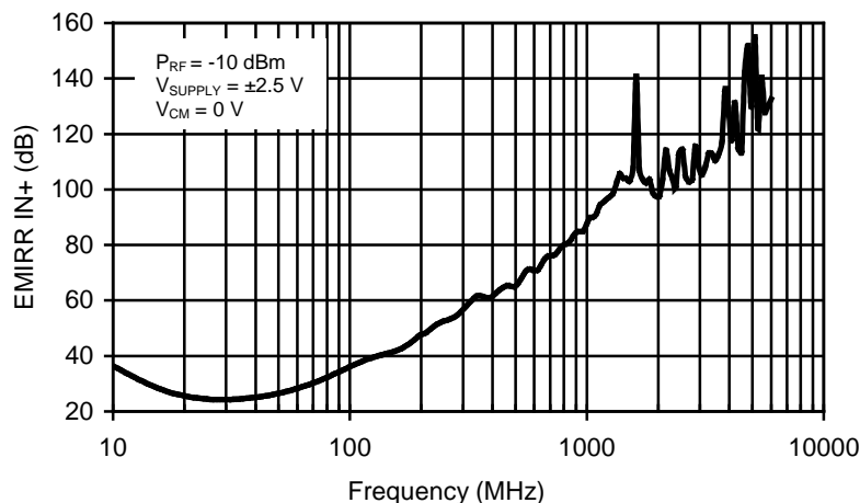
Figure 1. OPA335 EMIRR IN+ vs Frequency
