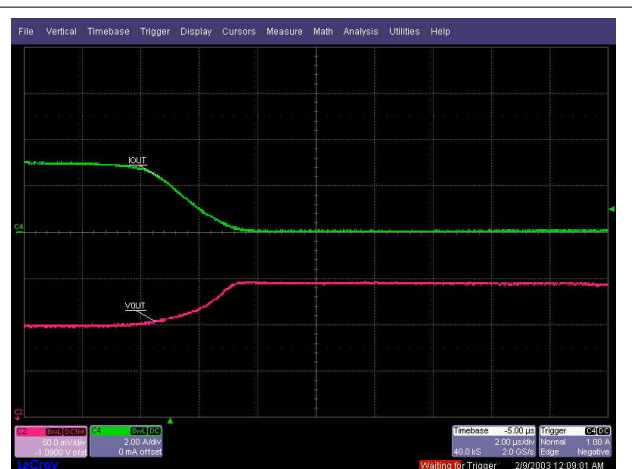
Figure 2-4. TPS7A53EVM-080 Load Transient Results: 3-A to 1-mA Load Step
