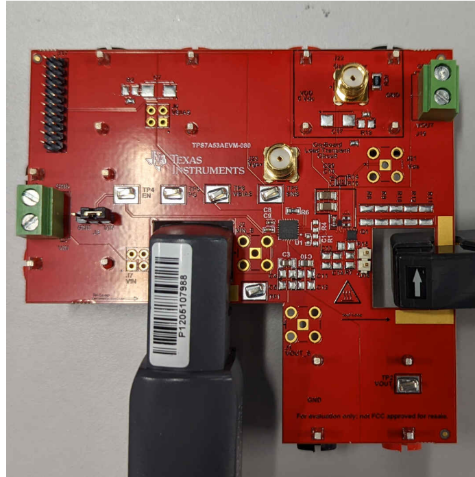
Figure 2-2. TPS7A53EVM-080 With Current Probes Attached
