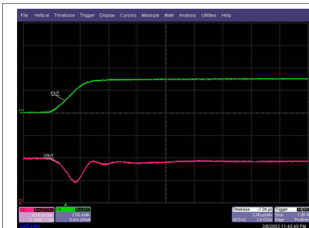
Figure 2-3. TPS7A53EVM-080 Load Transient Results: 1-mA to 3-A Load Step
