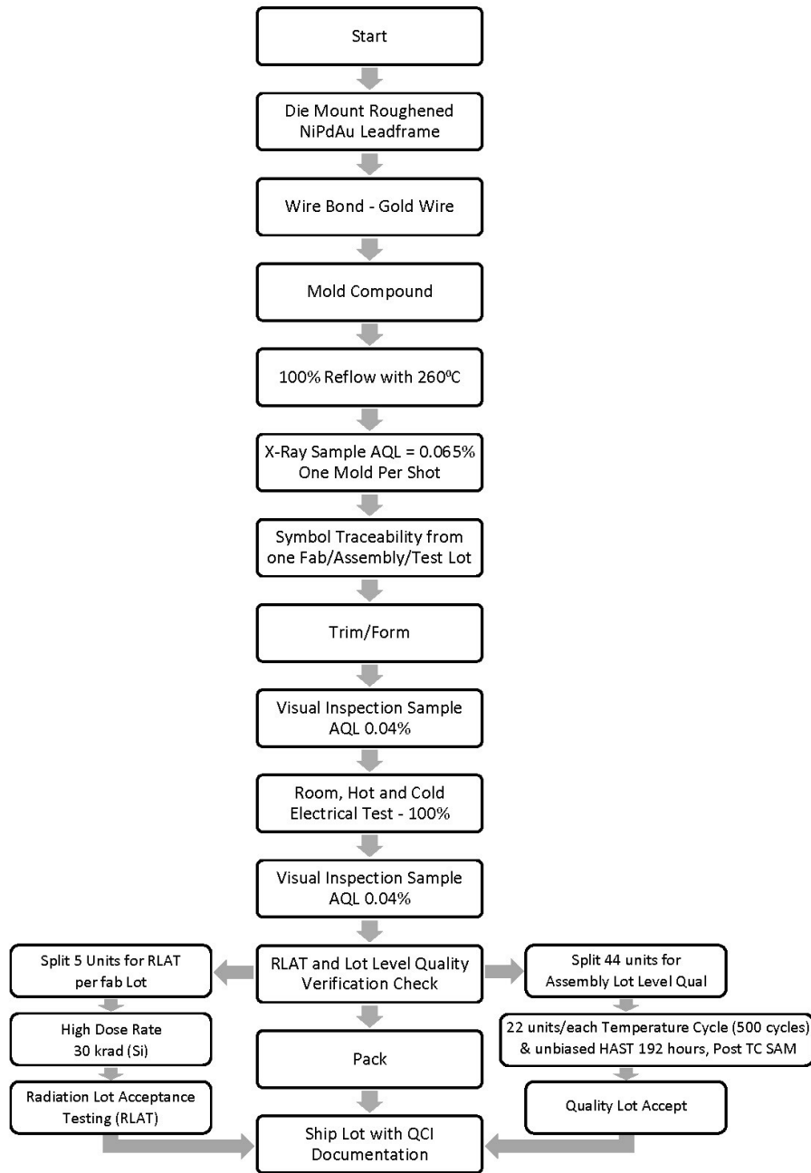
Figure 2-1. TMUX582F-SEP Space Enhanced Plastic Production Flow Chart
