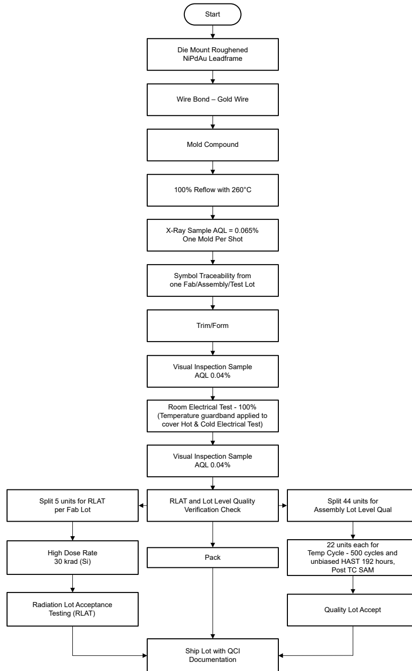
Figure 2-1. SN54SC8T139-SEP Space Enhanced Plastic Production Flow Chart
