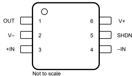
Figure 4-3. Pin Diagram (SOT-23 (DBV) - 6 Package)
