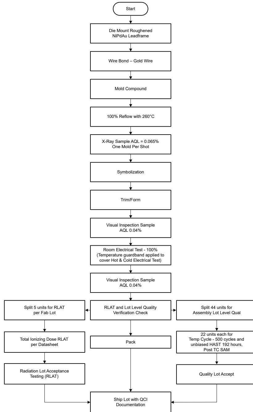
Figure 1-1. TMUX182-SEP Space Enhanced Plastic Production Flow Chart
