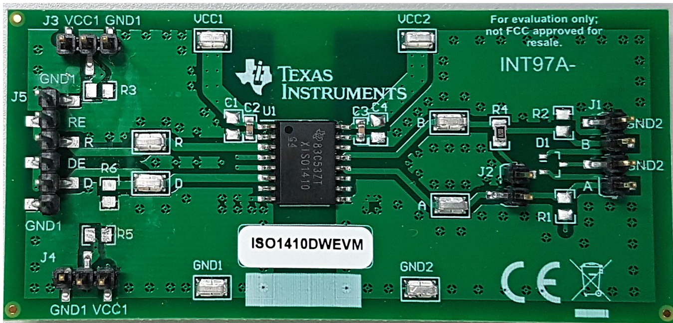
Figure 3. Board Layout
