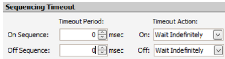
Figure 23. Sequencing Timeout
