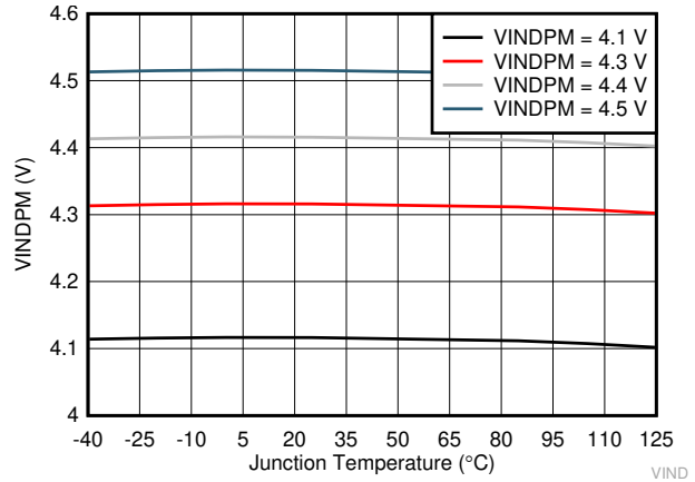
Figure 6-8. VINDPM vs Junction Temperature
