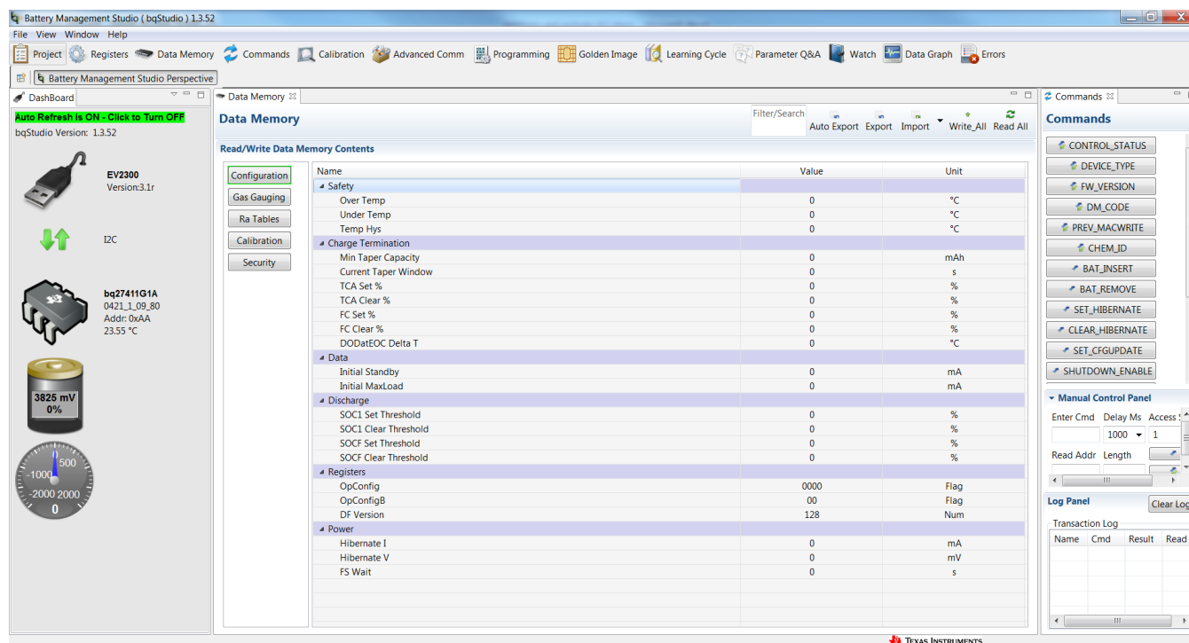
Figure 8. Data Memory Screen
