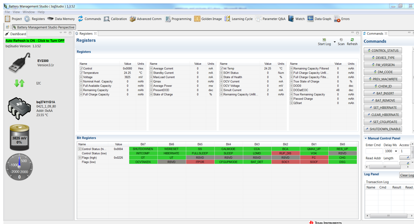
Figure 6. Registers Screen
