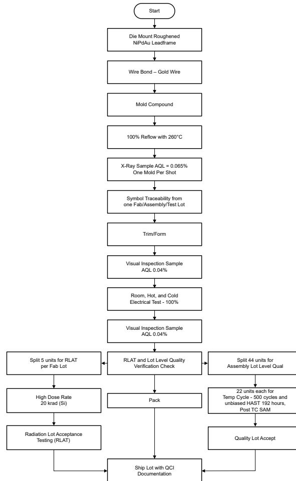
Figure 2-1. TPS7H2140-SEP Space Enhanced Plastic Production Flow Chart
