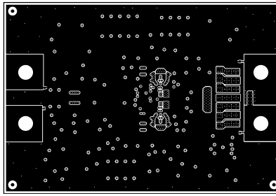
Figure 4-10. Bottom Layer
