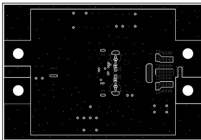
Figure 4-4. Layer 2
