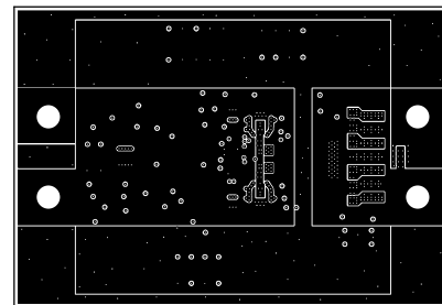
Figure 4-5. Layer 3
