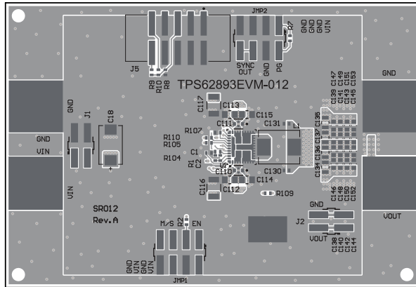
Figure 4-2. Top Layer - Components
