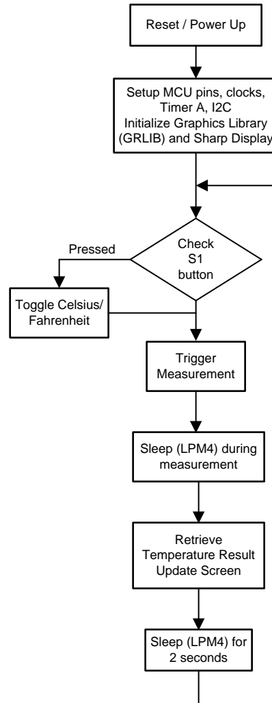
Figure 3. Software Flow Chart
