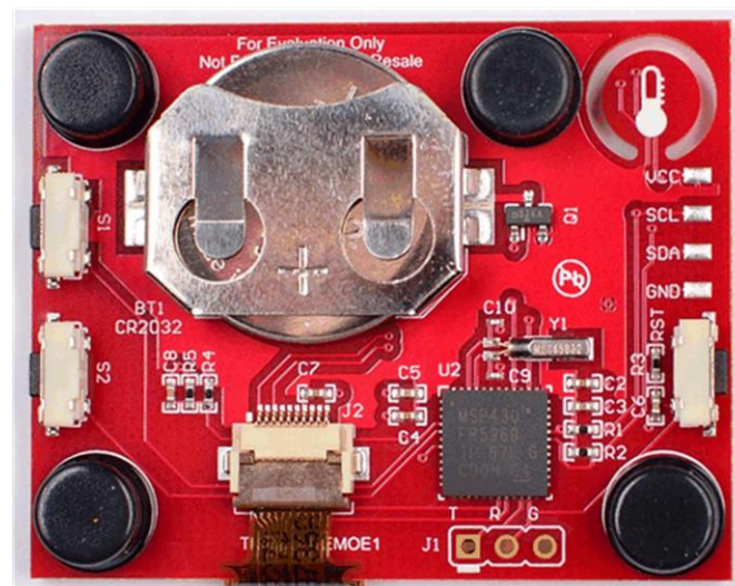
Figure 2. TMP116METER-EVM Back View
