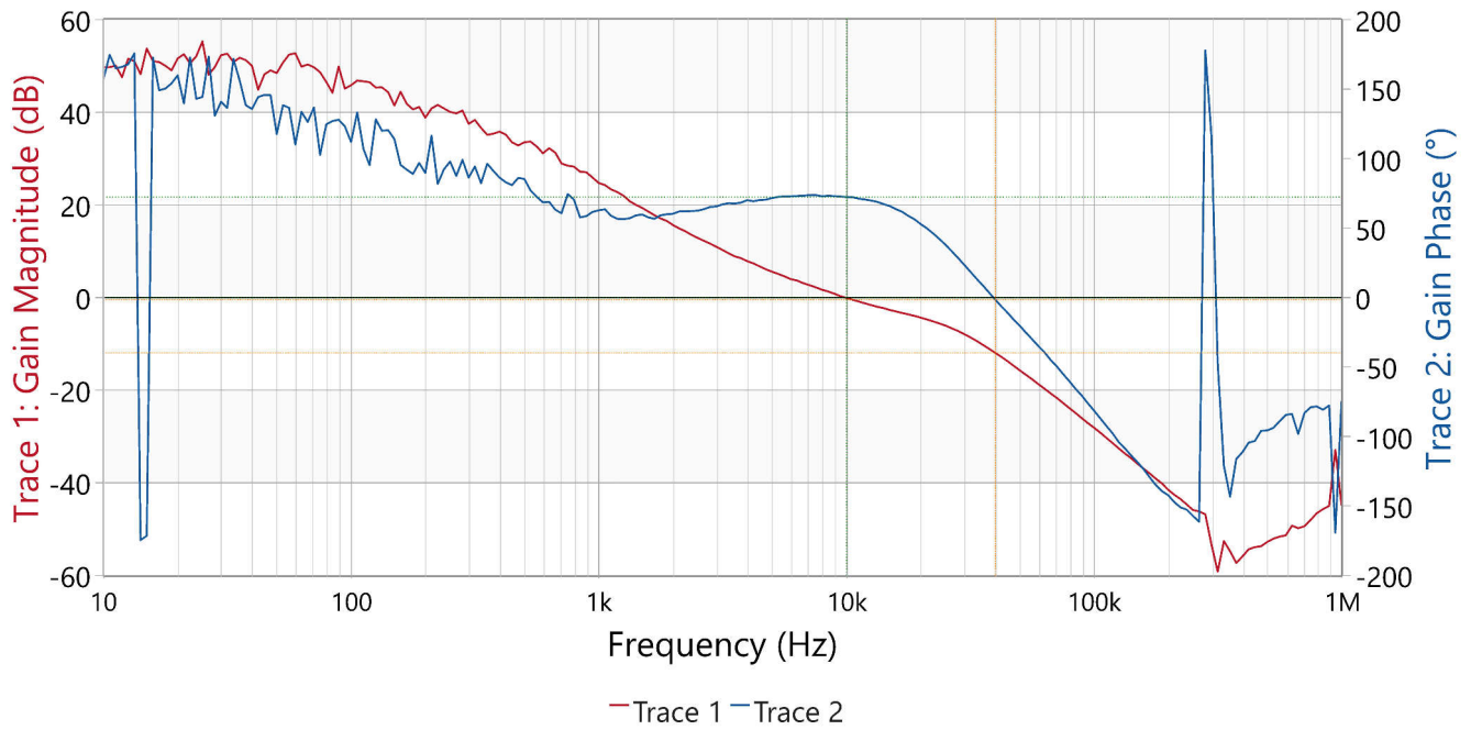
Figure 3-33. Control Loop Response, V_{IN} = 20.0V , V_{OUT} = 20V , I_{OUT} = 5.0A
