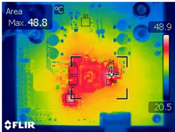
Figure 3-6. Thermal Image: V_{IN} = 20.0V , V_{OUT} = 20.0V , I_{OUT} = 5.0A , No Forced Air Cooling
