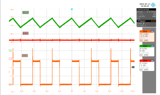
Figure 3-16. SW1, SW2, I_L ( V_{IN} = 12V , V_{OUT} = 28V , I_{OUT} = 5 A )
