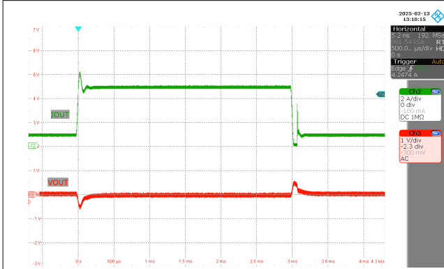
Figure 3-23. Load Step ( V_{IN} = 12\text{ V} , V_{OUT} = 5\text{ V} , I_{OUT} = 1\text{ A} – 5\text{ A} )
