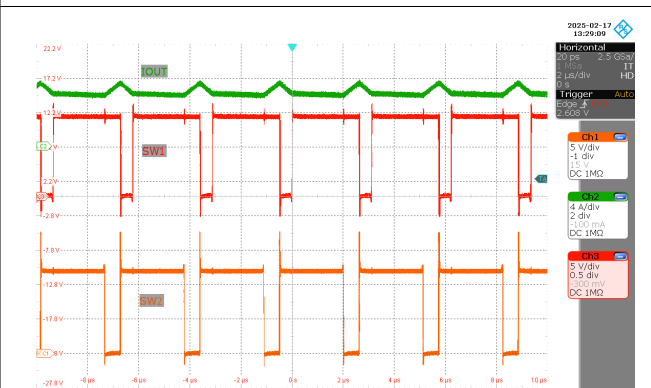
Figure 3-14. SW1, SW2, I_L ( V_{IN} = 12V , V_{OUT} = 12V , I_{OUT} = 5 A )
