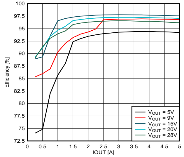
Figure 3-10. Efficiency Versus Output Current at V_{in} = 12V
