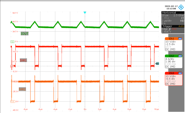
Figure 3-20. SW1, SW2, I_L ( V_{IN} = 20V , V_{OUT} = 20V , I_{OUT} = 5A )
