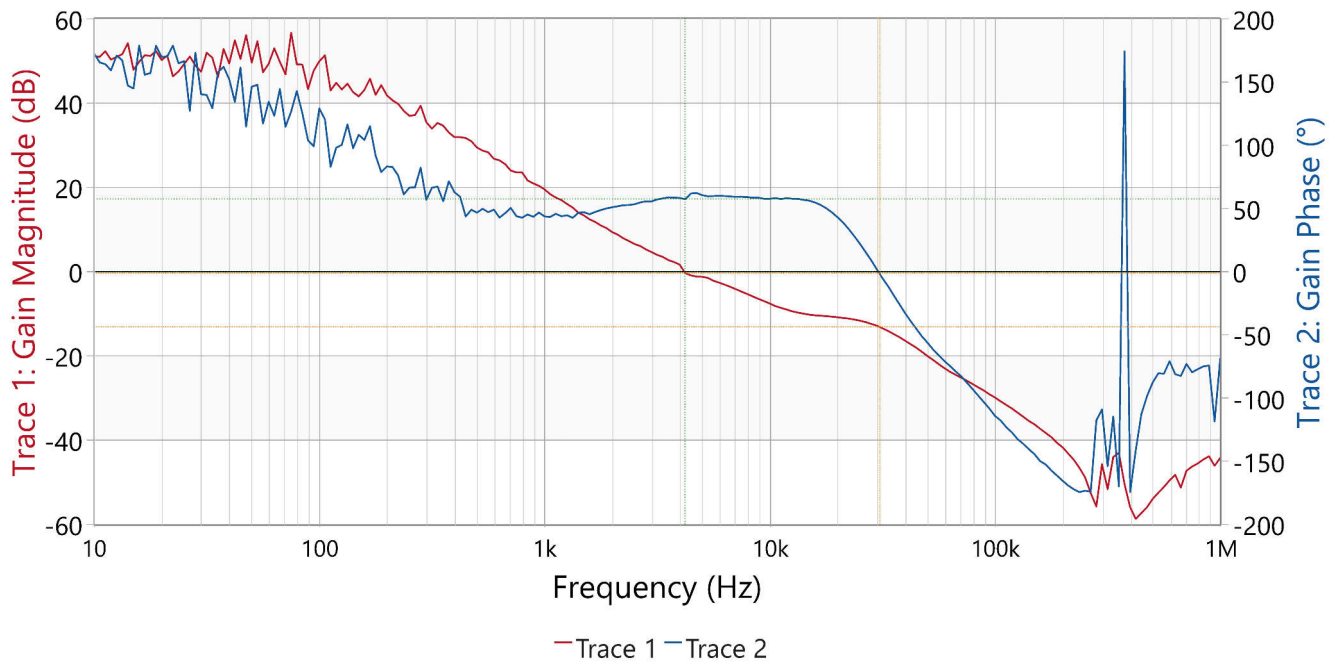
Figure 3-34. Control Loop Response, V_{IN} = 20.0V , V_{OUT} = 48.0V , I_{OUT} = 5.0A
