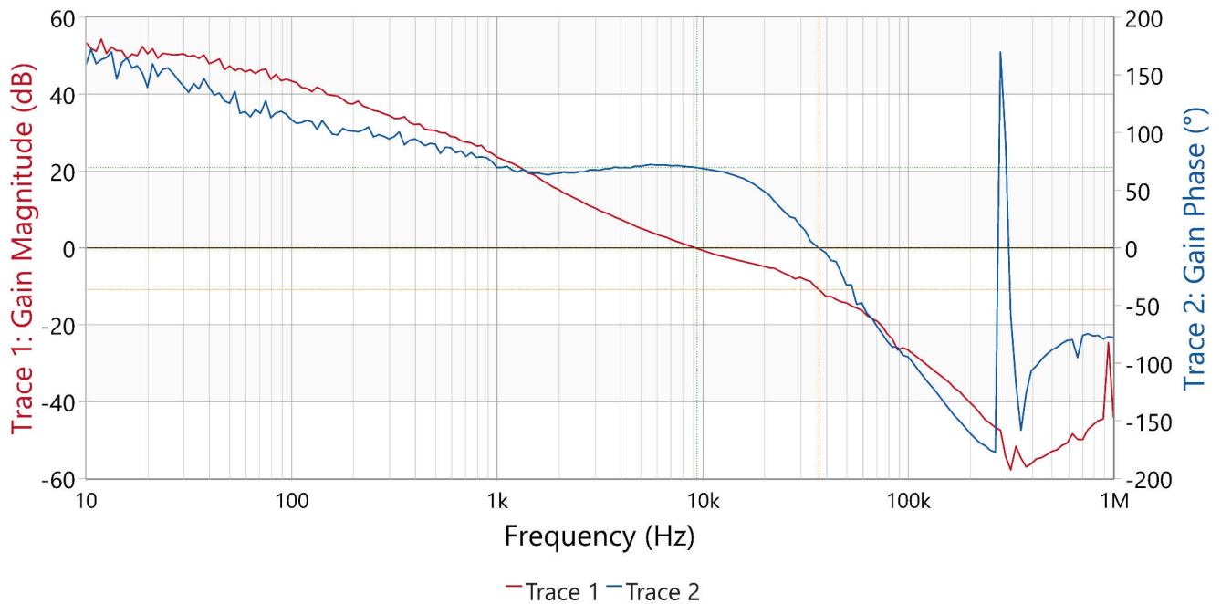
Figure 3-30. Control Loop Response, V_{IN} = 12.0V , V_{OUT} = 12.0V , I_{OUT} = 5.0A
