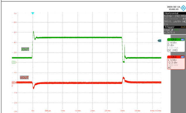
Figure 3-25. Load Step ( V_{IN} = 20\text{ V} , V_{OUT} = 5\text{ V} , I_{OUT} = 1\text{ A} – 5\text{ A} )
