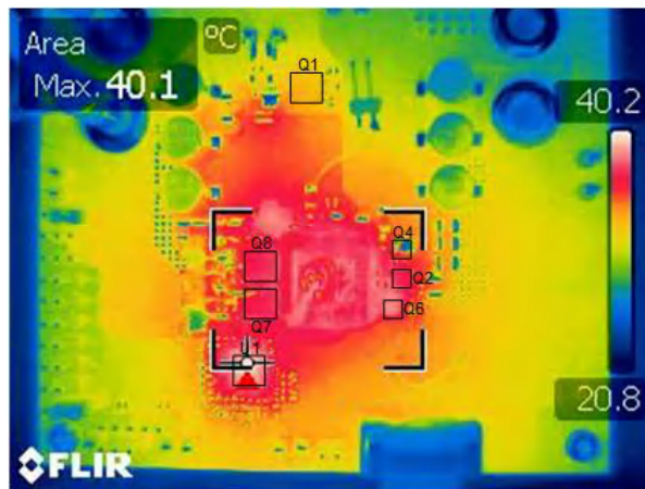
Figure 3-8. Thermal Image: V_{IN} = 20.0V , ILIM (Current Limiter) = 5.0A, Load = Short, No Forced Air Cooling
