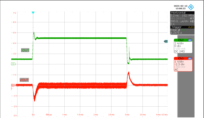
Figure 3-24. Load Step ( V_{IN} = 12\text{ V} , V_{OUT} = 28\text{ V} , I_{OUT} = 1\text{ A} – 5\text{ A} )
