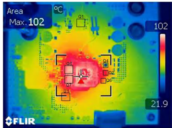
Figure 3-7. Thermal Image: V_{IN} = 20.0V , V_{OUT} = 48.0V , I_{OUT} = 5.0A , No Forced Air Cooling
