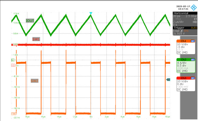
Figure 3-22. SW1, SW2, I_L ( V_{IN} = 20V , V_{OUT} = 48V , I_{OUT} = 5A )
