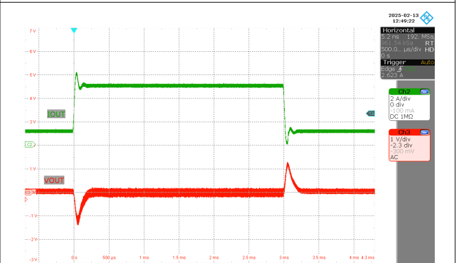
Figure 3-28. Load Step ( V_{IN} = 20\text{ V} , V_{OUT} = 48\text{ V} , I_{OUT} = 1\text{ A} – 5\text{ A} )
