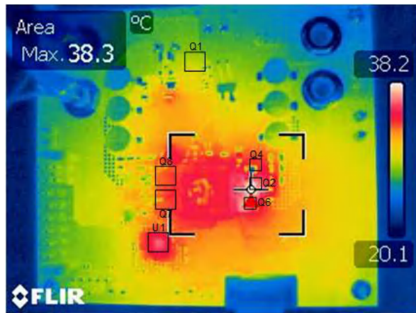
Figure 3-4. Thermal Image: V_{IN} = 20.0V , V_{OUT} = 5.0V , I_{OUT} = 5.0A , No Forced Air Cooling
