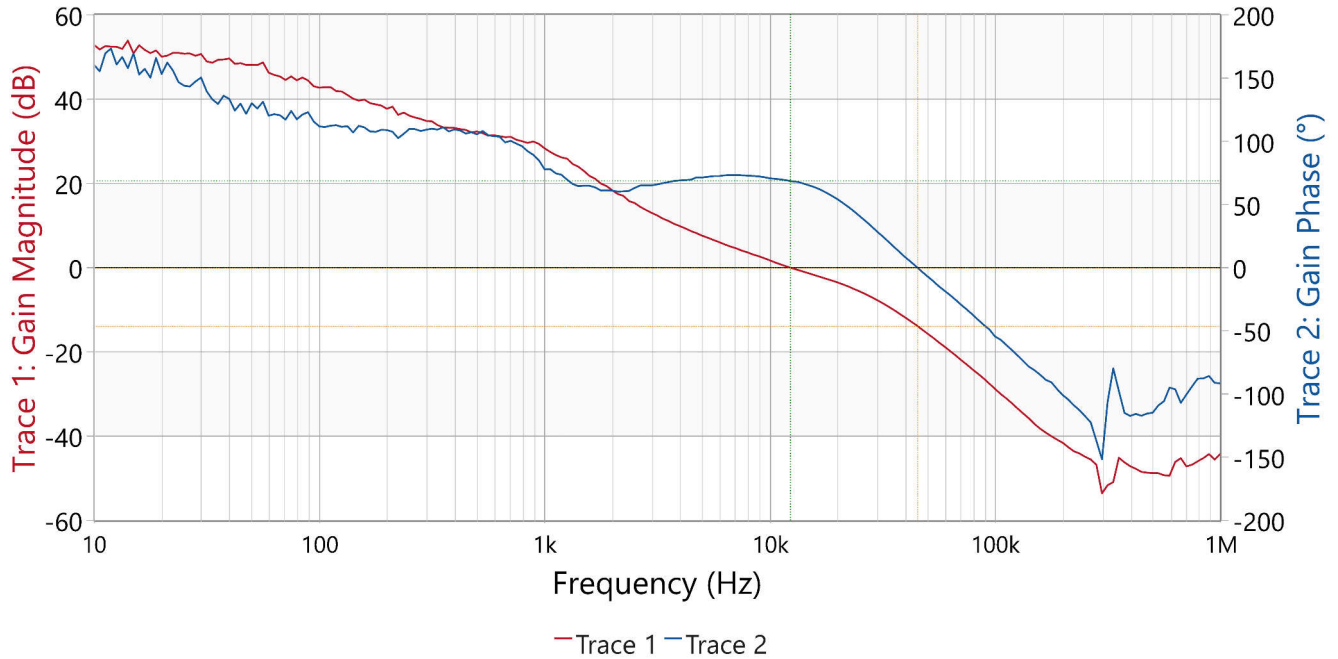
Figure 3-29. Control Loop Response, V_{IN} = 12.0V , V_{OUT} = 5.0V , I_{OUT} = 5.0A
