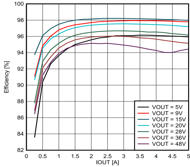
Figure 3-9. Efficiency Versus Output Current at V_{in} = 20V
