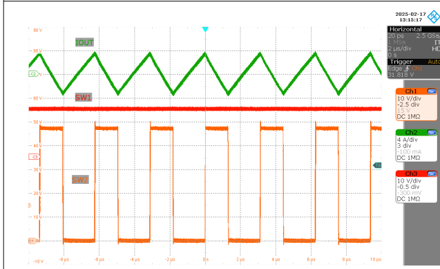
Figure 3-21. SW1, SW2, I_L ( V_{IN} = 20V , V_{OUT} = 48V , I_{OUT} = 0A )
