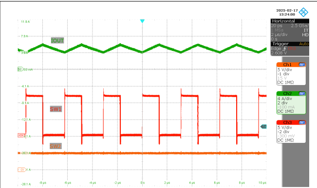
Figure 3-12. SW1, SW2, I_L ( V_{IN} = 12V , V_{OUT} = 5V , I_{OUT} = 5 A )
