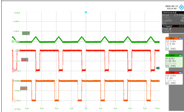
Figure 3-19. SW1, SW2, I_L ( V_{IN} = 20V , V_{OUT} = 20V , I_{OUT} = 0A )
