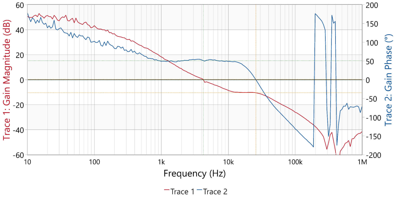
Figure 3-31. Control Loop Response, V_{IN} = 12.0V , V_{OUT} = 28V , I_{OUT} = 5.0A
