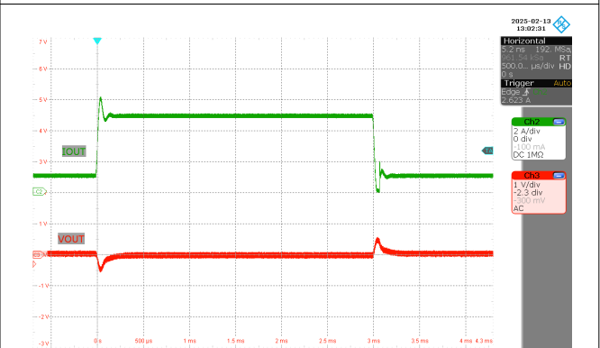
Figure 3-26. Load Step ( V_{IN} = 20\text{ V} , V_{OUT} = 12\text{ V} , I_{OUT} = 1\text{ A} – 5\text{ A} )
