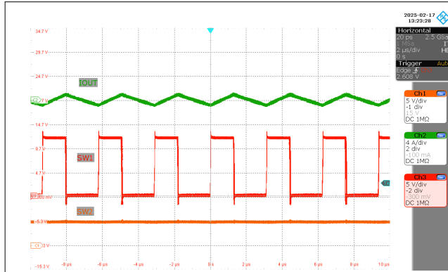
Figure 3-11. SW1, SW2, I_L ( V_{IN} = 12V , V_{OUT} = 5V , I_{OUT} = 0 A )
