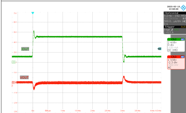
Figure 3-27. Load Step ( V_{IN} = 20\text{ V} , V_{OUT} = 20\text{ V} , I_{OUT} = 1\text{ A} – 5\text{ A} )
