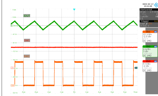
Figure 3-15. SW1, SW2, I_L ( V_{IN} = 12V , V_{OUT} = 28V , I_{OUT} = 0 A )
