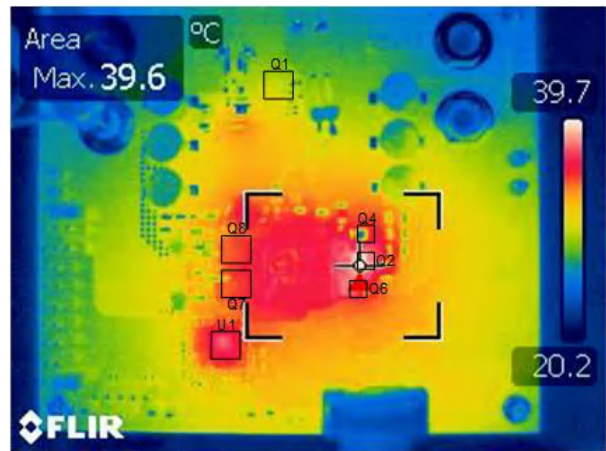
Figure 3-5. Thermal Image: V_{IN} = 20.0V , V_{OUT} = 12.0V , I_{OUT} = 5.0A , No Forced Air Cooling
