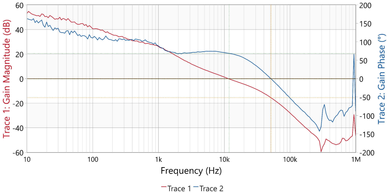
Figure 3-32. Control Loop Response, V_{IN} = 20.0V , V_{OUT} = 5.0V , I_{OUT} = 5.0A
