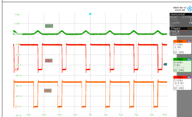
Figure 3-13. SW1, SW2, I_L ( V_{IN} = 12V , V_{OUT} = 12V , I_{OUT} = 0 A )
