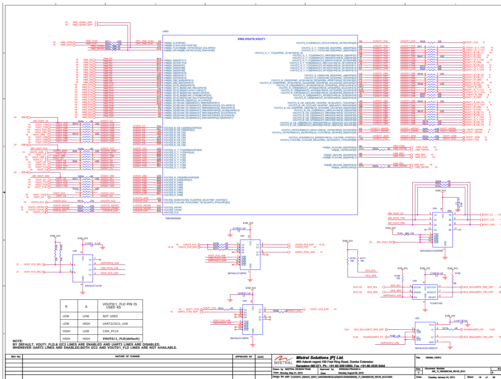
Figure A-17. DM385 VIN0, VOUT0, and VOUT1
