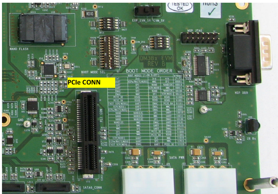
Figure 3-15. PCIe Connector
