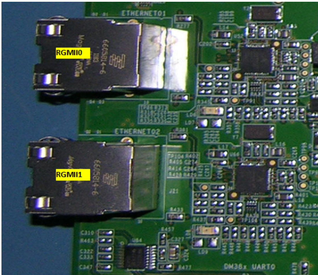
Figure 3-14. Ethernet Connectors
