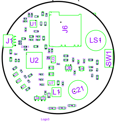
View from Top side (Scale 1:1)
