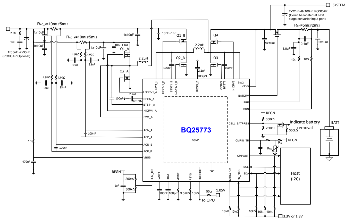
Figure 8-1. Application Diagram of BQ25773
