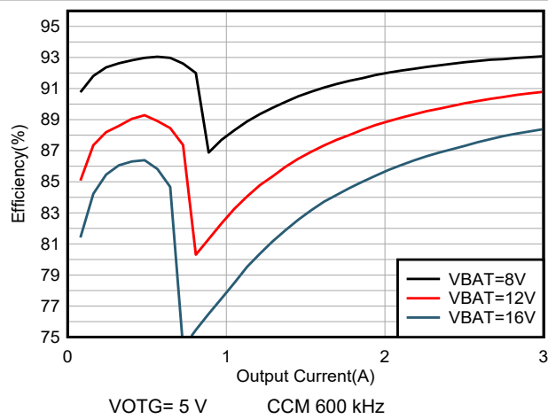
Figure 6-11. OTG Efficiency
