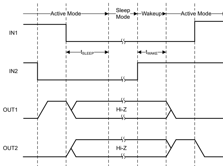
Figure 8-13. Sleep Mode Entry and Wakeup Timing Diagram
