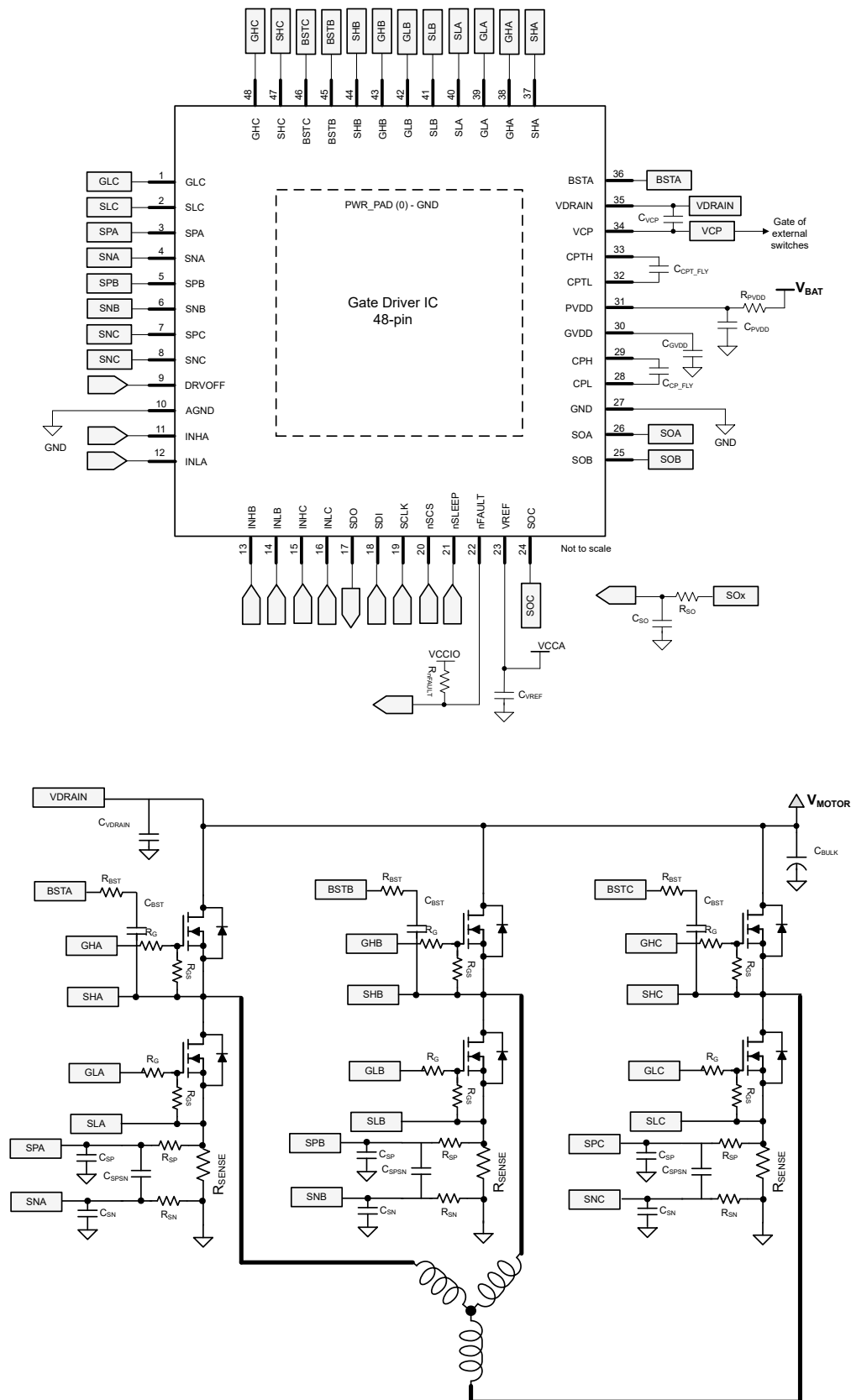
Figure 8-1. DRV8334 Typical Application Schematic
