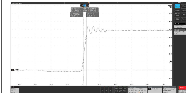
Figure 8-5. SW Node Behavior Showing the Rise Time for a Buck Converter with HB-HS supplied externally and R_{BST}=1.3 \Omega
