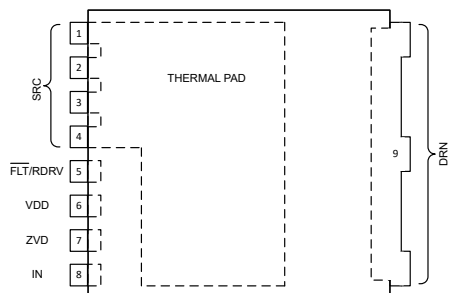
Figure 4-3. LMG3656R035, TOLL Package (Top View)
