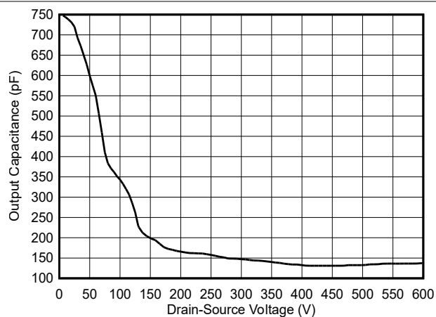
Figure 5-4. Output Capacitance vs Drain-Source Voltage
