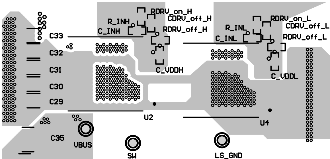
Figure 8-13. LMG3650R035 Half-Bridge Mid-Layer Layout
