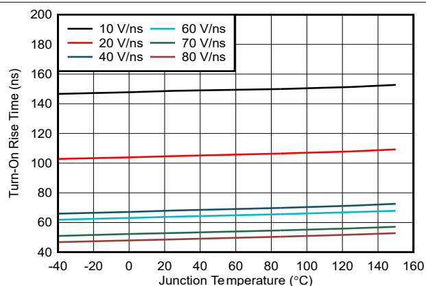
Figure 5-6. Turn-On Rise Time vs Junction Temperature
