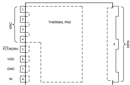
Figure 4-1. LMG3650R035, TOLL Package (Top View)
