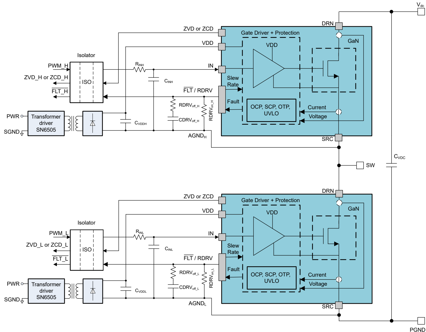
Figure 8-3. LMG3656R035 or LMG3657R035 Typical Half-Bridge Application With Isolated Power Supply
