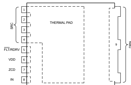
Figure 4-4. LMG3657R035, TOLL Package (Top View)
