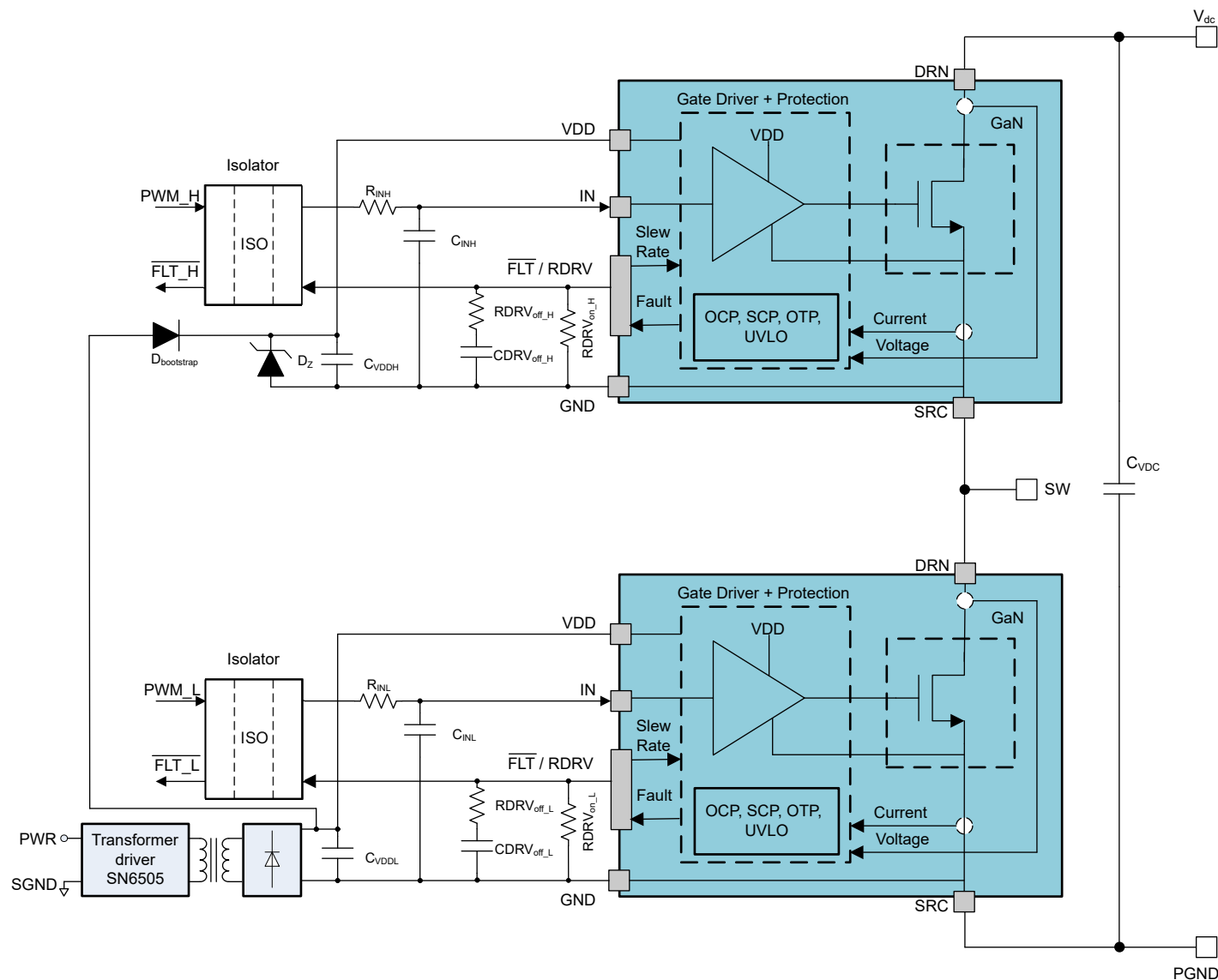
Figure 8-4. LMG3650R035 Typical Half-Bridge Application With Bootstrap
