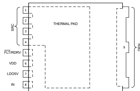
Figure 4-2. LMG3651R035, TOLL Package (Top View)
