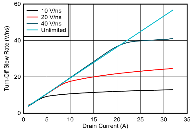
Figure 5-8. Turn-Off Slew Rate vs Drain Current
