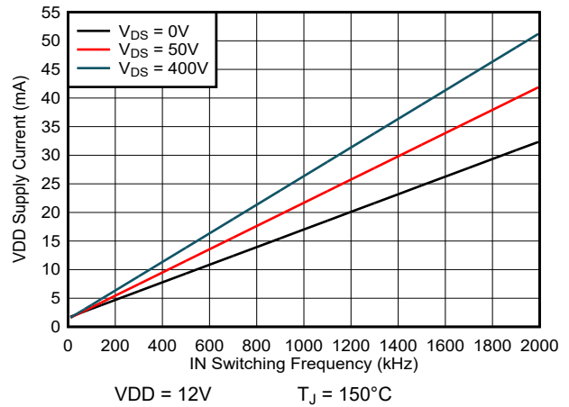
Figure 5-10. VDD Supply Current vs IN Switching Frequency
