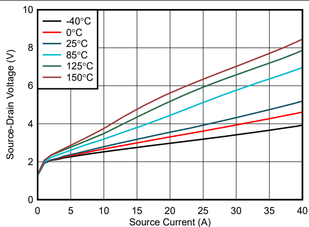
Figure 5-2. Off-State Source-Drain Voltage vs Source Current
