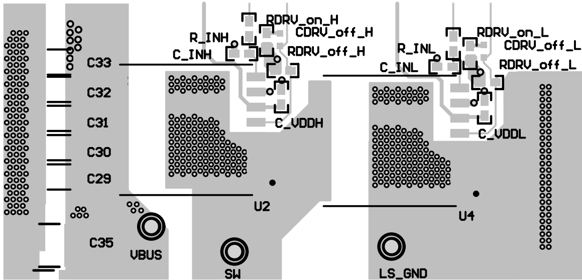
Figure 8-12. LMG3650R035 Half-Bridge Top-Layer Layout
