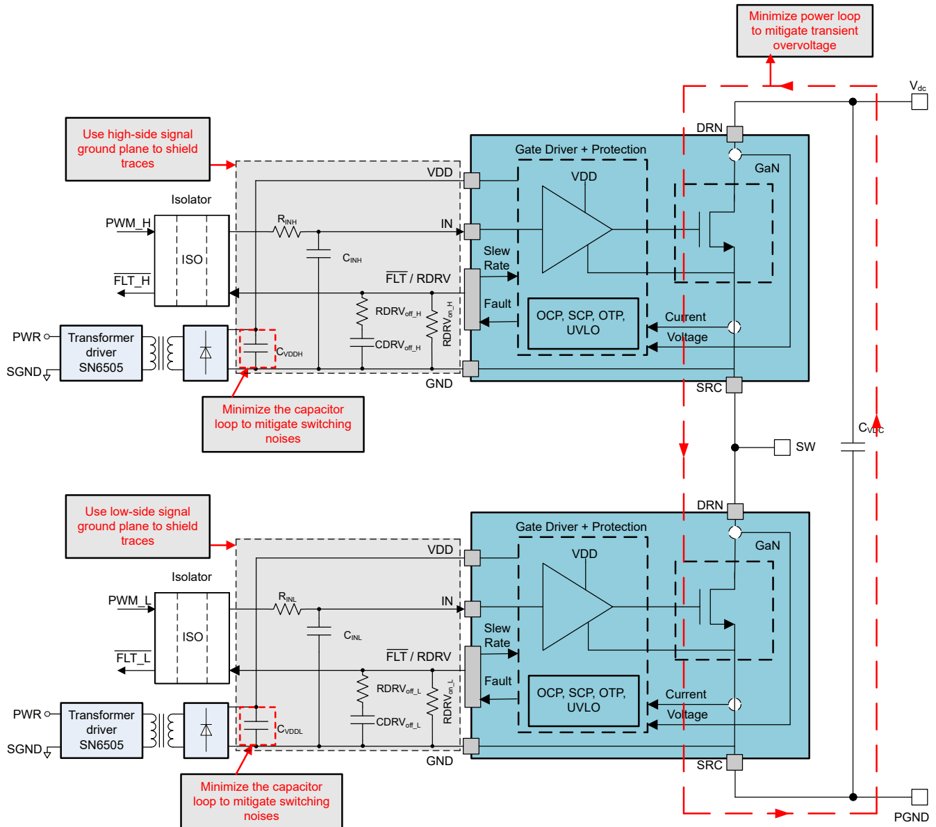
Figure 8-9. LMG3650R035 Typical Schematic With Layout Considerations
