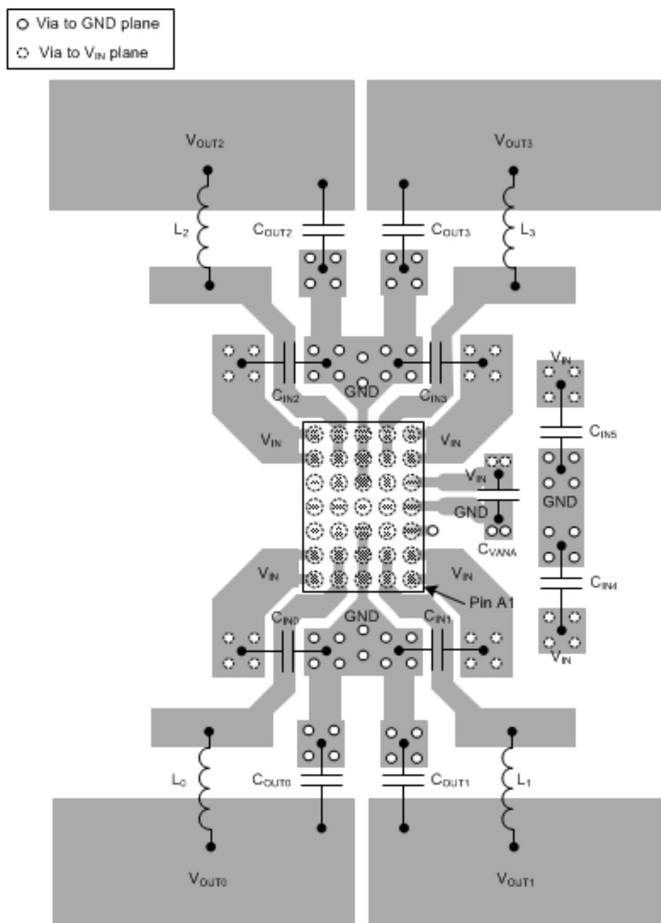
Figure 8-26. LP8758-EA Board Layout
