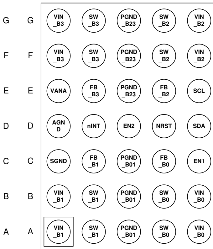
Figure 5-2. YFF Package 35-Pin DSBGA Bottom View
