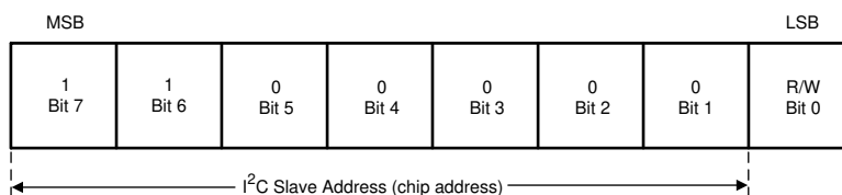
Figure 7-13. Device Address
