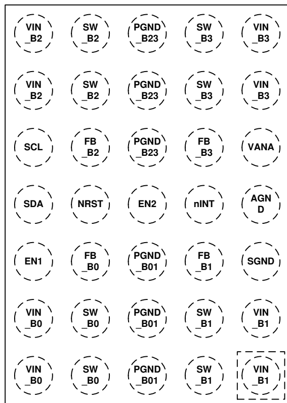
Figure 5-1. YFF Package 35-Pin DSBGA Top View
