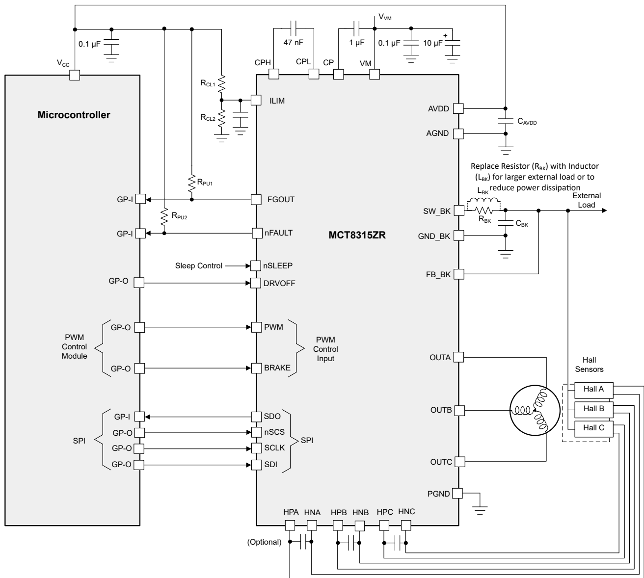
Figure 9-2. Primary Application Schematics for MCT8315ZR (SPI variant)
