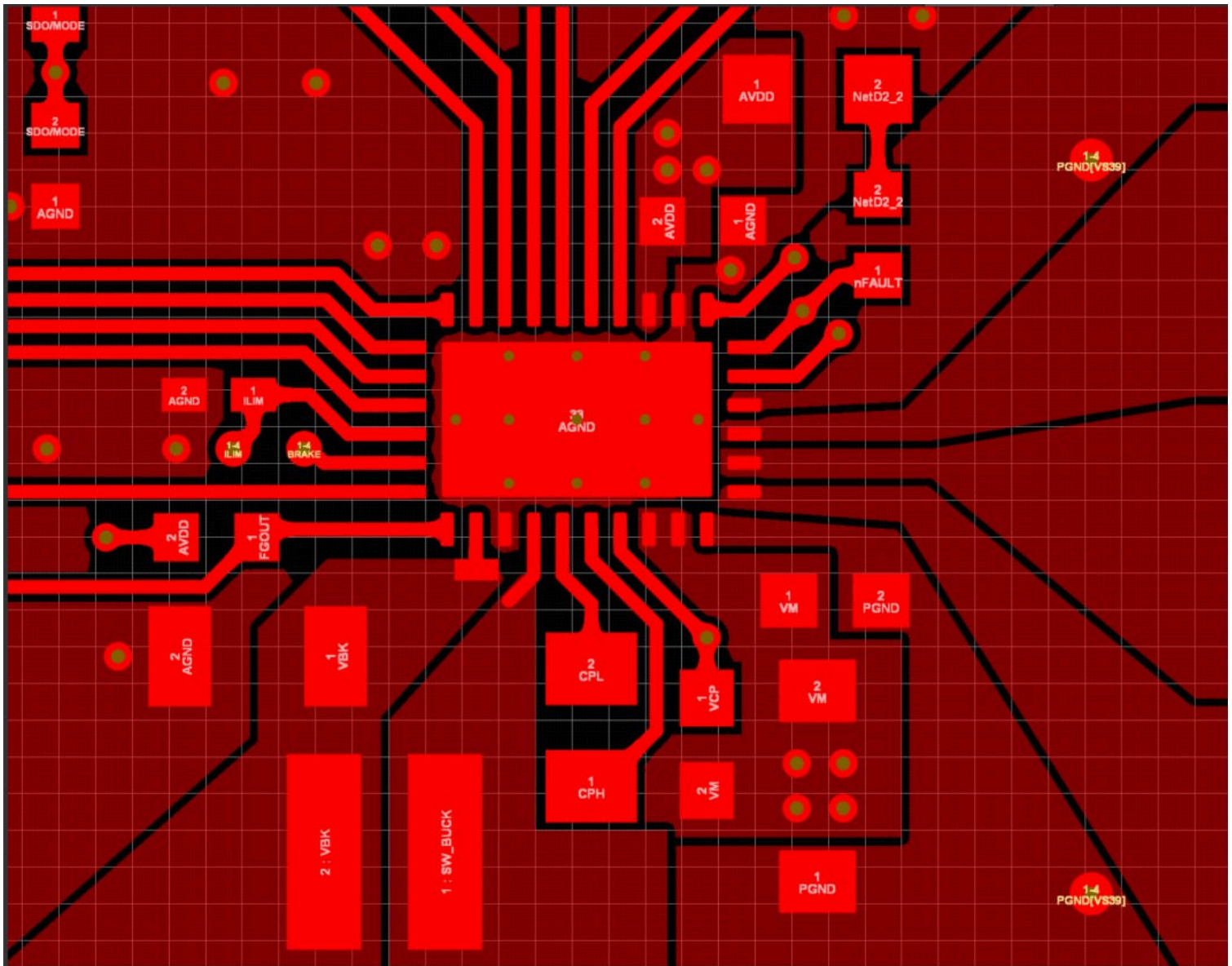
Figure 11-1. Recommended Layout Example for MCT8315Z
