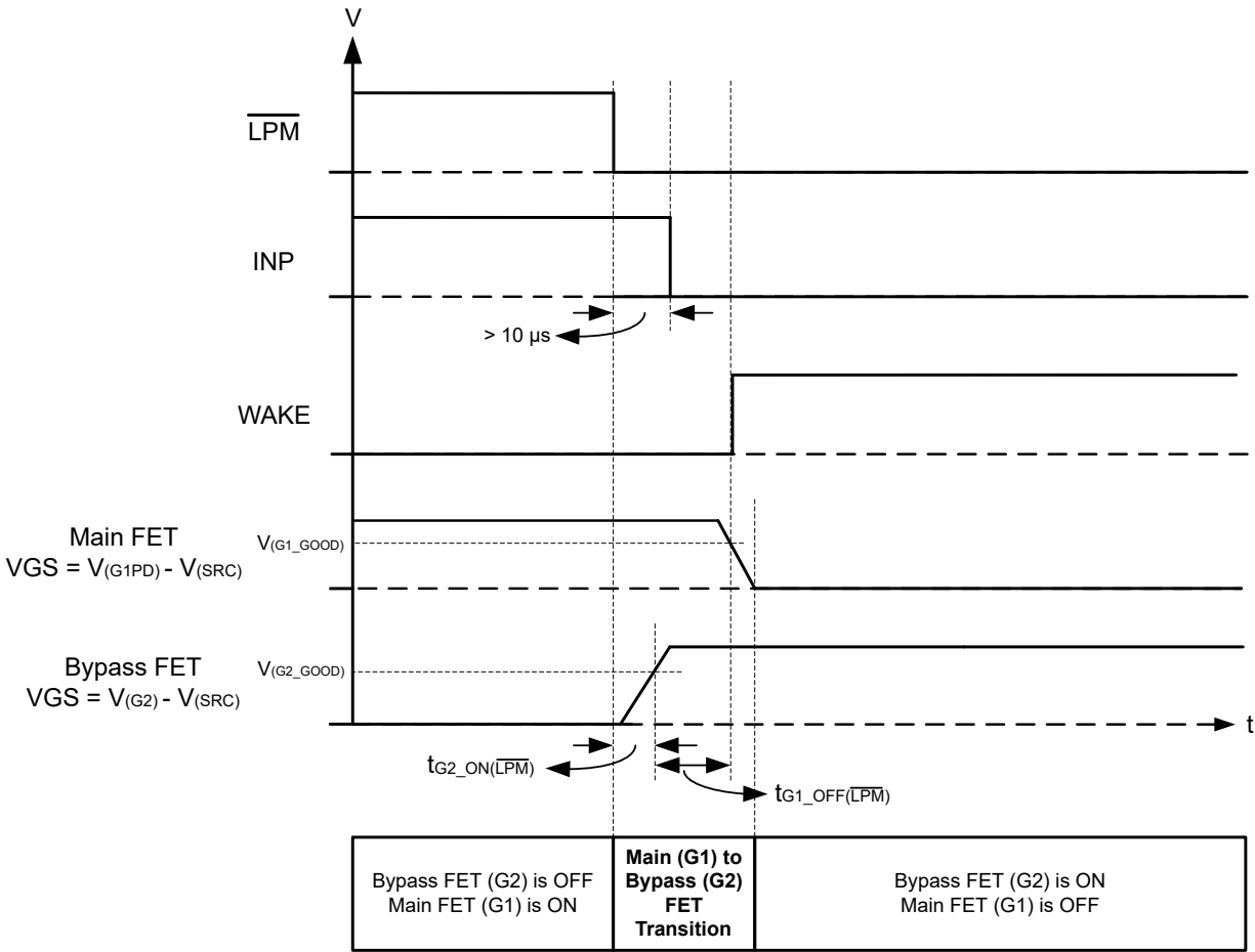
Figure 7-15. \overline{LPM} and INP Signal Sequencing Consideration to Enter Into Low Power Mode From Active Mode
