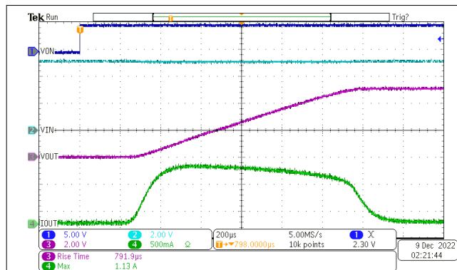
Figure 9-2. Inrush Current for C_L = 220 \text{ } \mu\text{F} with C_T = 1000 \text{ pF}
