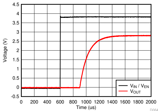
Figure 7-5. Start-Up
