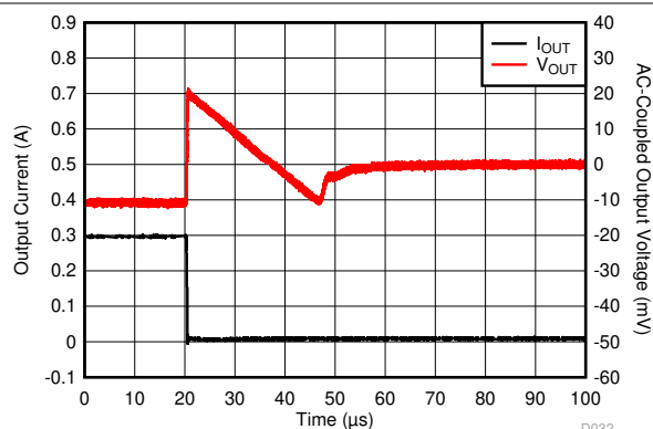
Figure 5-37. Load Transient
