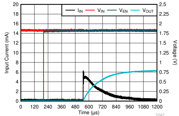
Figure 5-64. Start-Up
