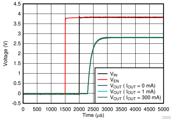
Figure 5-61. Start-Up
