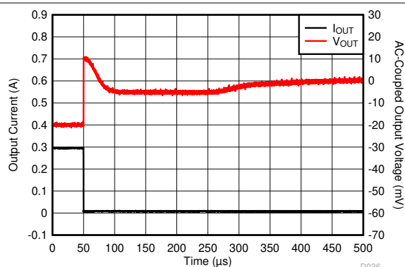
Figure 5-39. Load Transient
