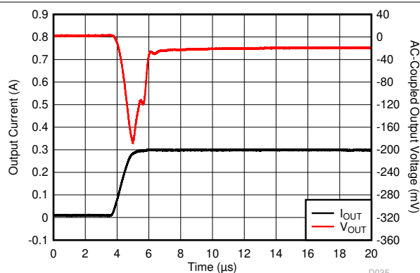
Figure 5-38. Load Transient
