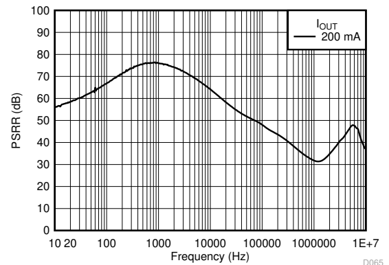
Figure 7-6. PSRR
