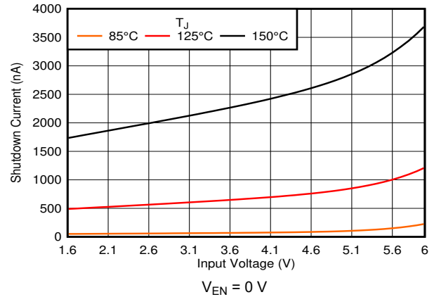
Figure 5-26. Shutdown Current vs V_{IN}
