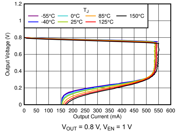
Figure 5-28. Current Limit
