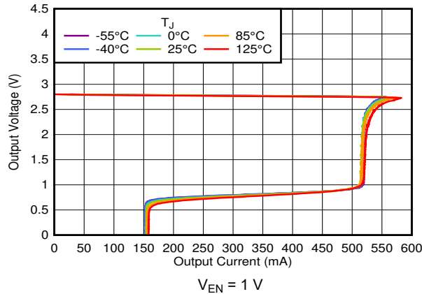
Figure 5-27. Current Limit
