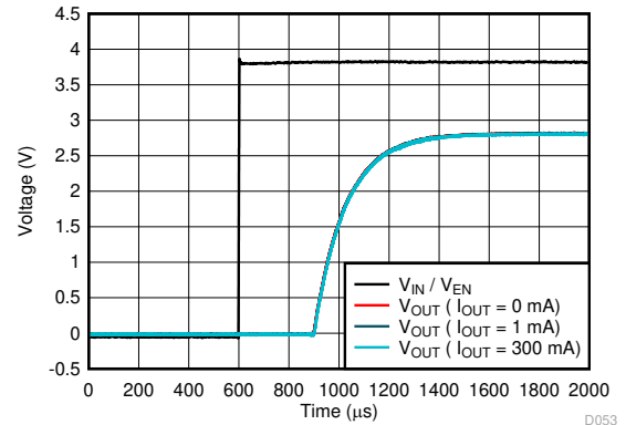
Figure 5-62. Start-Up
