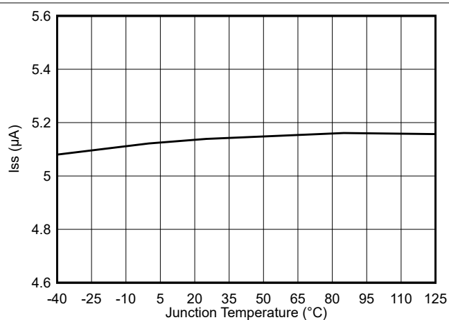
Figure 5-10. Soft-Start Charge Current vs Junction Temperature
