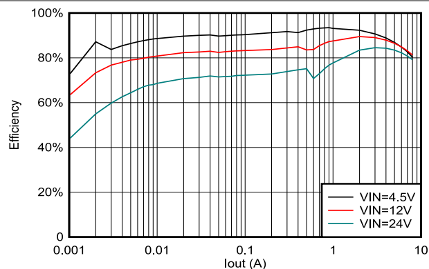
Figure 5-19. TPSM86837 Efficiency, V_{OUT} = 1.8V , F_{sw} = 800kHz
