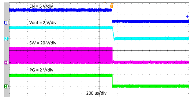
Figure 7-13. Disable Relative to EN
