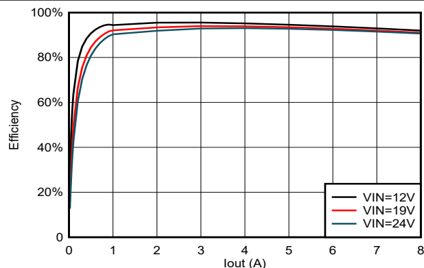
Figure 5-24. TPSM86838 Efficiency, V_{OUT} = 5V , F_{sw} = 800kHz
