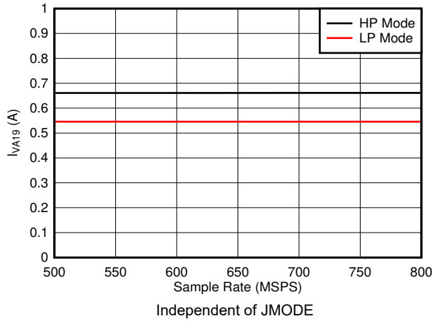
Figure 5-75. Quad Channel, I_{VA19} vs F_S
