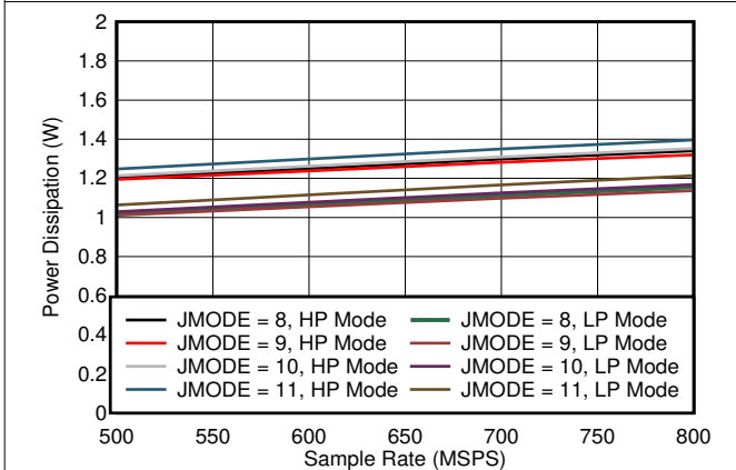
Figure 5-83. Dual Channel, Power Dissipation vs F_S for JMODES 8 - 11
