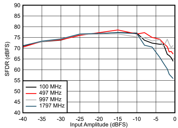
Figure 5-30. SFDR vs Input Amplitude Low Power Mode
