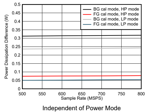
Figure 5-102. Dual Channel, Power Dissipation Change with Calibration Mode
