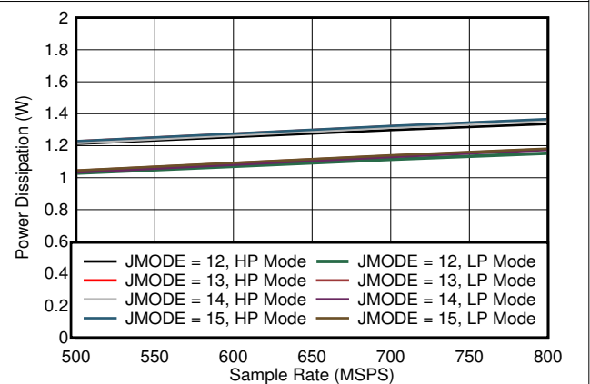
Figure 5-84. Dual Channel, Power Dissipation vs F_S for JMODES 12 - 15
