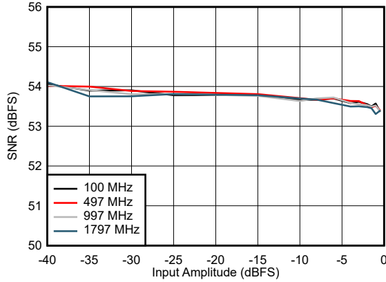
Low Power Mode Figure 5-31. SNR vs Input Amplitude
