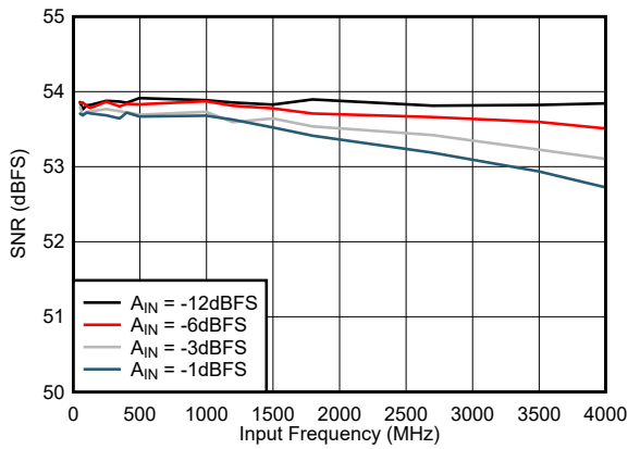
Figure 5-15. SNR vs Input Frequency
