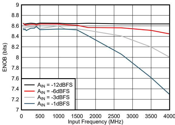
Figure 5-17. ENOB vs Input Frequency
