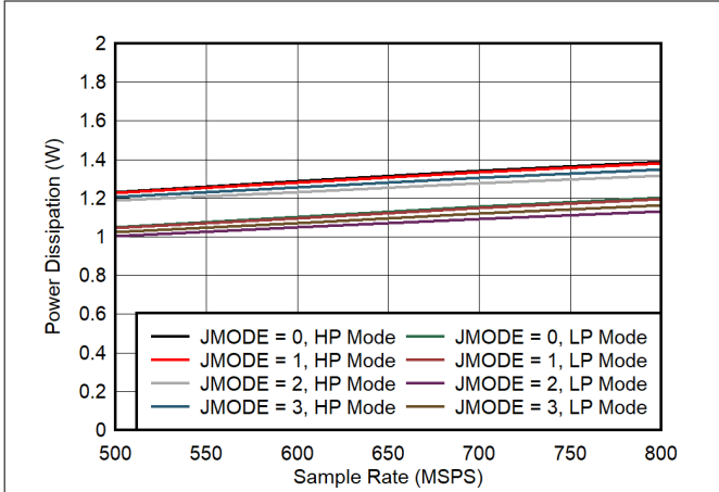
Figure 5-81. Dual Channel, Power Dissipation vs F_S for JMODES 0 - 3
