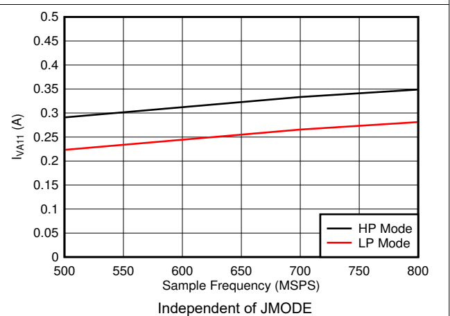
Figure 5-86. Dual Channel, I_{VA11} vs F_S
