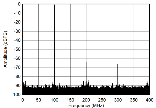
Figure 5-10. Single Tone FFT at 100MHz and -1dBFS Low Power Mode
