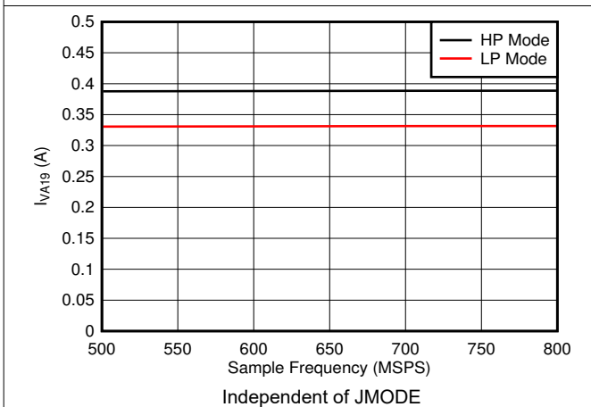
Figure 5-85. Dual Channel, I_{VA19} vs F_S
