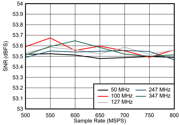
Low Power Mode Figure 5-25. SNR vs Sample Rate
