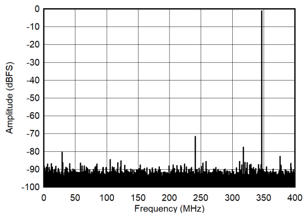
Figure 5-11. Single Tone FFT at 347MHz and -1dBFS
