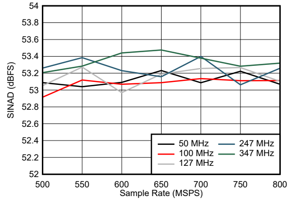
Low Power Mode Figure 5-26. SINAD vs Sample Rate
