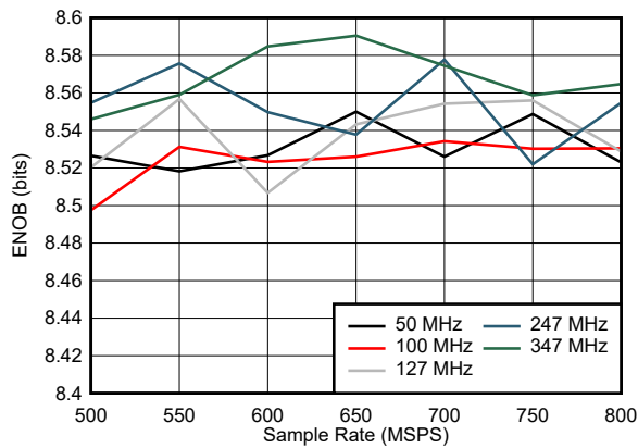
Low Power Mode Figure 5-27. ENOB vs Sample Rate
