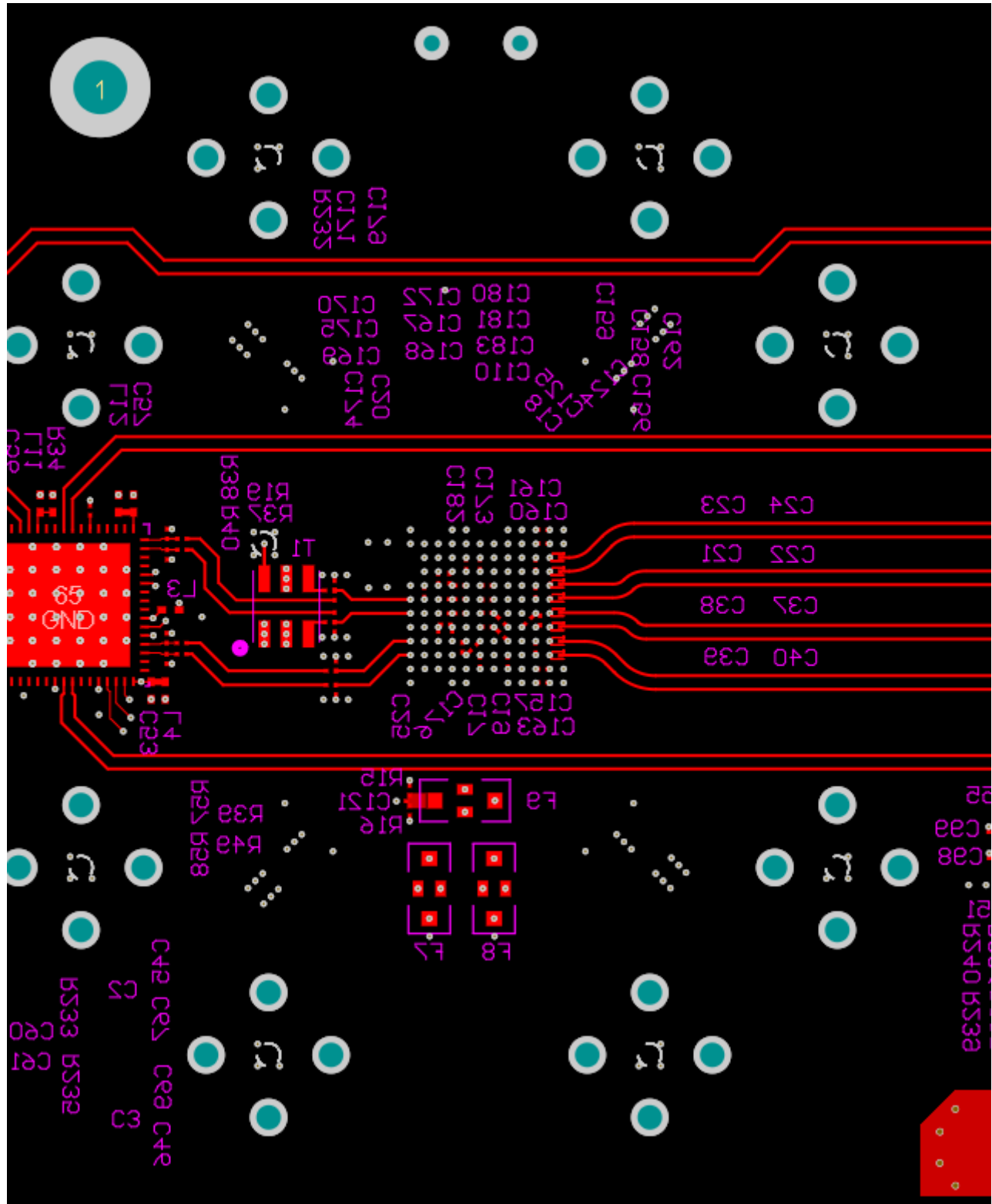
Figure 7-7. Bottom Layer Routing: CLK_{\pm} , SYSREF and D[7:4]_{\pm} Routing
