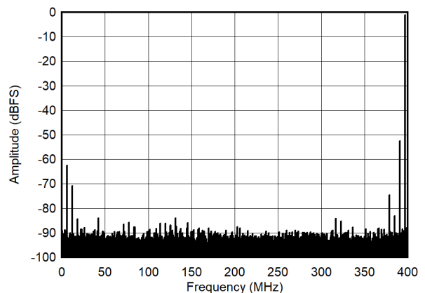
Figure 5-12. Single Tone FFT at 1197MHz and -1dBFS
