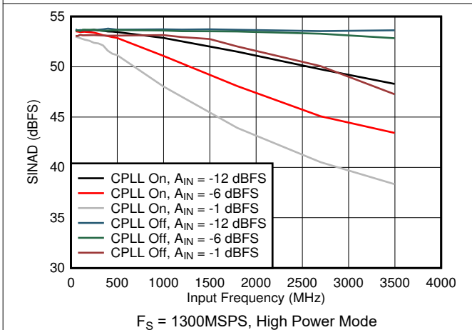
Figure 5-71. SINAD vs Input Frequency, CPLL and Input Amplitude
