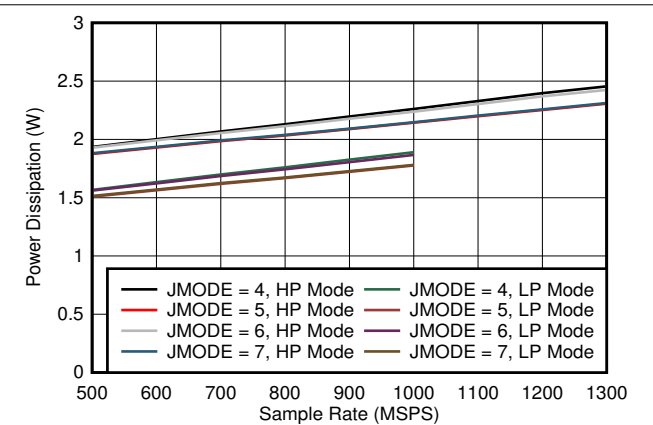
Figure 5-82. Quad Channel, Power Dissipation vs FS for JMODES 4 - 7
