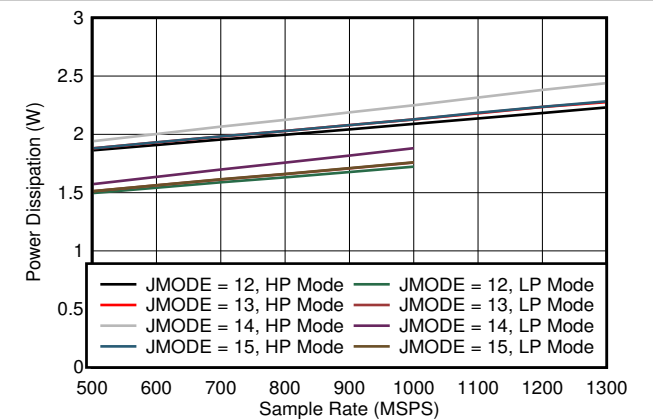
Figure 5-84. Quad Channel, Power Dissipation vs FS for JMODES 12 - 15
