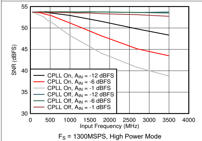
Figure 5-69. SNR vs Input Frequency, CPLL and Input Amplitude
