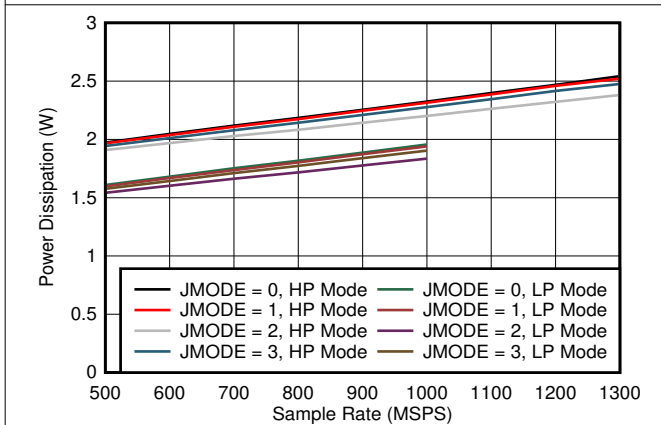
Figure 5-81. Quad Channel, Power Dissipation vs FS for JMODES 0 - 3
