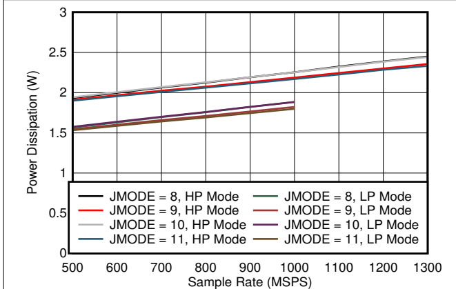
Figure 5-83. Quad Channel, Power Dissipation vs FS for JMODES 8 - 11
