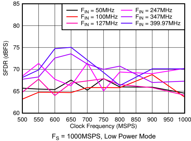
Figure 5-25. SFDR vs Sample Rate
