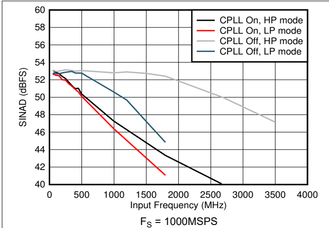
Figure 5-67. SINAD vs Input Frequency and CPLL
