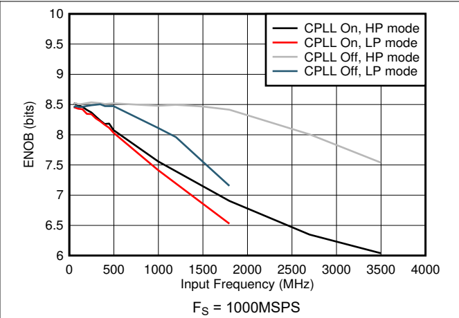
Figure 5-68. ENOB vs Input Frequency and CPLL
