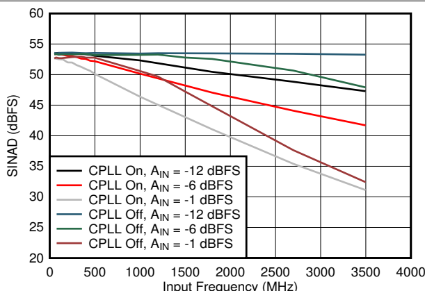
F_S = 1000\text{MSPS} , Low Power Mode
