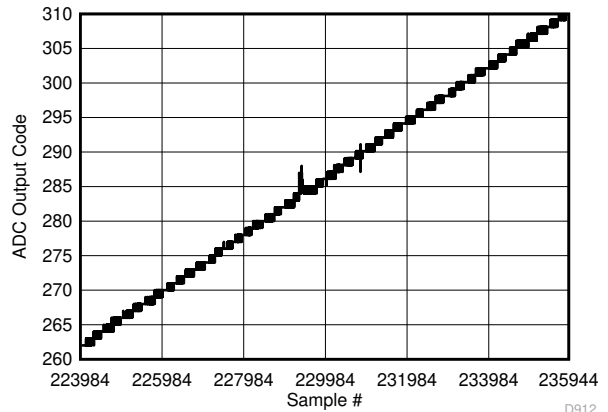
Figure 5-128. Background Calibration Core Transition (AC Signal Zoomed)
