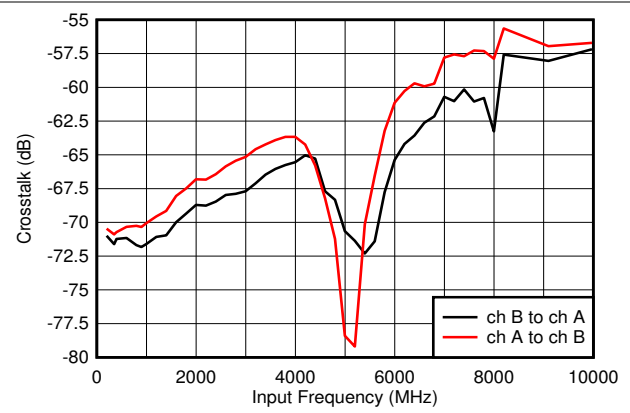
Figure 5-2. Crosstalk vs Input Frequency
