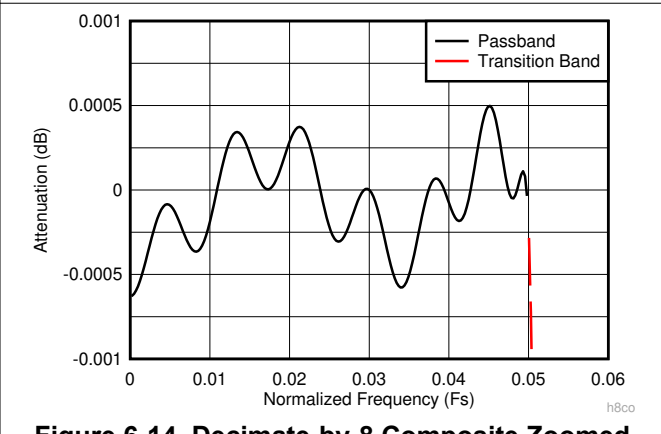
Figure 6-14. Decimate-by-8 Composite Zoomed Pass-Band Response h8co
