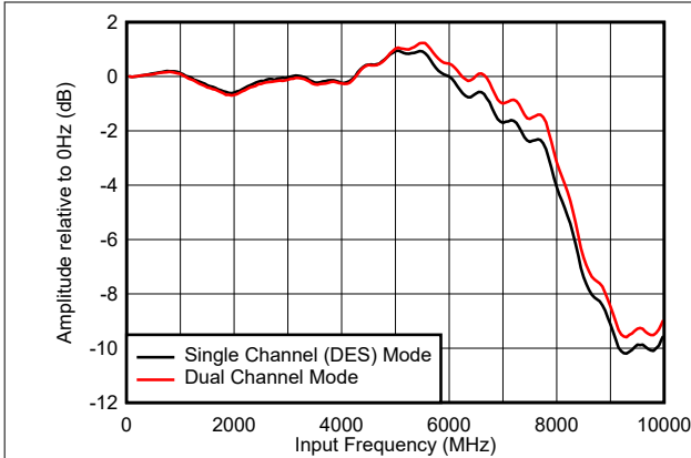
Figure 5-1. Input Amplitude vs Input Frequency
