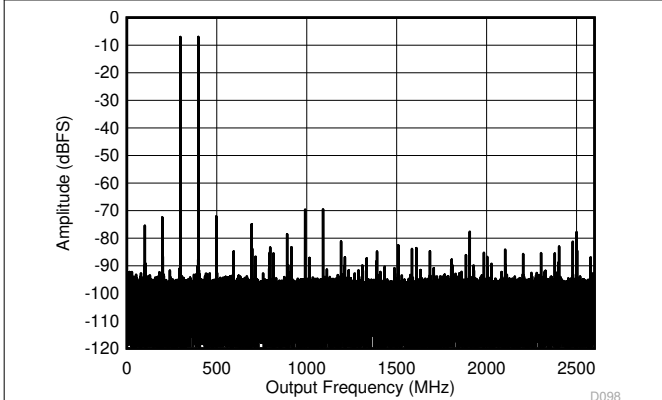
each tone at -7 dBFS, 100 MHz Tone Spacing Figure 5-23. Dual Channel Mode: Two Tone FFT at 347 MHz
