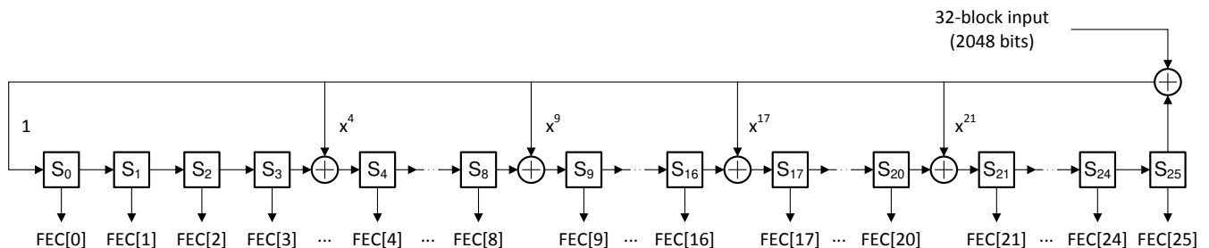
Figure 6-22. FEC Parity Bit Generator
