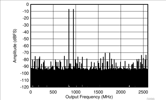
each tone at -7 dBFS, 100 MHz Tone Spacing Figure 5-24. Dual Channel Mode: Two Tone FFT at 897 MHz
