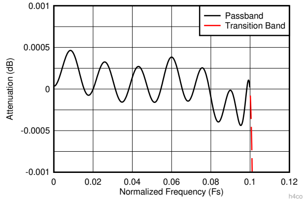
Figure 7-12. Decimate-by-4 Composite Zoomed Pass-Band Response h4co
