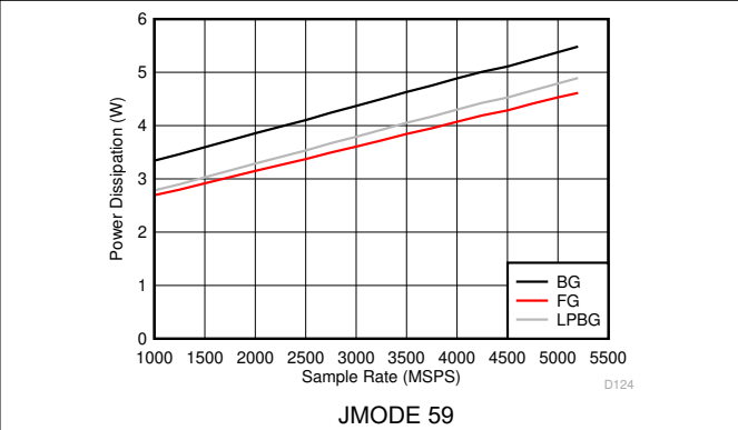
Figure 6-142. Dual Channel Mode: Power Dissipation vs Sample Rate
