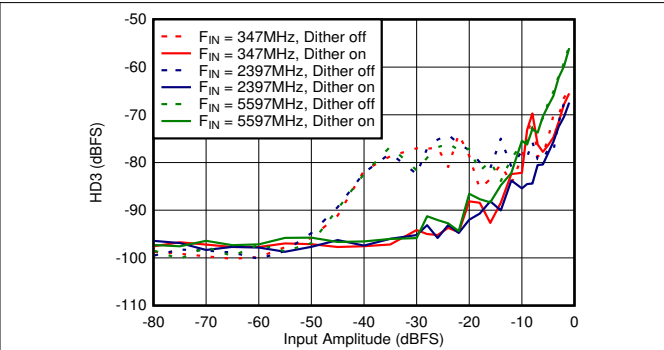
Figure 6-80. Dual Channel Mode: HD3 vs Input Amplitude and Dither
