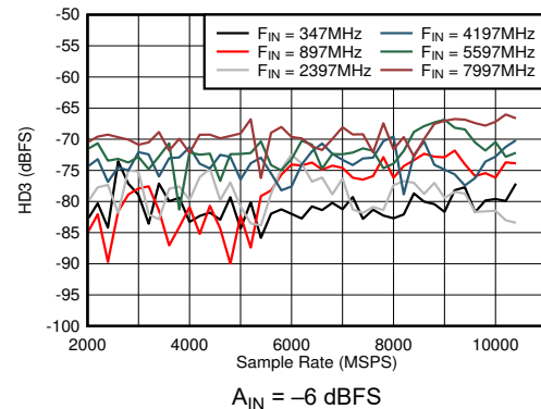
Figure 6-40. DES Mode: HD3 vs Sample Rate and Input Frequency A_{\text{IN}} = -6\text{ dBFS}
