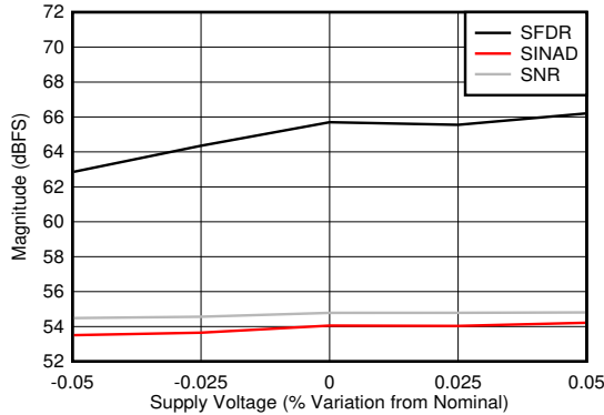
Figure 6-97. Dual Channel Mode: SNR, SINAD and SFDR vs Supply Voltage
