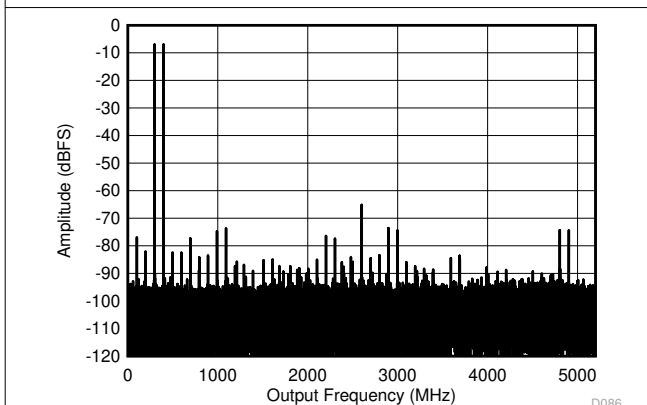
Figure 6-11. DES Mode: Two Tone FFT at 347 MHz
