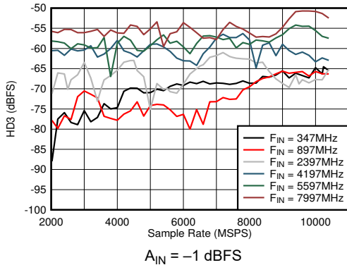
Figure 6-39. DES Mode: HD3 vs Sample Rate and Input Frequency A_{\text{IN}} = -1\text{ dBFS}
