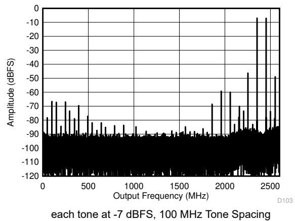
each tone at -7 dBFS, 100 MHz Tone Spacing Figure 6-28. Dual Channel Mode: Two Tone FFT at 7997 MHz
