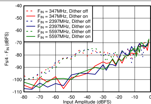
Figure 6-72. DES Mode: F_{s/4} - F_{IN} vs Input Amplitude and Dither
