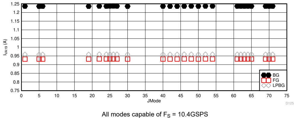
Figure 6-111. DES Mode: I_{VA19} vs JMODE at 10.4GSPS
