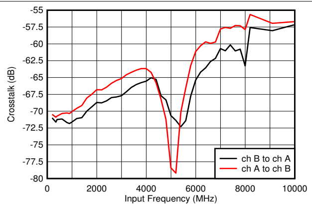
Dual channel mode, JMODE 3 Figure 6-2. Crosstalk vs Input Frequency
