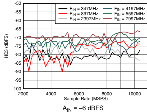
Figure 6-40. DES Mode: HD3 vs Sample Rate and Input Frequency A_{\text{IN}} = -6\text{ dBFS}
