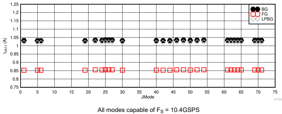
Figure 6-112. DES Mode: I_{VA11} vs JMODE at 10.4GSPS
