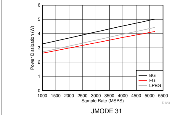
Figure 6-141. Dual Channel Mode: Power Dissipation vs Sample Rate
