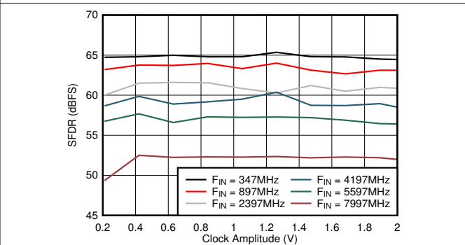
Figure 6-84. DES Mode: SFDR vs Clock Amplitude
