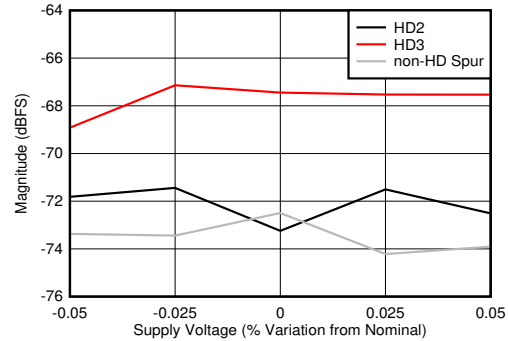
Figure 6-98. Dual Channel Mode: HD2, HD3 and Worst non-HD Spur vs Supply Voltage
