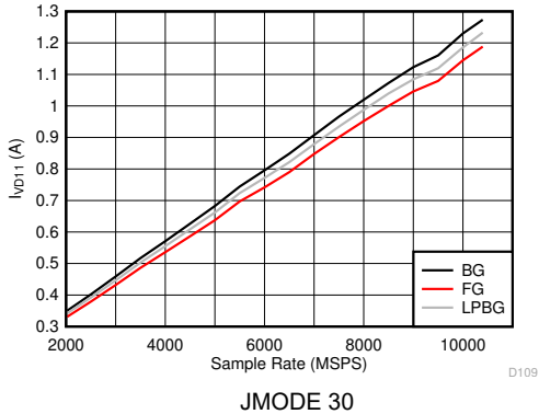
Figure 6-127. DES Mode: I_{VD11} vs Sample Rate
