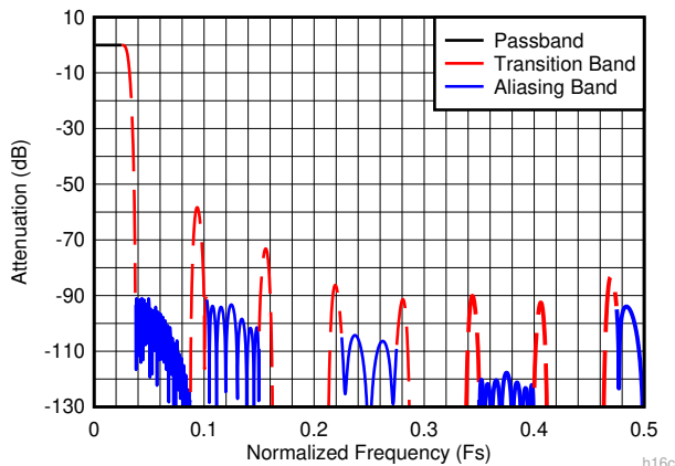
Figure 7-15. Decimate-by-16 Composite Response h16c
