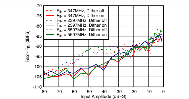
Figure 6-82. Dual Channel Mode: F_s/2 - F_{\text{IN}} vs Input Amplitude and Dither
