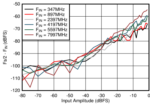
Figure 6-67. DES Mode: F_{s/2} - F_{IN} vs Input Amplitude and Frequency
