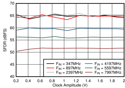
Figure 6-86. Dual Channel Mode: SFDR vs Clock Amplitude
