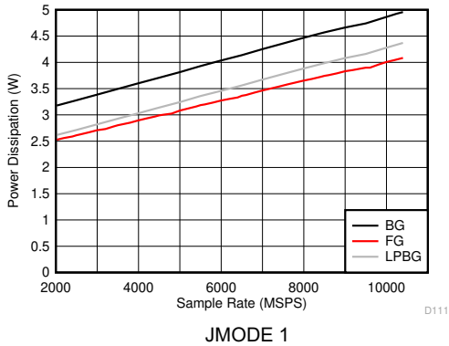
Figure 6-129. DES Mode: Power Dissipation vs Sample Rate
