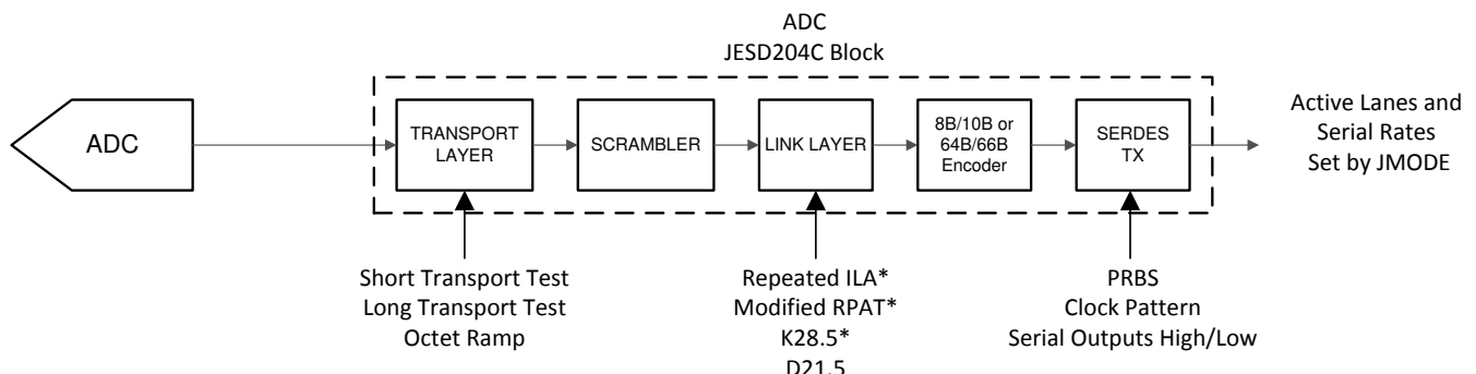
Figure 7-24. Test Mode Insertion Points
