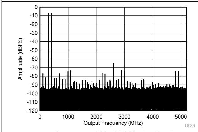
Figure 6-11. DES Mode: Two Tone FFT at 347 MHz
