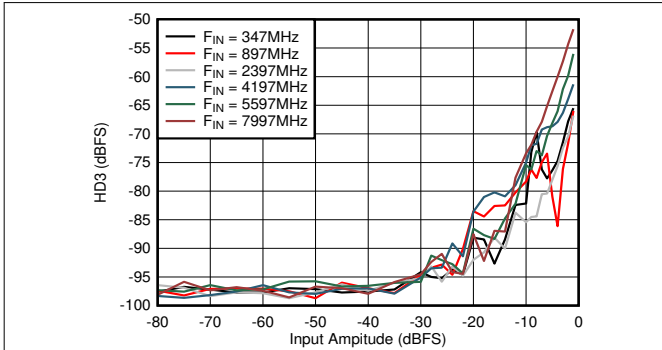
Figure 6-79. Dual Channel Mode: HD3 vs Input Amplitude and Frequency
