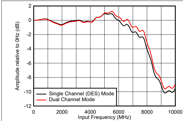
Figure 6-1. Input Amplitude vs Input Frequency
