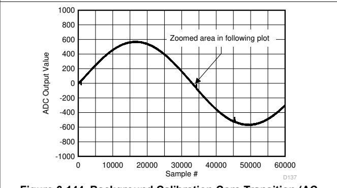
Figure 6-144. Background Calibration Core Transition (AC Signal)
