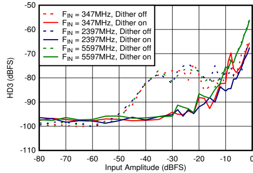
Figure 6-80. Dual Channel Mode: HD3 vs Input Amplitude and Dither
