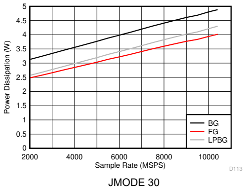
Figure 6-131. DES Mode: Power Dissipation vs Sample Rate
