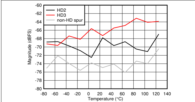
Figure 6-89. DES Mode: HD2, HD3 and Worst non-HD Spur vs Temperature
