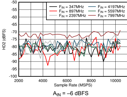
Figure 6-37. DES Mode: HD2 vs Sample Rate and Input Frequency A_{\text{IN}} = -6\text{ dBFS}
