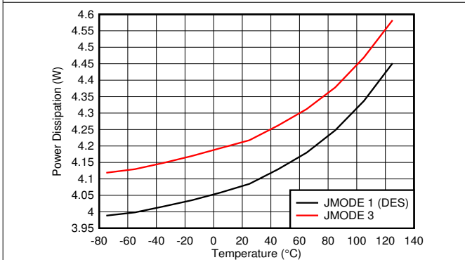
Figure 6-143. Power Dissipation vs Temperature
