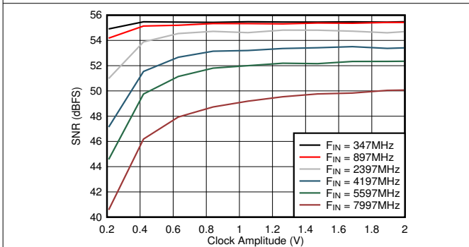
Figure 6-83. DES Mode: SNR vs Clock Amplitude
