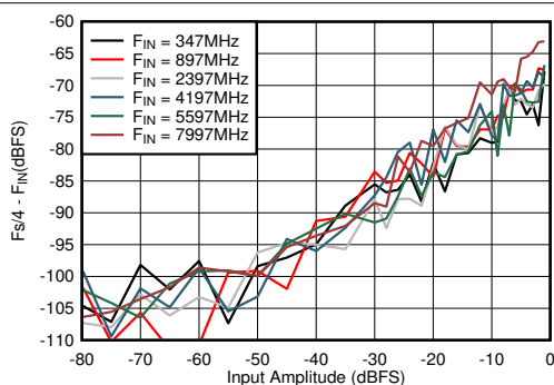
Figure 6-71. DES Mode: F_{s/4} - F_{IN} vs Input Amplitude and Frequency
