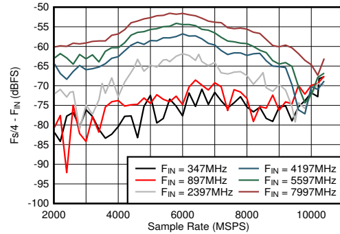
Figure 6-44. DES Mode: F_s/4 - F_{IN} vs Sample Rate and Input Frequency
