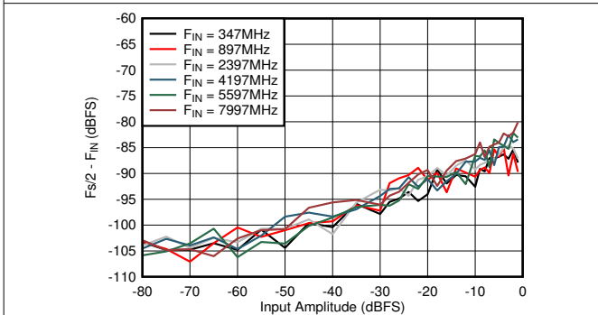
Figure 6-81. Dual Channel Mode: F_s/2 - F_{\text{IN}} vs Input Amplitude and Frequency
