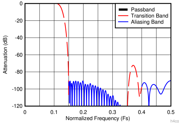
Figure 7-11. Decimate-by-4 Composite Response h4co
