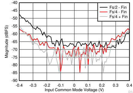
Figure 6-100. F_s/2 - F_{IN} and F_s/4 \pm F_{IN} vs Input Common Mode Voltage
