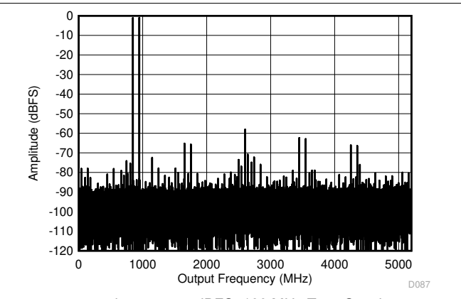
Figure 6-12. DES Mode: Two Tone FFT at 897 MHz
