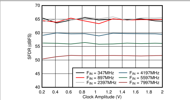
Figure 6-86. Dual Channel Mode: SFDR vs Clock Amplitude
