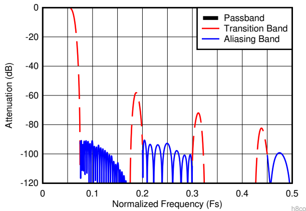
Figure 7-13. Decimate-by-8 Composite Response h8co
