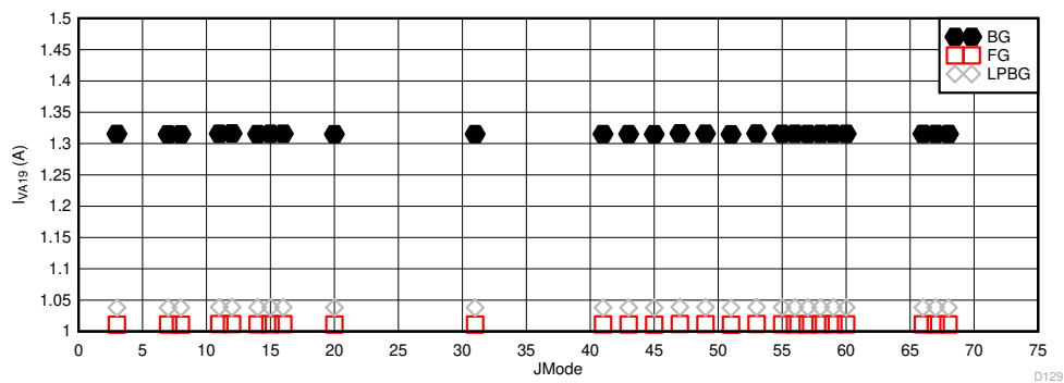
Figure 6-114. DES Mode: Power Dissipation vs JMODE at 10.4GSPS
