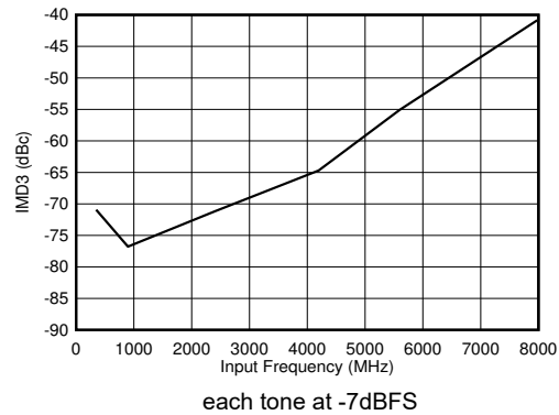
Figure 6-106. Dual Channel Mode: IMD3 vs Input Frequency
