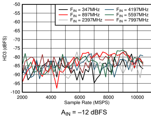
Figure 6-41. DES Mode: HD3 vs Sample Rate and Input Frequency A_{\text{IN}} = -12\text{ dBFS}
