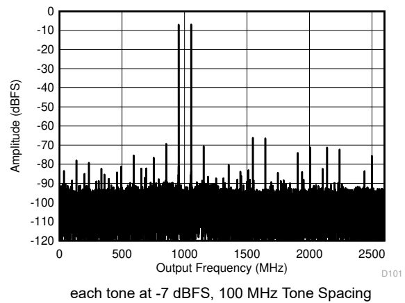
each tone at -7 dBFS, 100 MHz Tone Spacing Figure 6-26. Dual Channel Mode: Two Tone FFT at 4197 MHz
