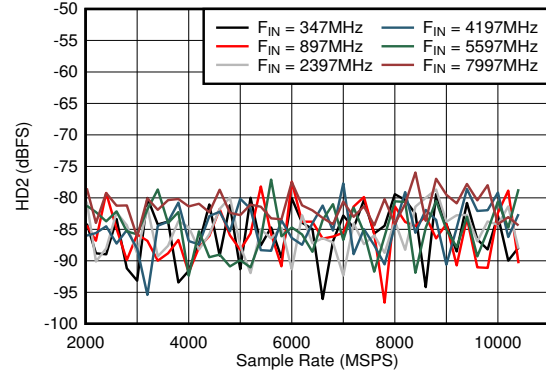
Figure 6-38. DES Mode: HD2 vs Sample Rate and Input Frequency A_{\text{IN}} = -12\text{ dBFS}
