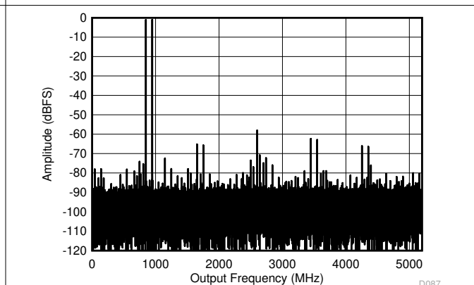
Figure 6-12. DES Mode: Two Tone FFT at 897 MHz
