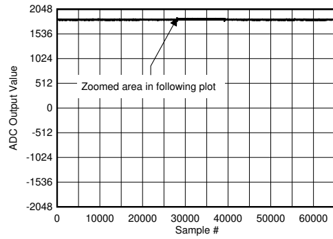
Figure 6-146. Background Calibration Core Transition (DC Signal)
