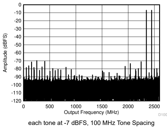
each tone at -7 dBFS, 100 MHz Tone Spacing Figure 6-25. Dual Channel Mode: Two Tone FFT at 2397 MHz
