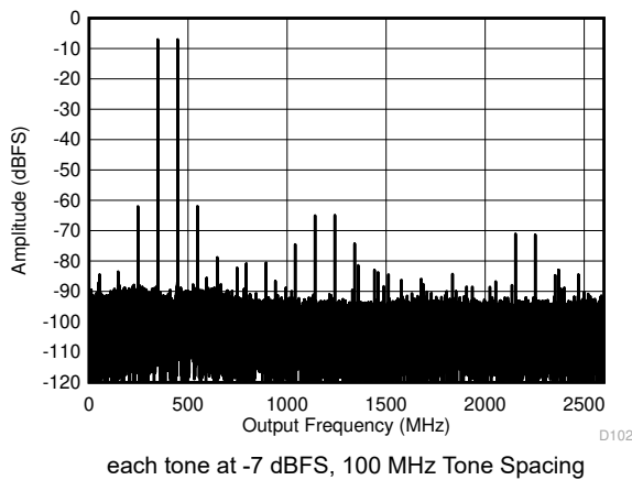
each tone at -7 dBFS, 100 MHz Tone Spacing Figure 6-27. Dual Channel Mode: Two Tone FFT at 5597 MHz
