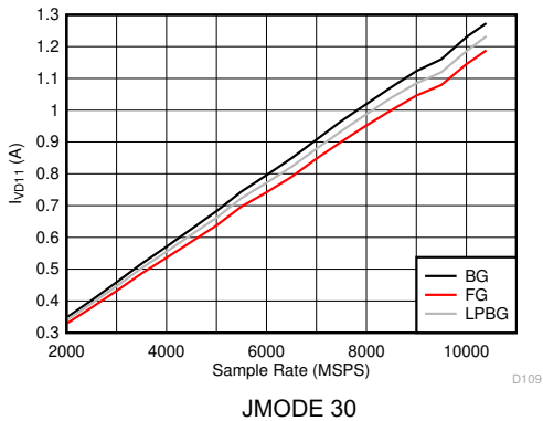
Figure 6-127. DES Mode: I_{VD11} vs Sample Rate
